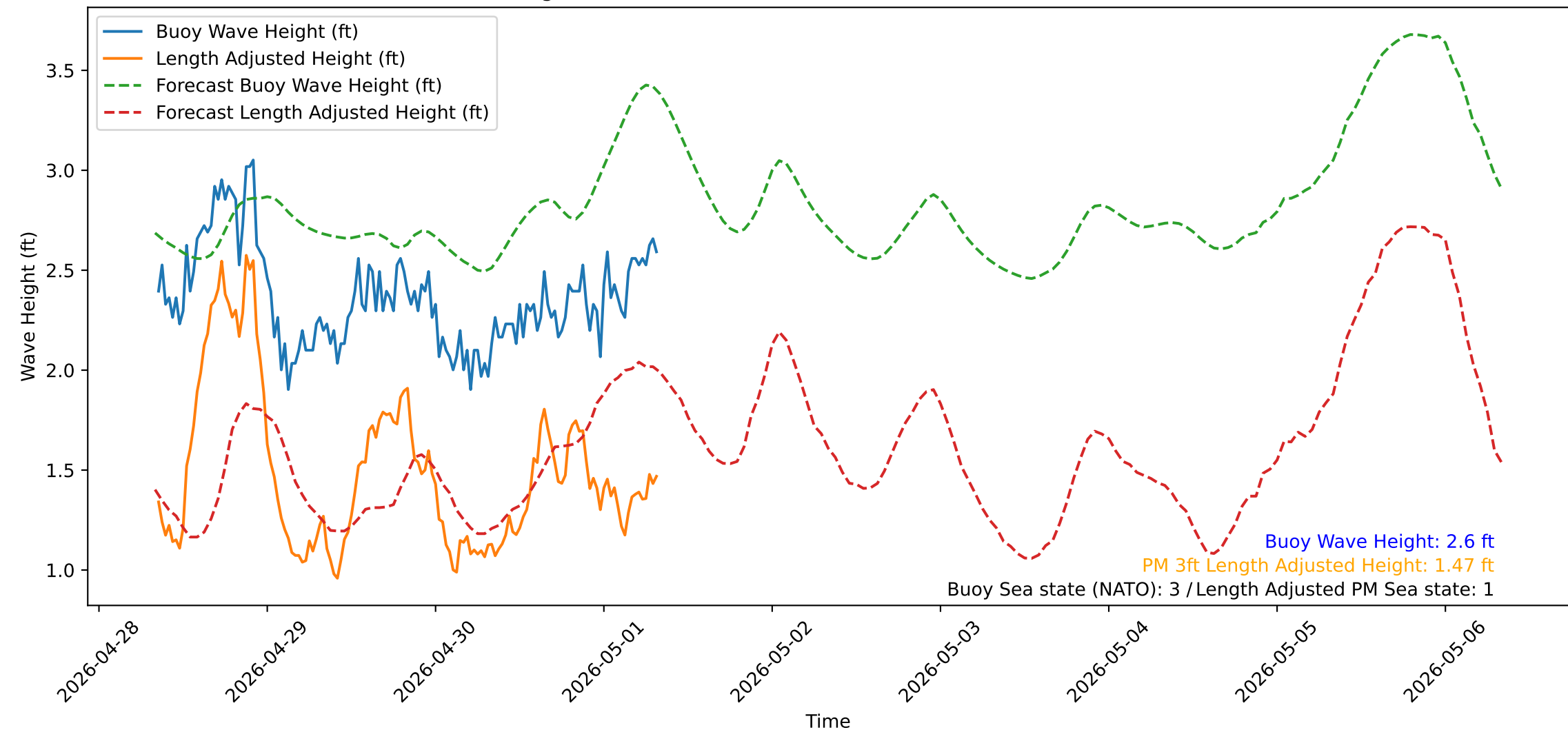
Wave Heights over Time for Oceanside Harbor at 2026-05-01 08:20:31
