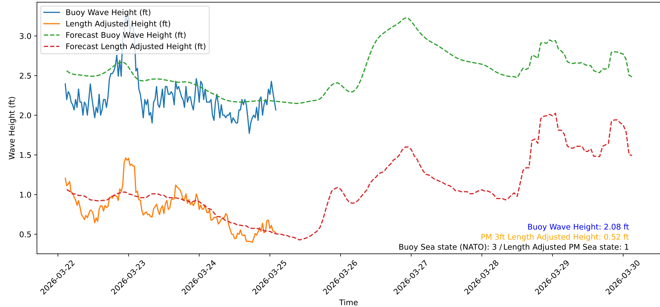
Wave Heights over Time for Green Beach at 2026-03-25 02:41:10
