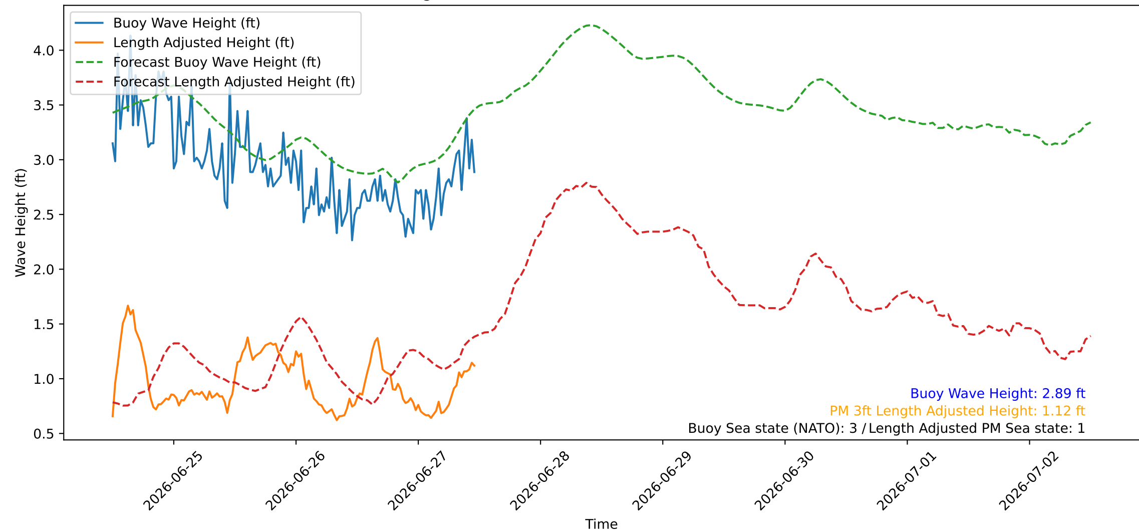
Wave Heights over Time for Red Beach at 2026-06-27 11:40:46
