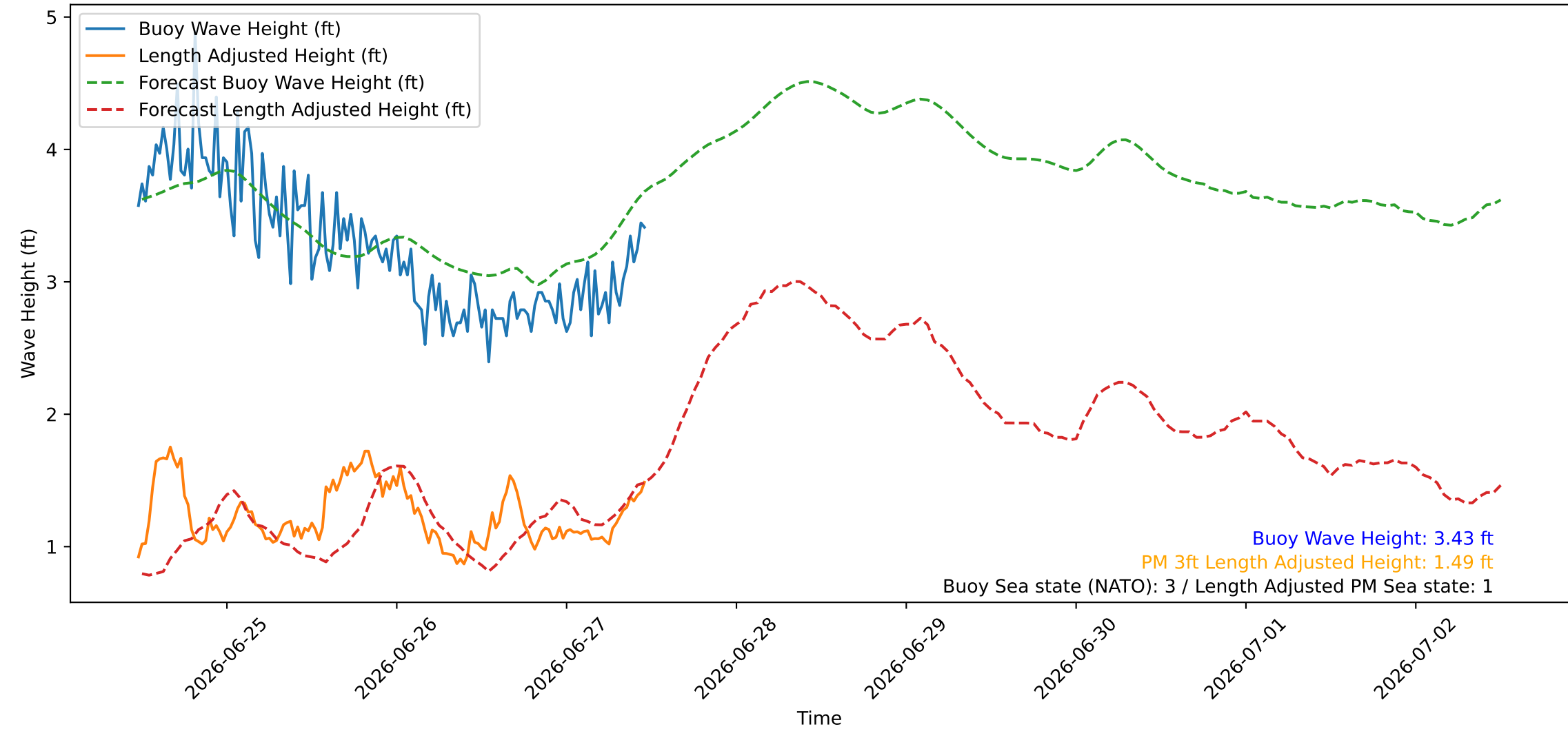
Wave Heights over Time for Oceanside Harbor at 2026-06-27 11:40:26
