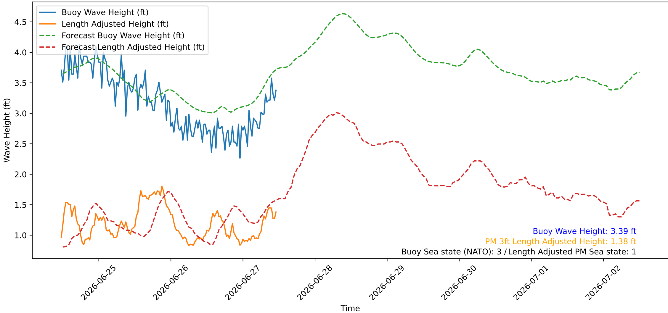
Wave Heights over Time for Green Beach at 2026-06-27 11:41:09
