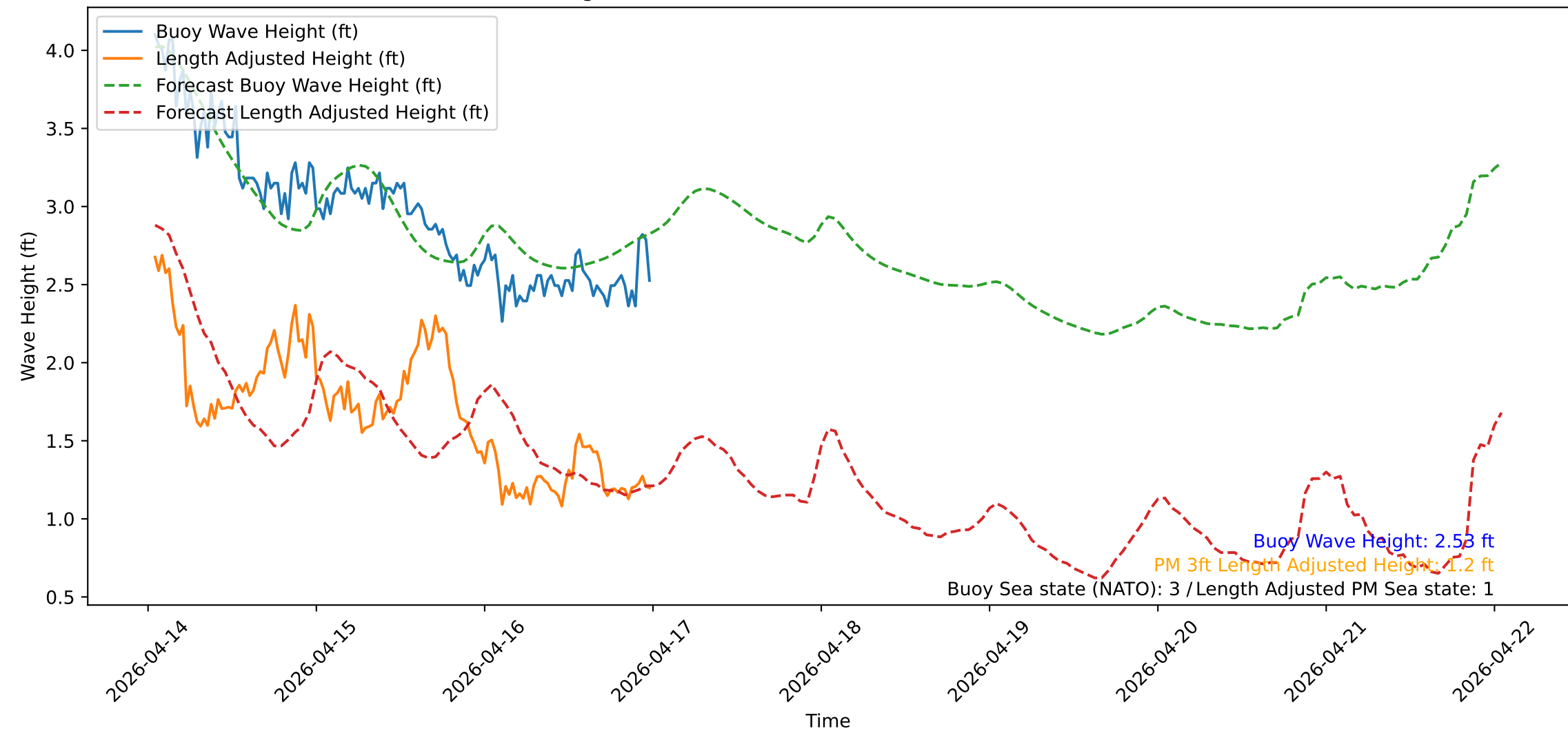
Wave Heights over Time for Red Beach at 2026-04-17 00:30:51
