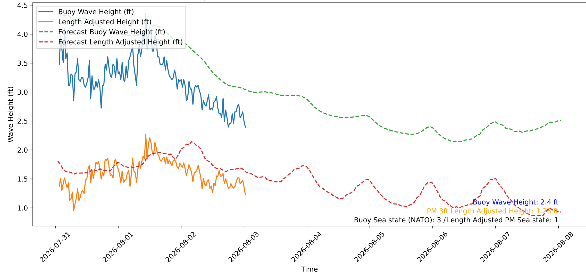
Wave Heights over Time for Oceanside Harbor at 2026-08-03 01:20:26
