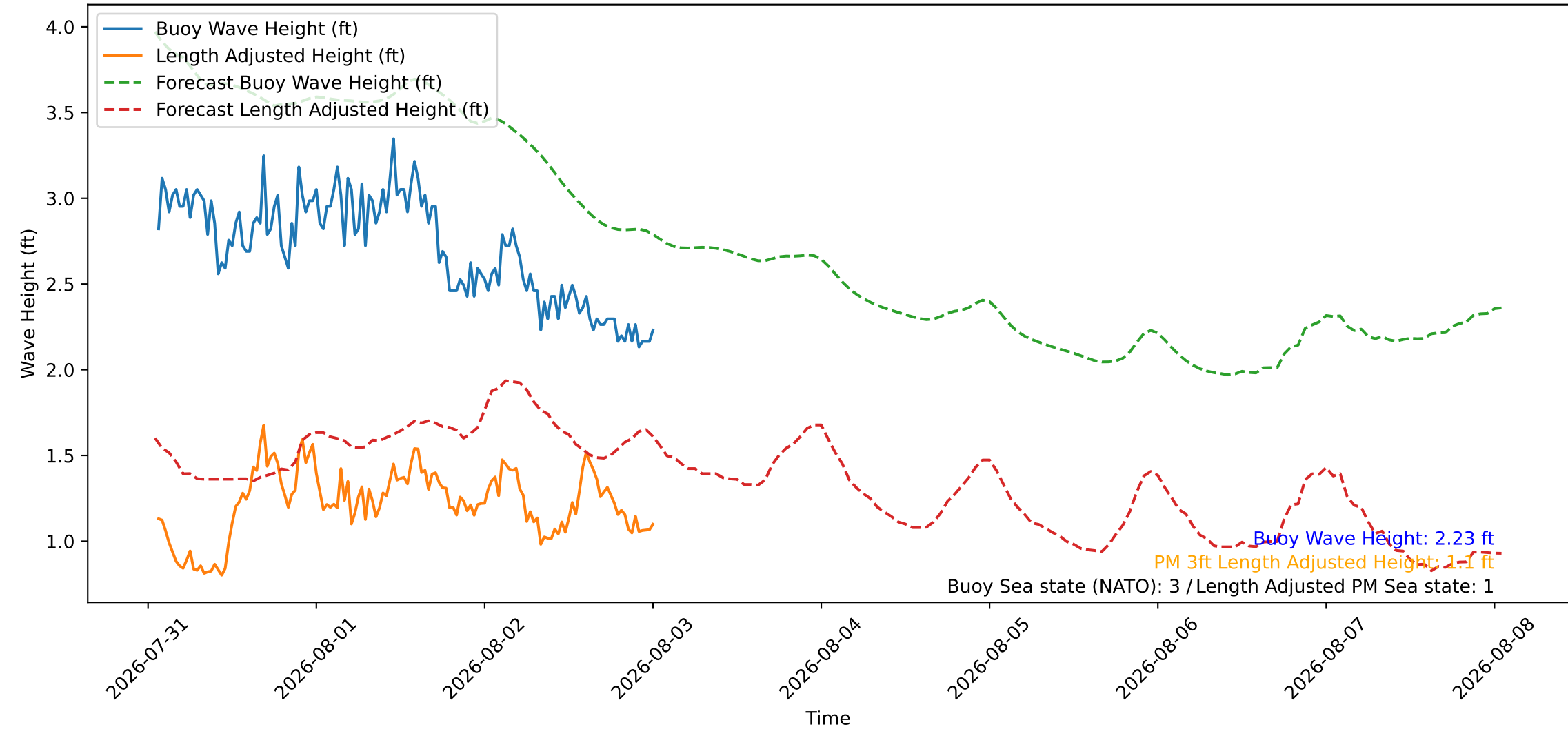
Wave Heights over Time for Red Beach at 2026-08-03 01:20:47
