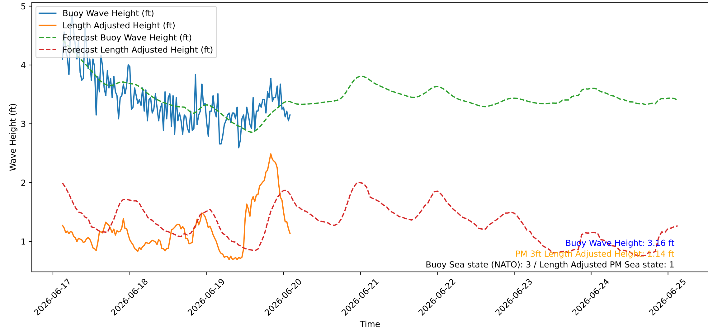
Wave Heights over Time for Red Beach at 2026-06-20 02:50:46
