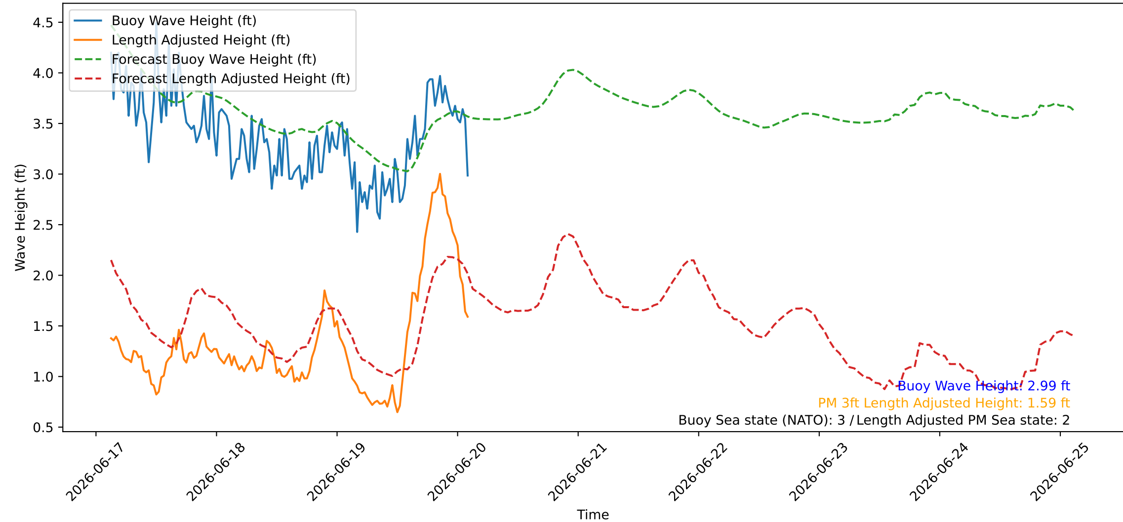
Wave Heights over Time for Green Beach at 2026-06-20 02:51:08
