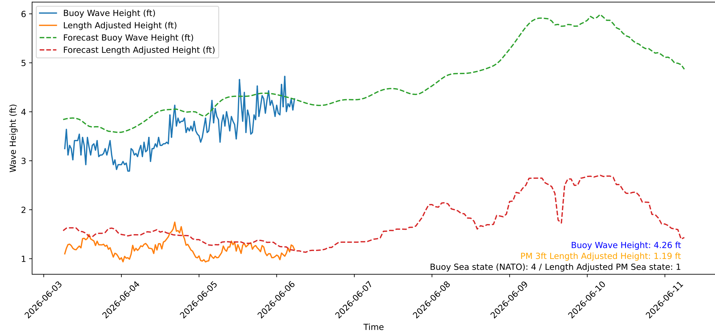
Wave Heights over Time for Green Beach at 2026-06-06 06:21:08
