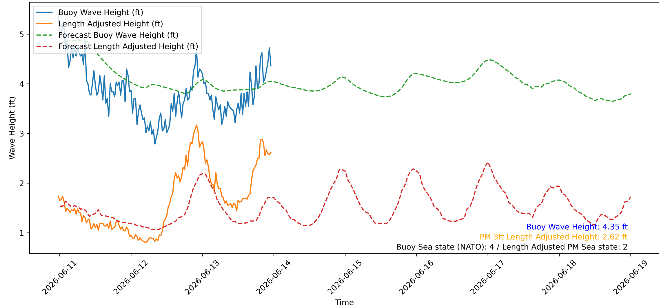
Wave Heights over Time for Oceanside Harbor at 2026-06-13 23:30:26
