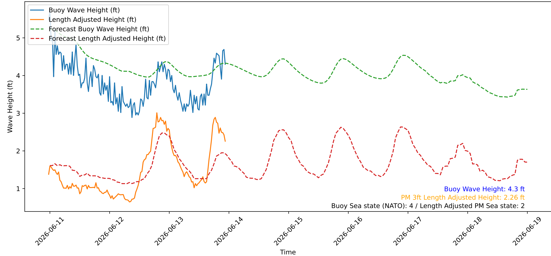
Wave Heights over Time for Green Beach at 2026-06-13 23:31:07
