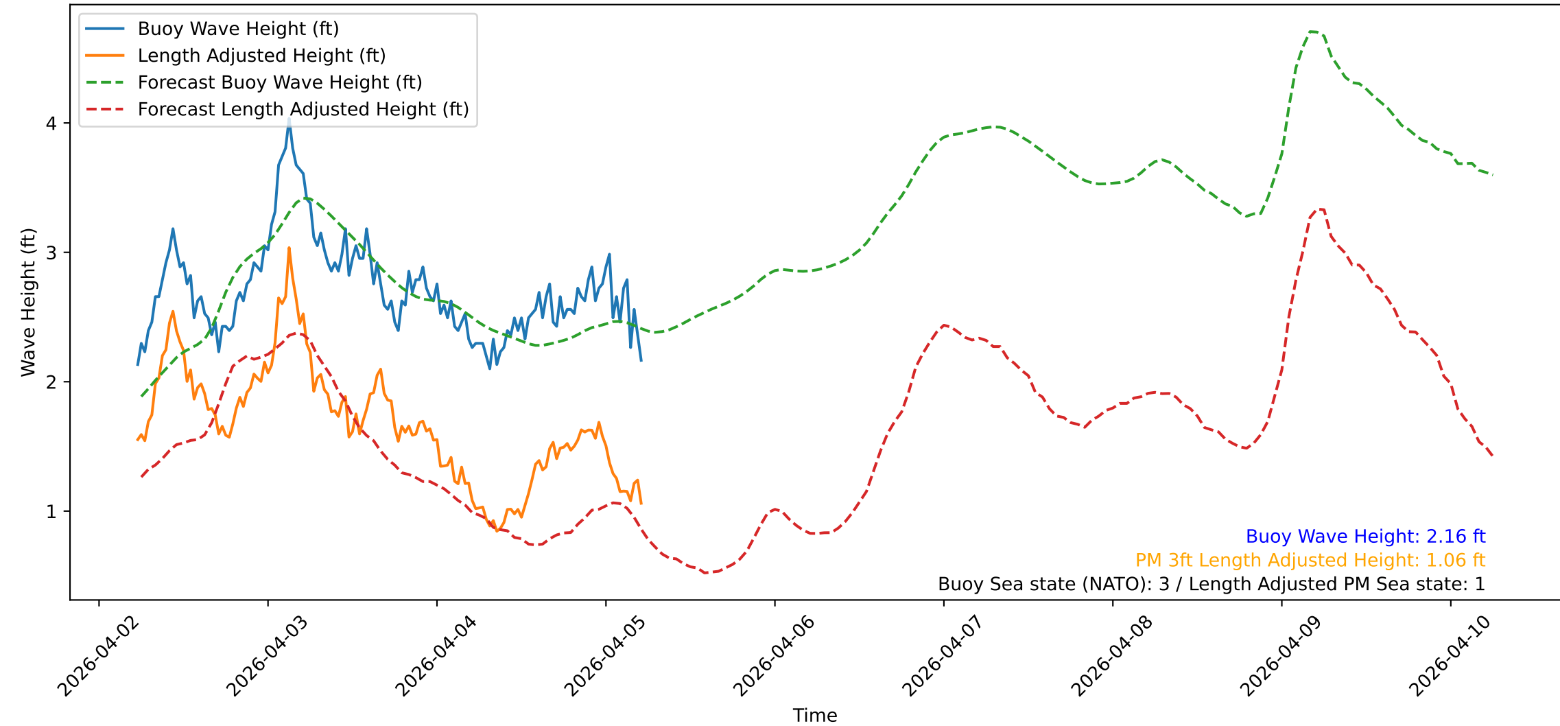
Wave Heights over Time for Oceanside Harbor at 2026-04-05 05:40:31
