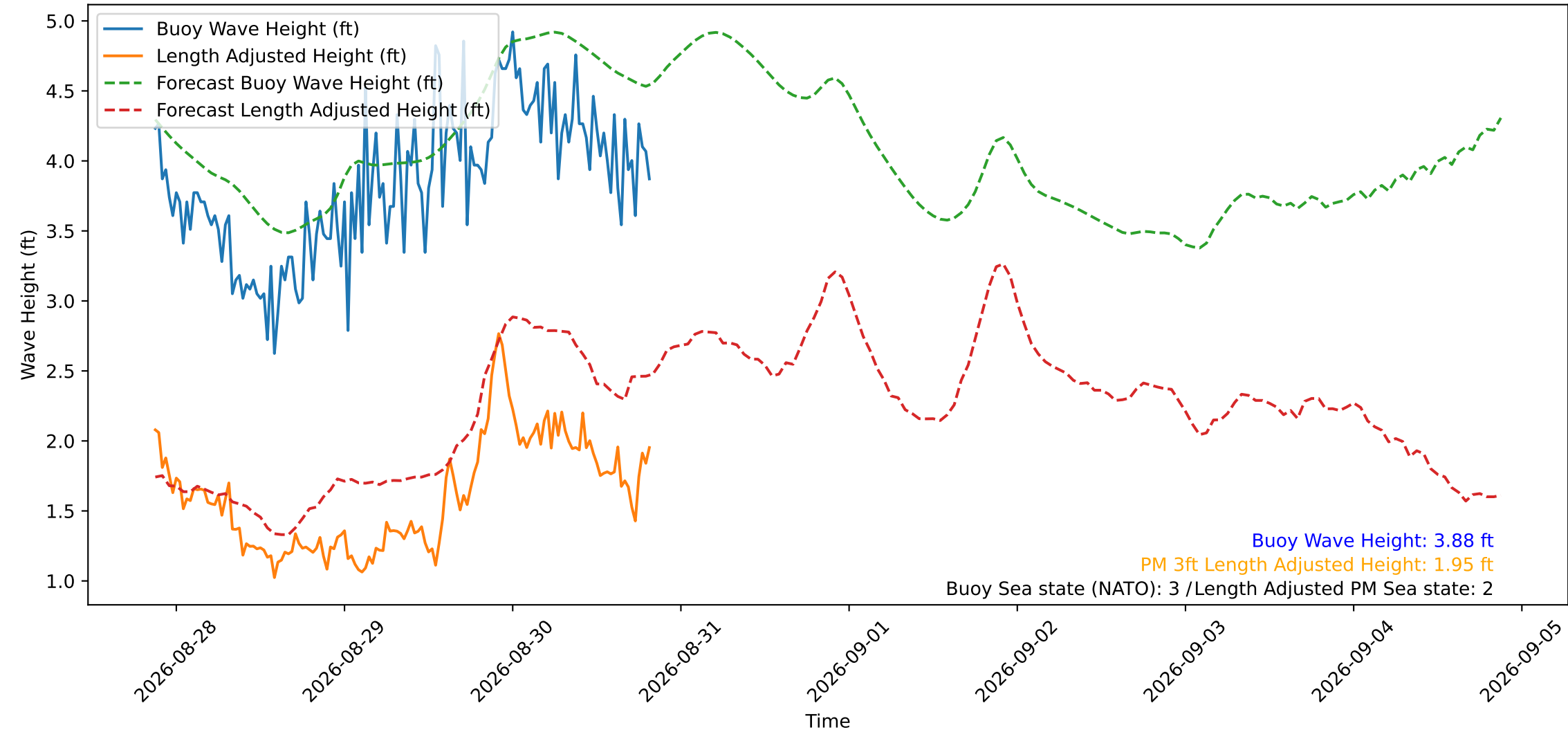
Wave Heights over Time for Green Beach at 2026-08-30 20:31:11
