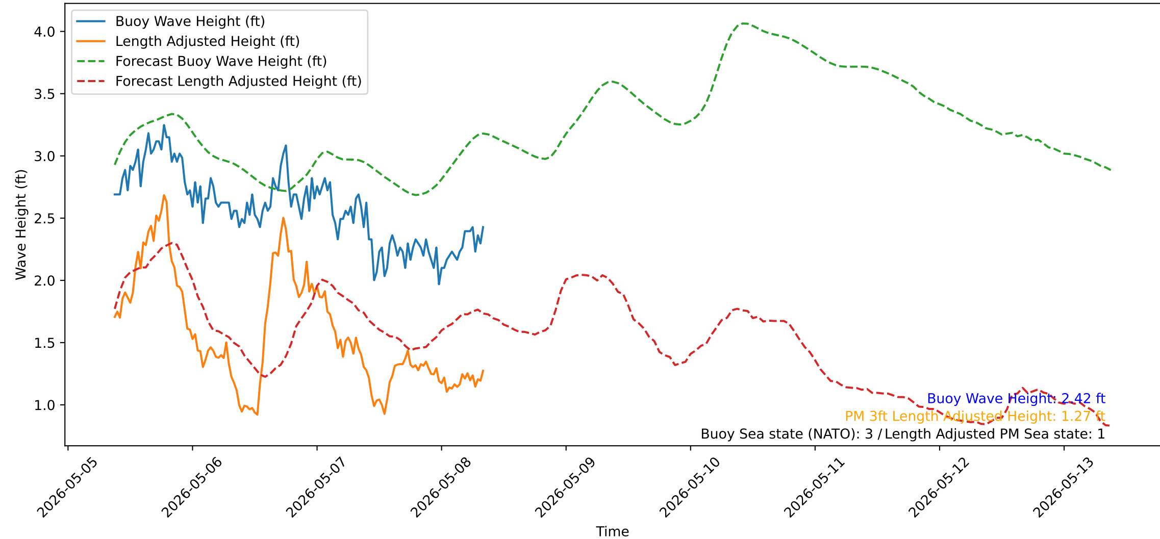
Wave Heights over Time for Oceanside Harbor at 2026-05-08 08:50:31
