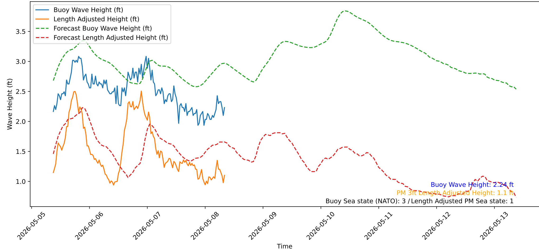
Wave Heights over Time for Red Beach at 2026-05-08 08:50:52
