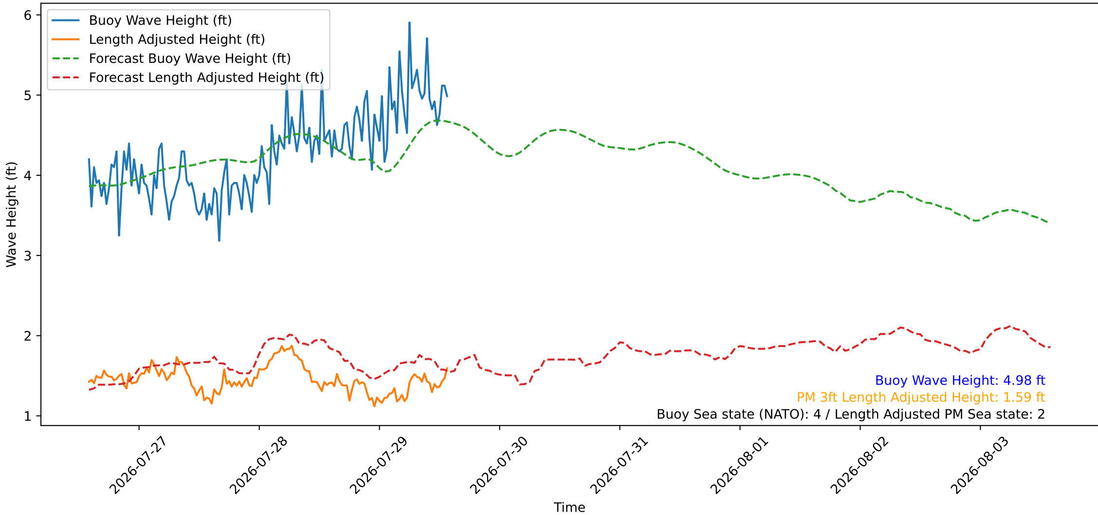
Wave Heights over Time for Oceanside Harbor at 2026-07-29 14:10:26
