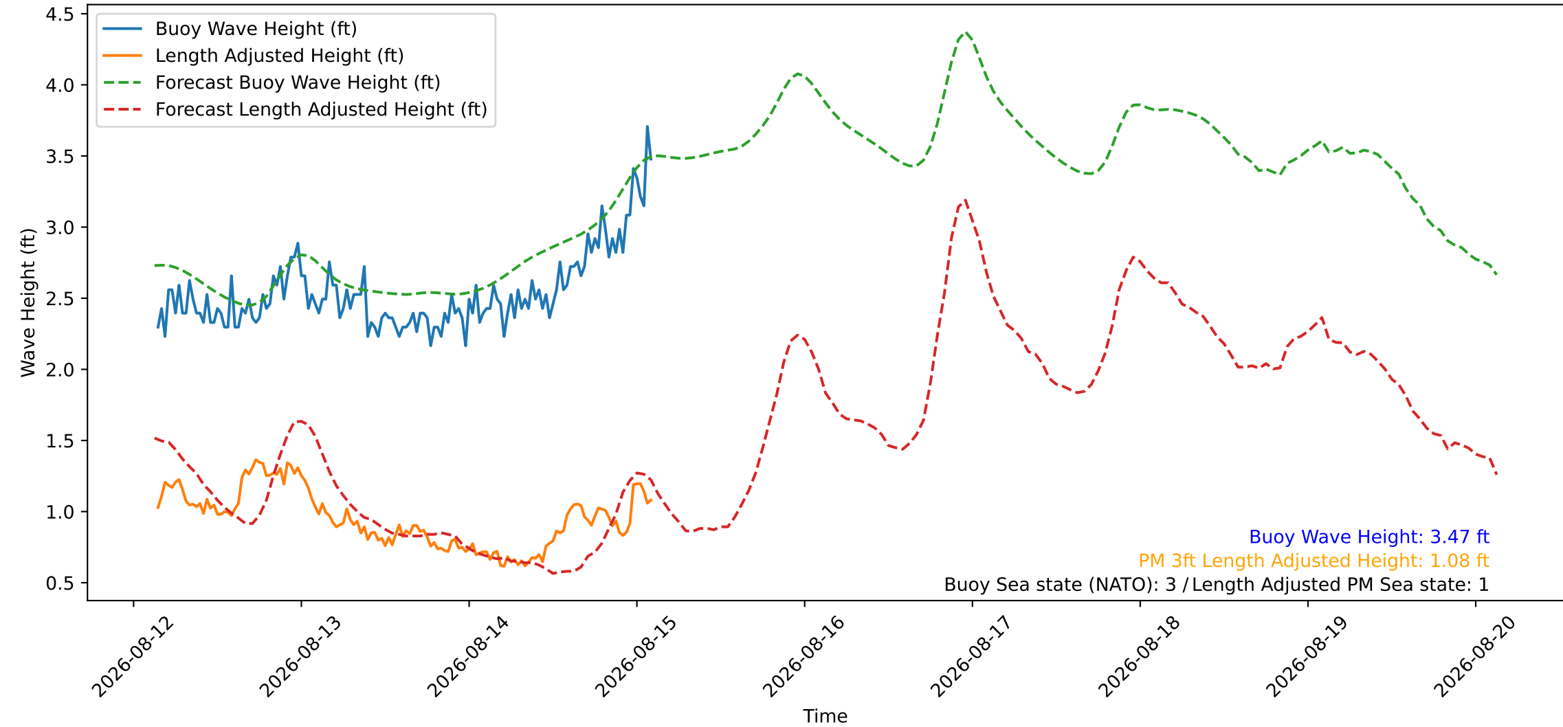
Wave Heights over Time for Red Beach at 2026-08-15 03:00:46
