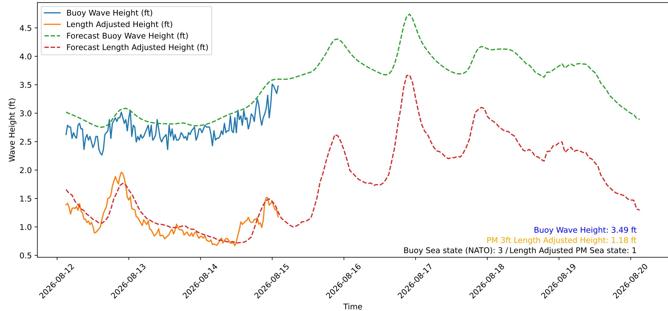
Wave Heights over Time for Green Beach at 2026-08-15 03:01:08
