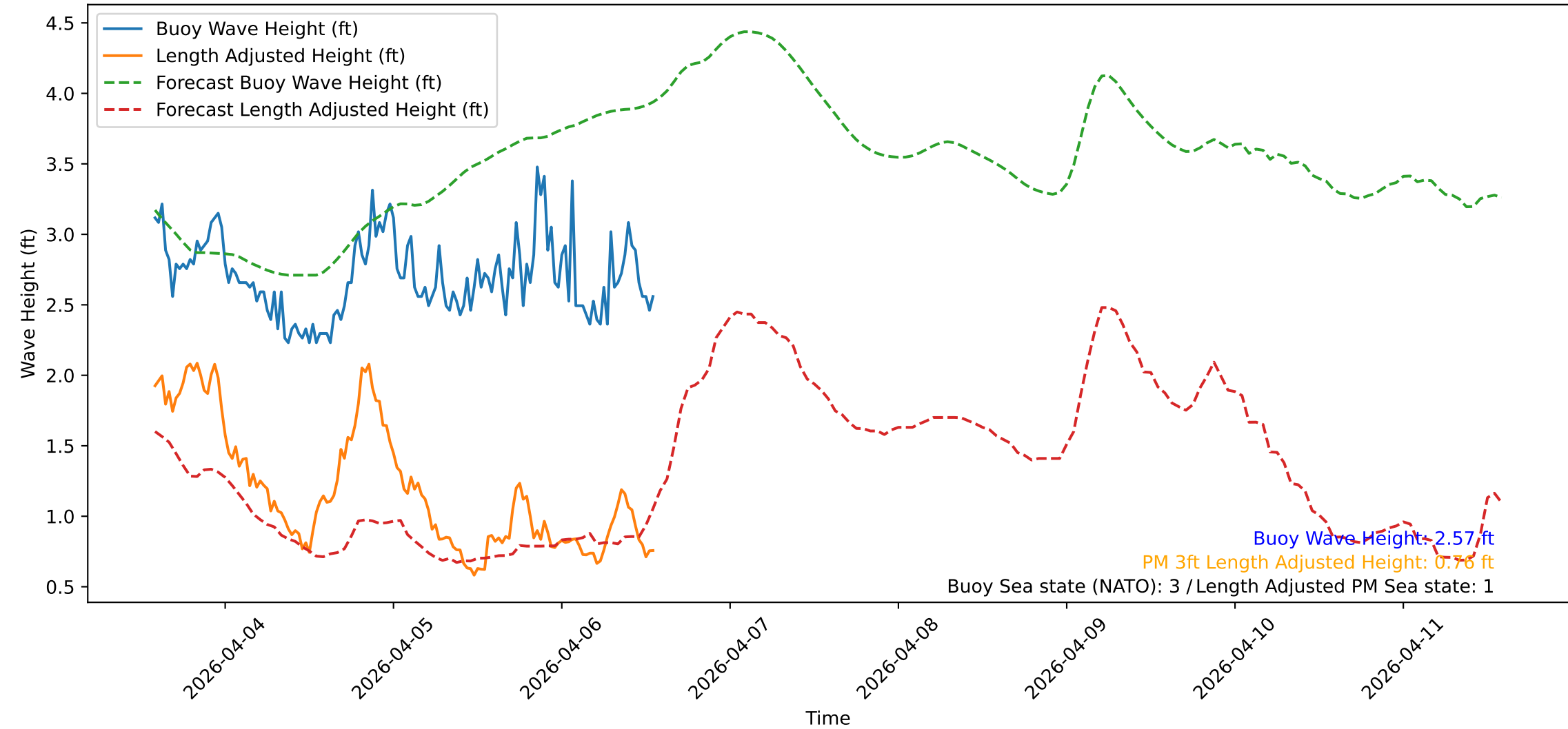
Wave Heights over Time for Green Beach at 2026-04-06 13:51:09
