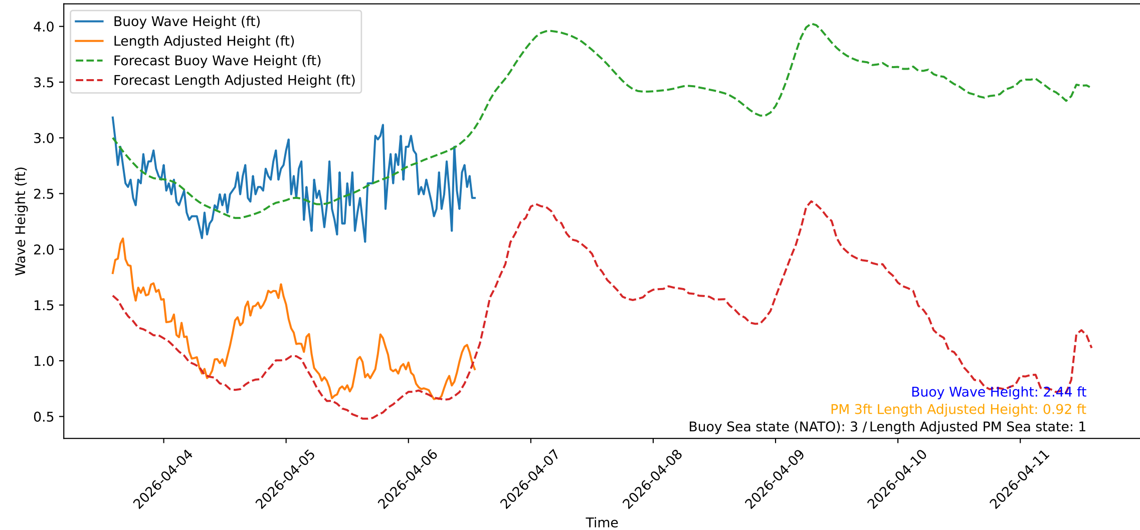
Wave Heights over Time for Oceanside Harbor at 2026-04-06 13:50:31
