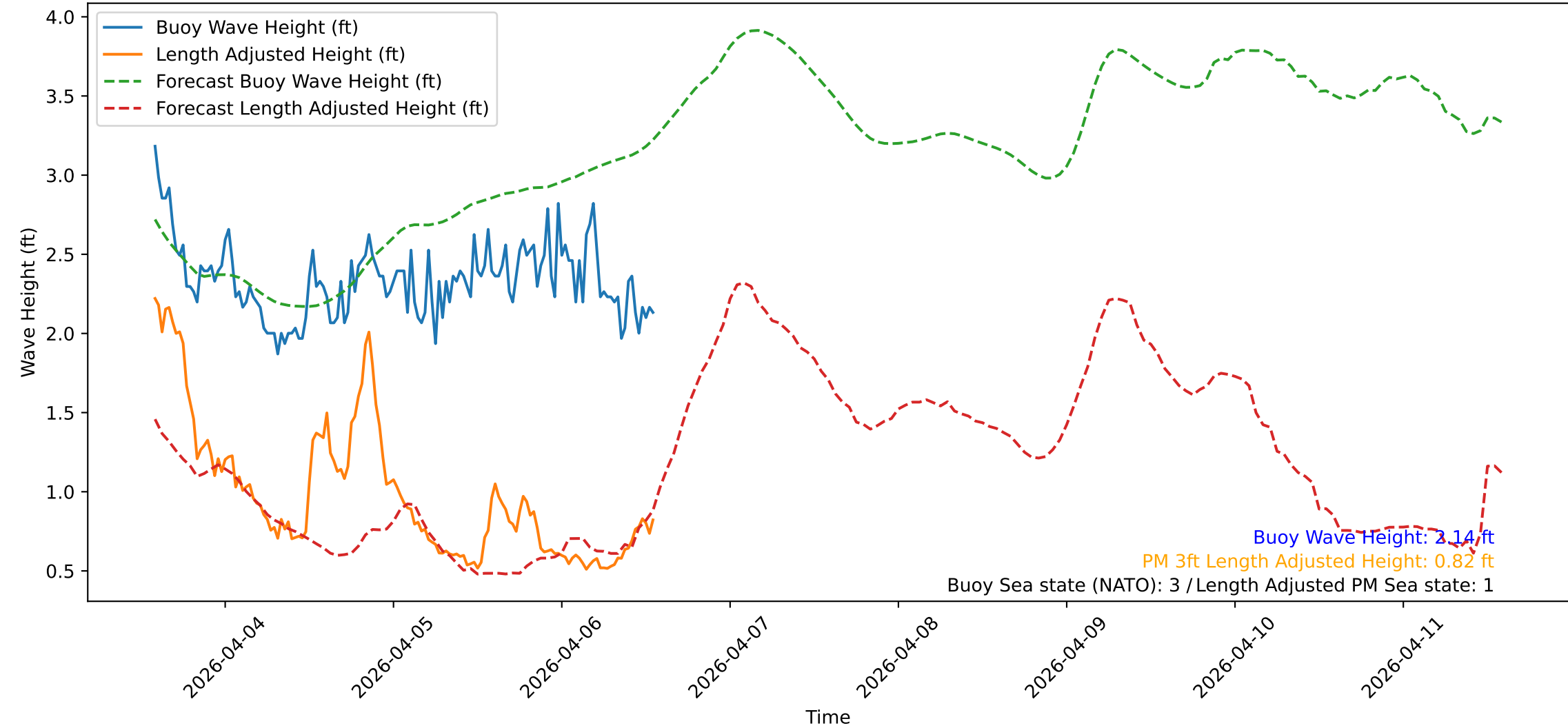
Wave Heights over Time for Red Beach at 2026-04-06 13:50:47
