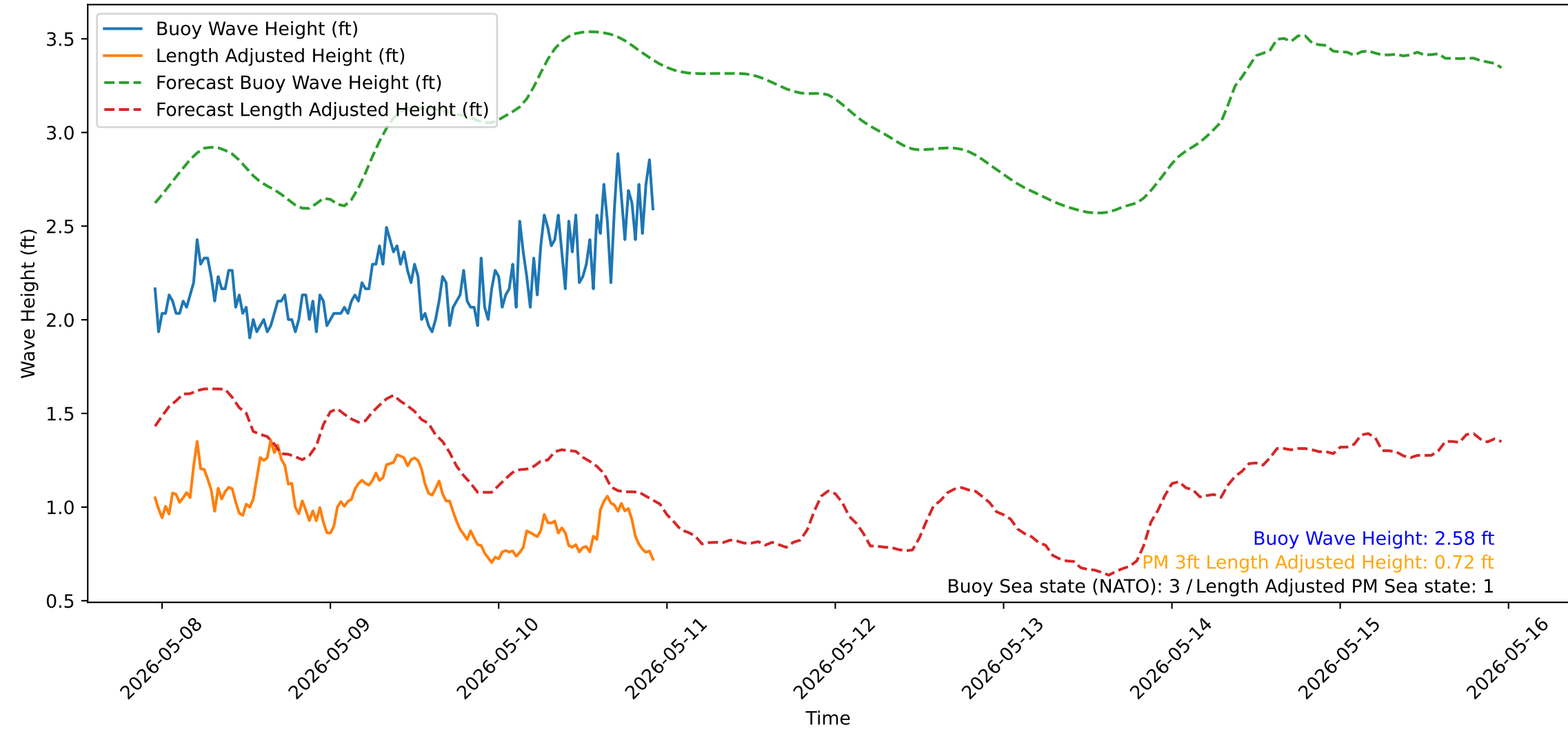
Wave Heights over Time for Red Beach at 2026-05-10 22:40:50
