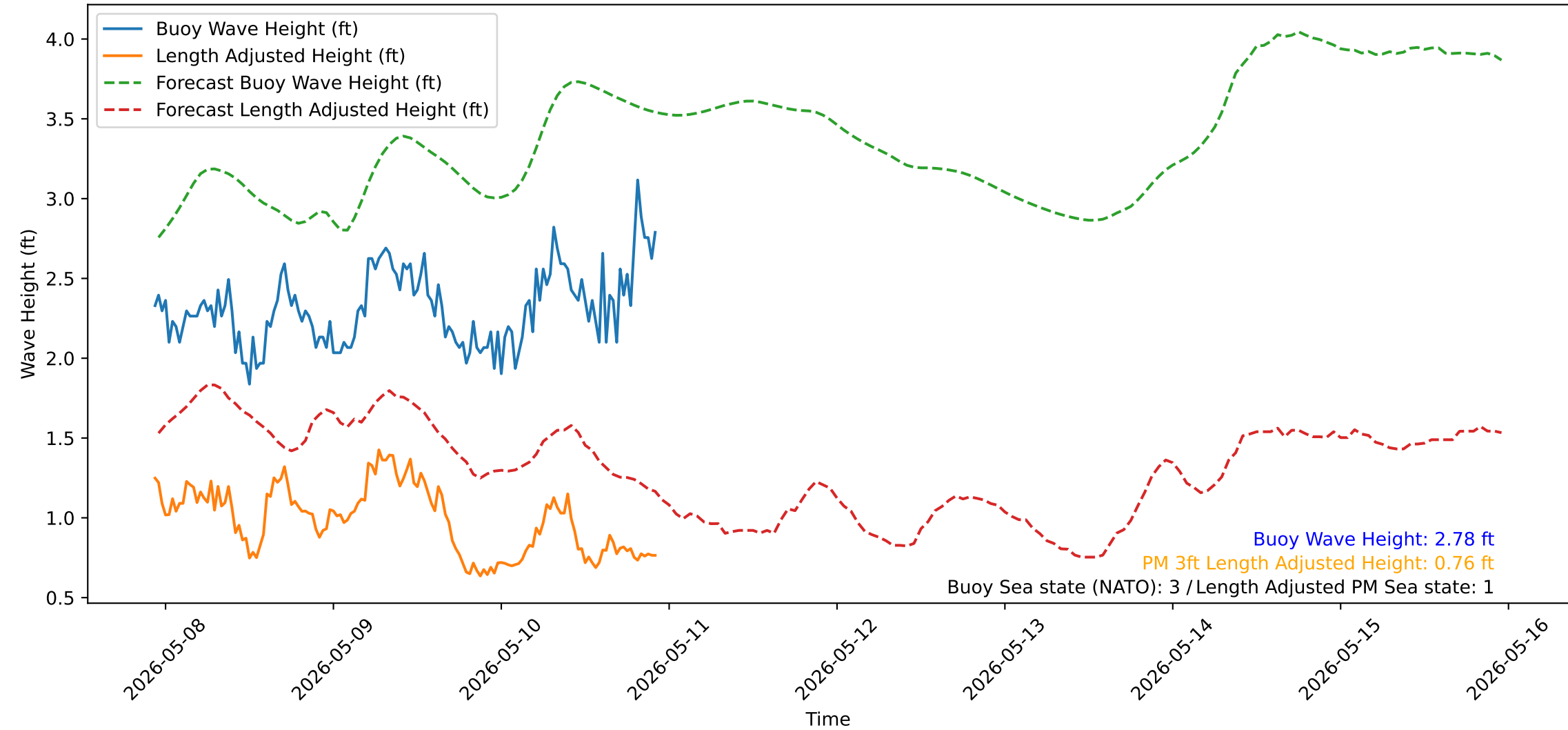
Wave Heights over Time for Green Beach at 2026-05-10 22:41:13
