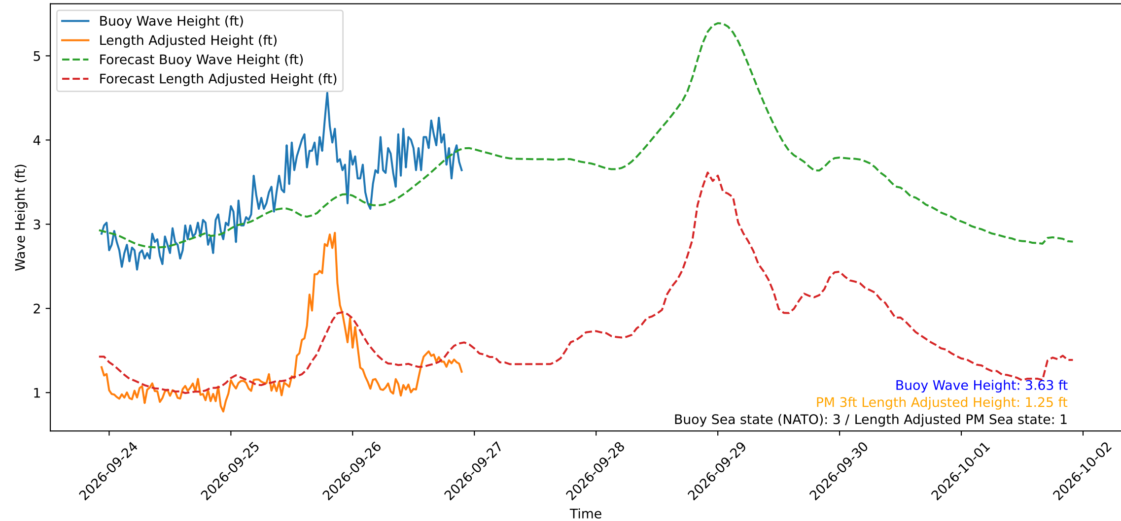
Wave Heights over Time for Green Beach at 2026-09-26 22:11:12
