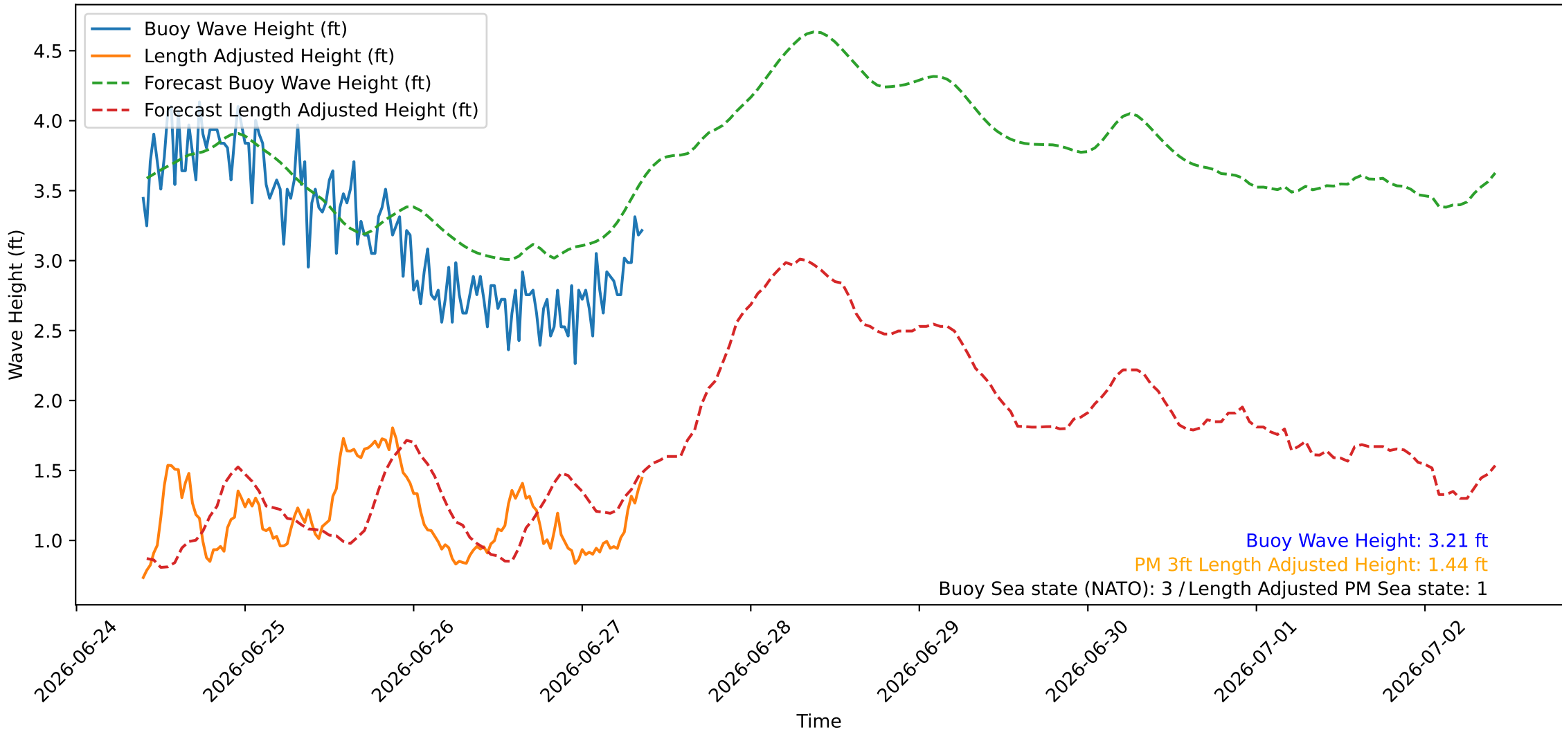
Wave Heights over Time for Green Beach at 2026-06-27 09:31:08
