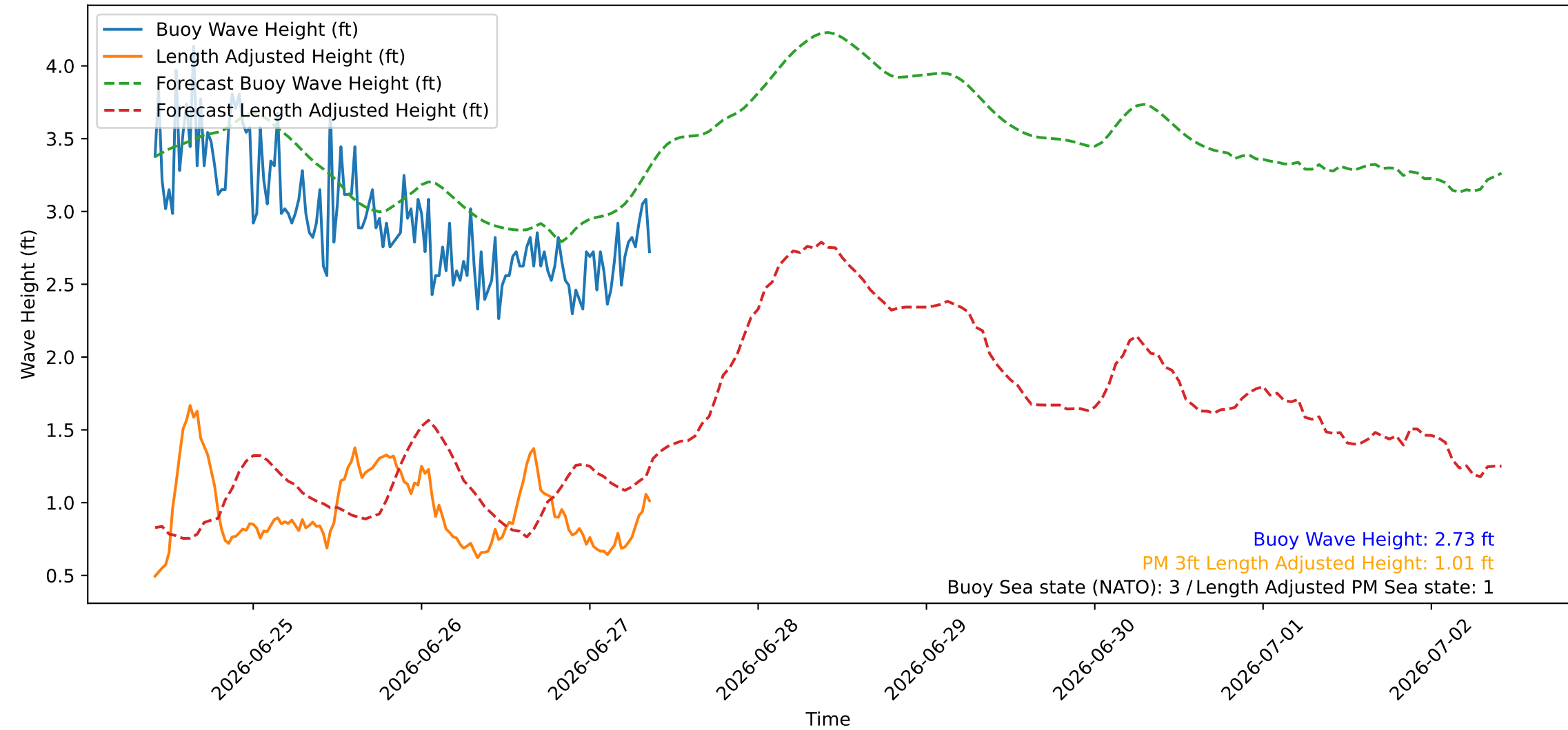
Wave Heights over Time for Red Beach at 2026-06-27 09:30:46
