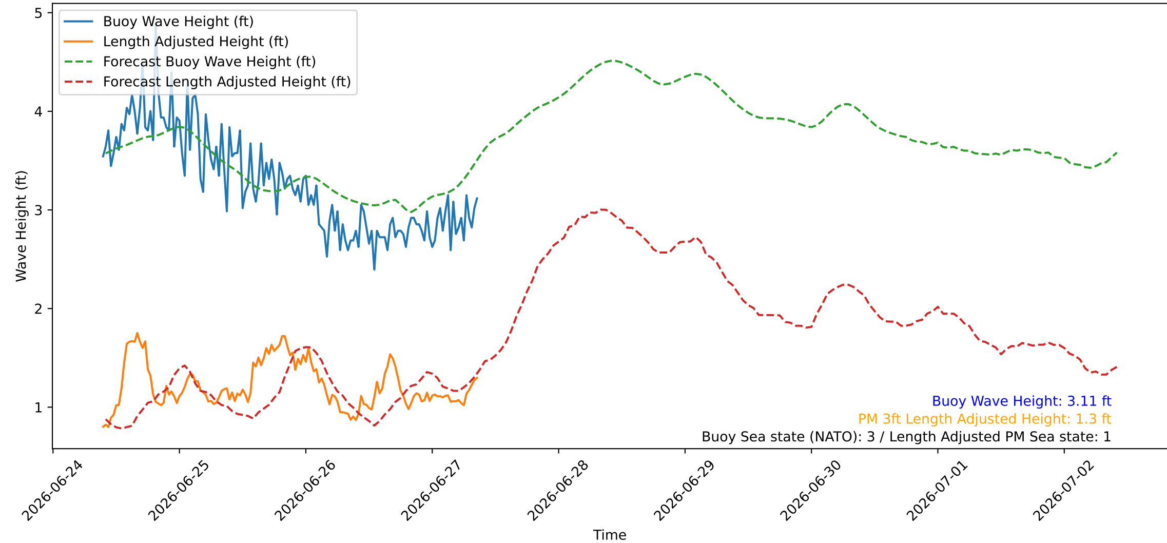
Wave Heights over Time for Oceanside Harbor at 2026-06-27 09:30:27
