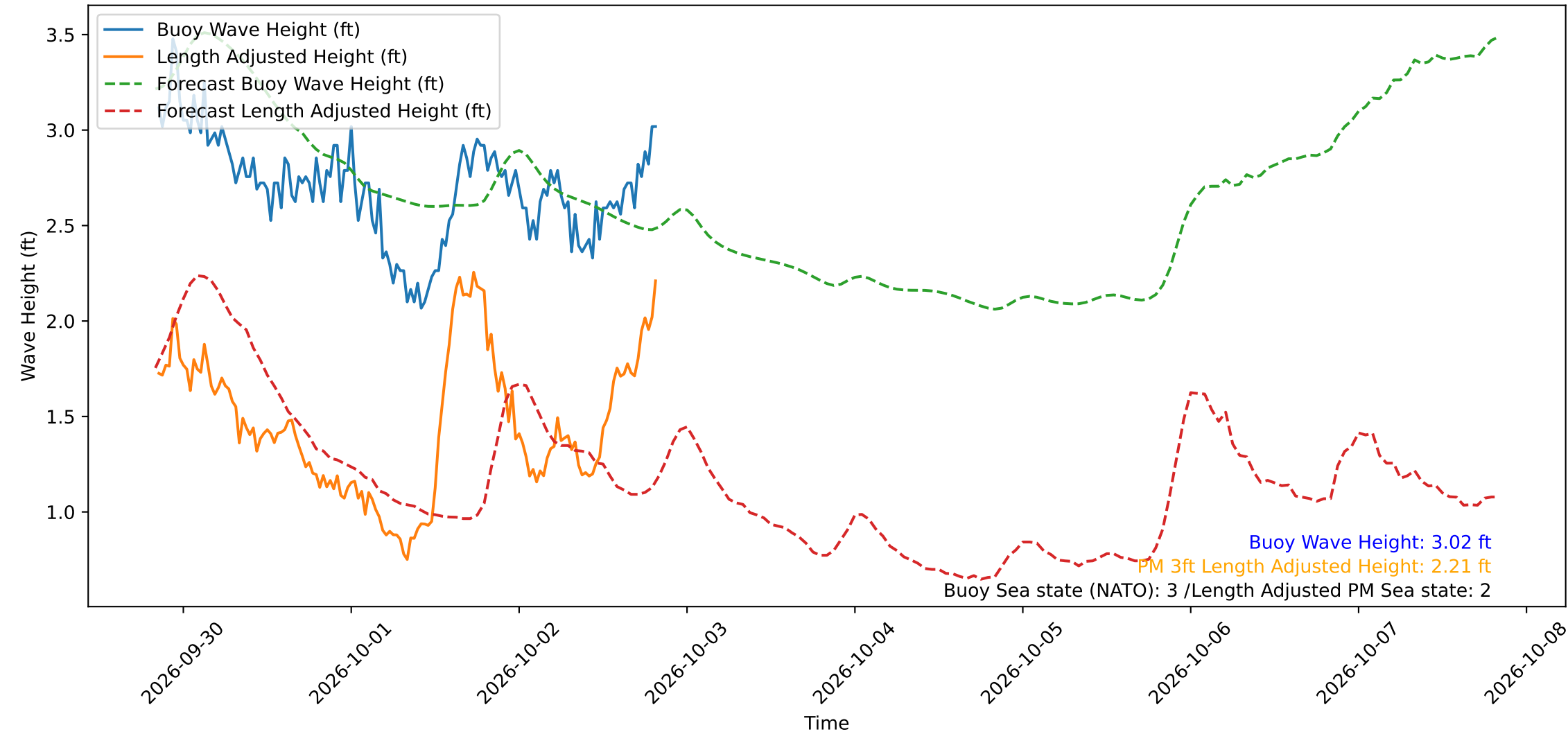
Wave Heights over Time for Red Beach at 2026-10-02 20:10:51
