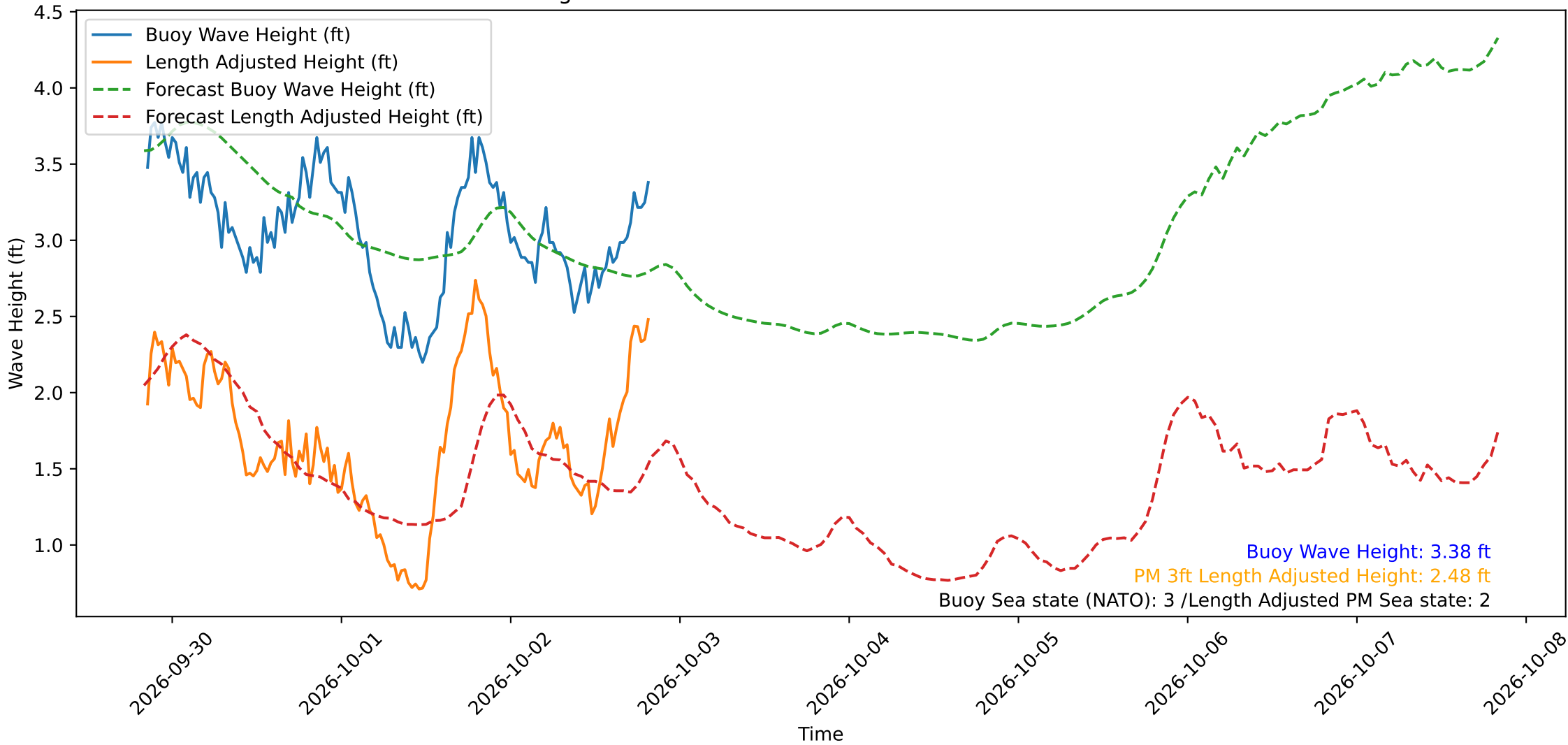
Wave Heights over Time for Green Beach at 2026-10-02 20:11:14
