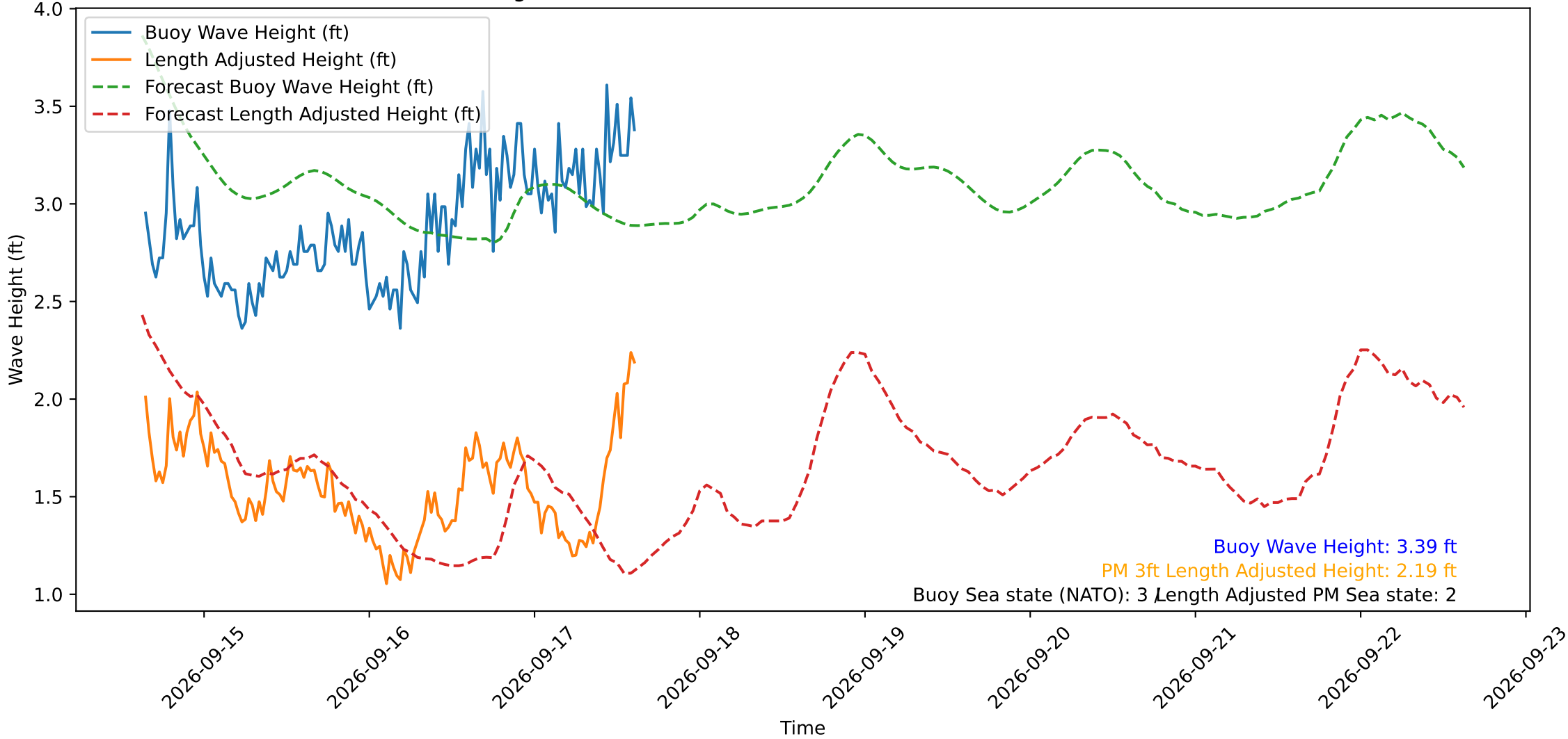
Wave Heights over Time for Oceanside Harbor at 2026-09-17 15:20:29
