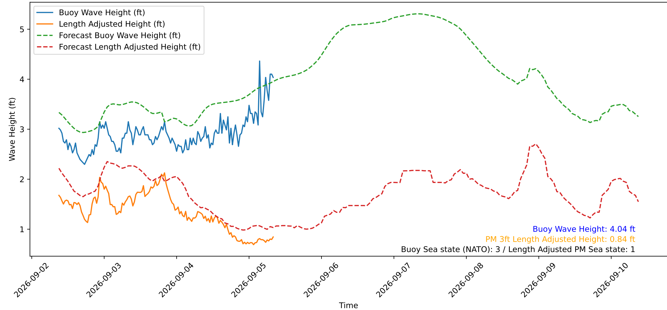
Wave Heights over Time for Red Beach at 2026-09-05 08:40:49
