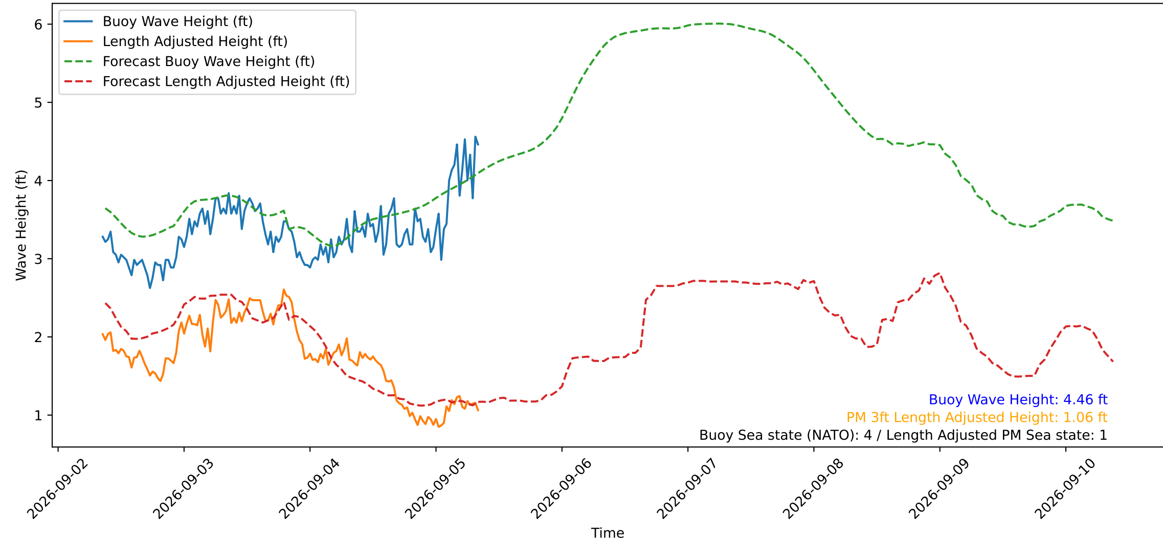
Wave Heights over Time for Oceanside Harbor at 2026-09-05 08:40:29
