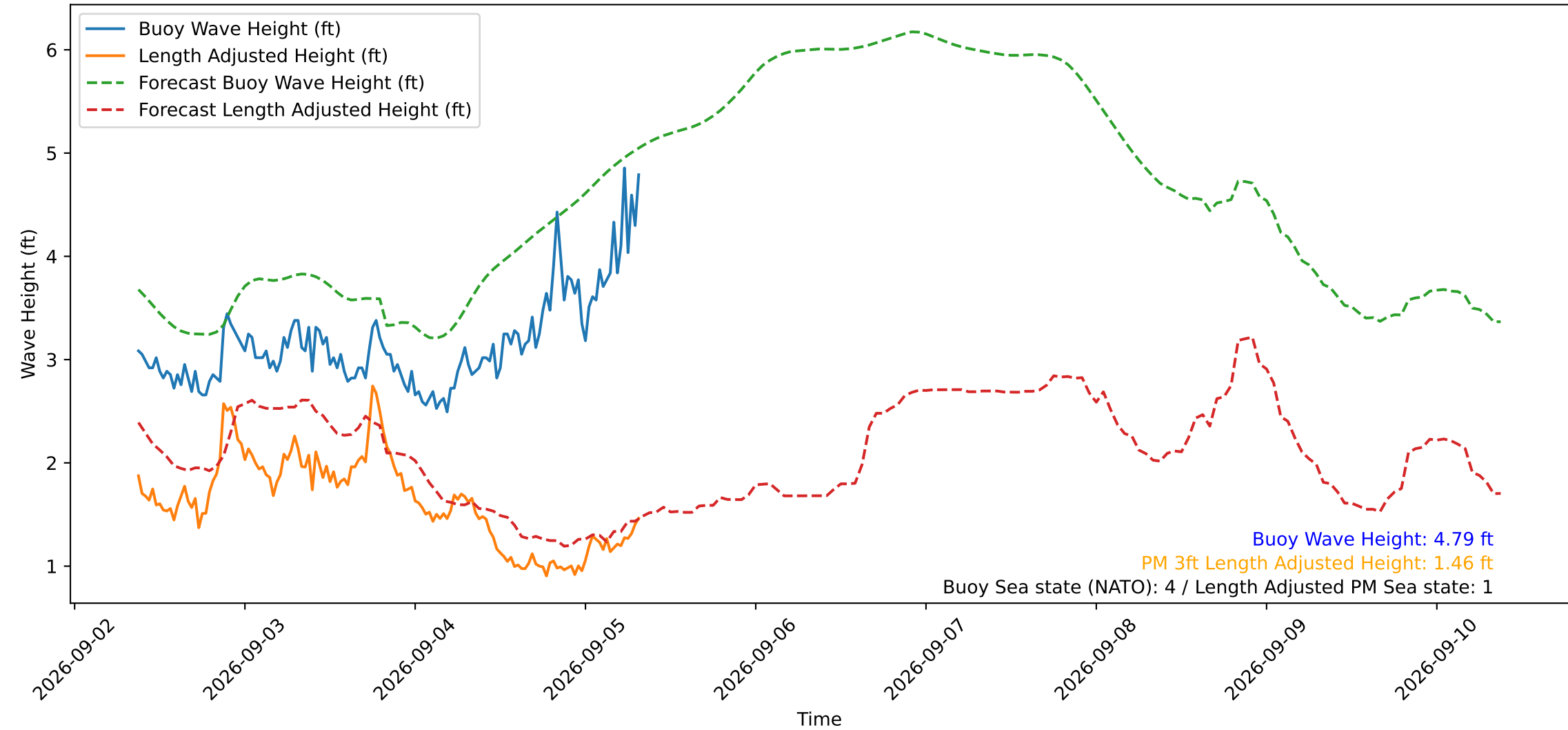
Wave Heights over Time for Green Beach at 2026-09-05 08:41:11
