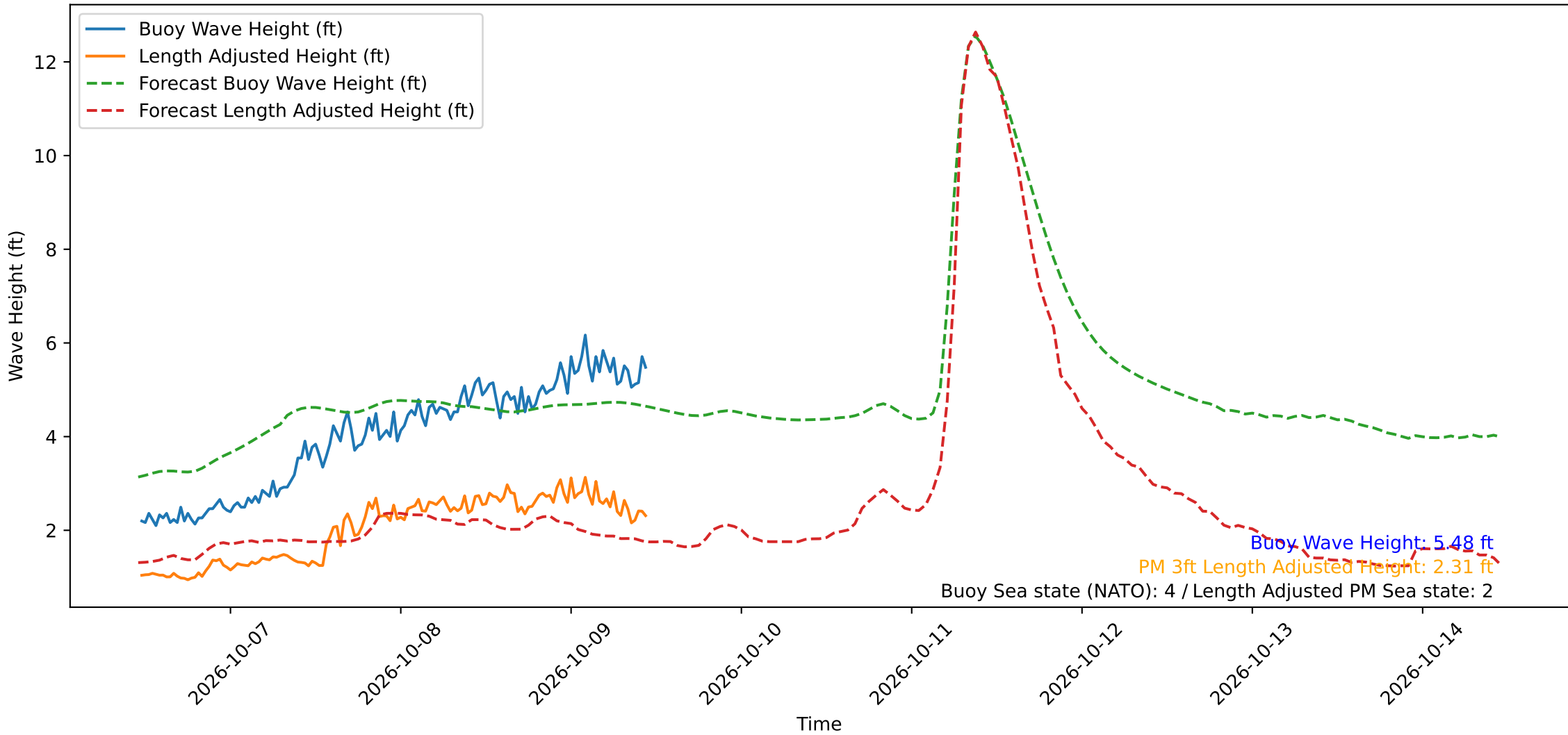
Wave Heights over Time for Green Beach at 2026-10-09 11:11:11
