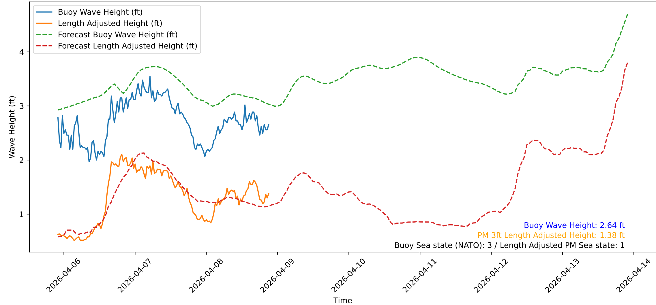
Wave Heights over Time for Red Beach at 2026-04-08 21:40:47
