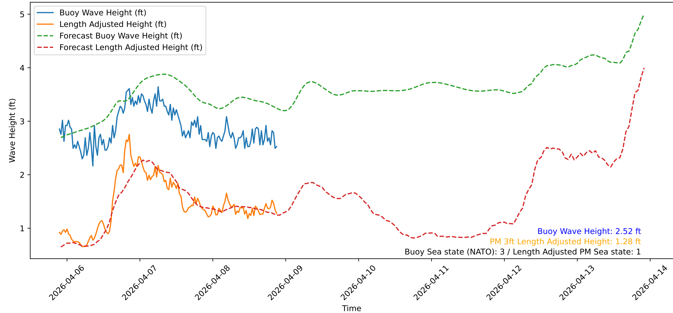
Wave Heights over Time for Oceanside Harbor at 2026-04-08 21:40:31
