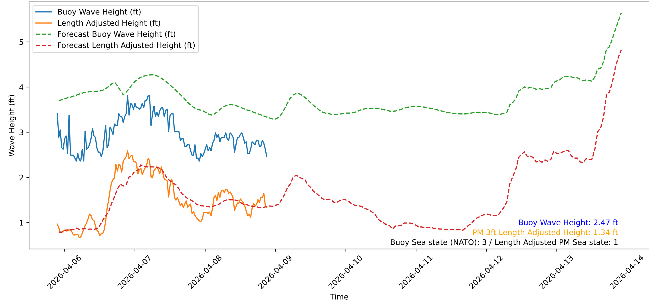
Wave Heights over Time for Green Beach at 2026-04-08 21:41:10
