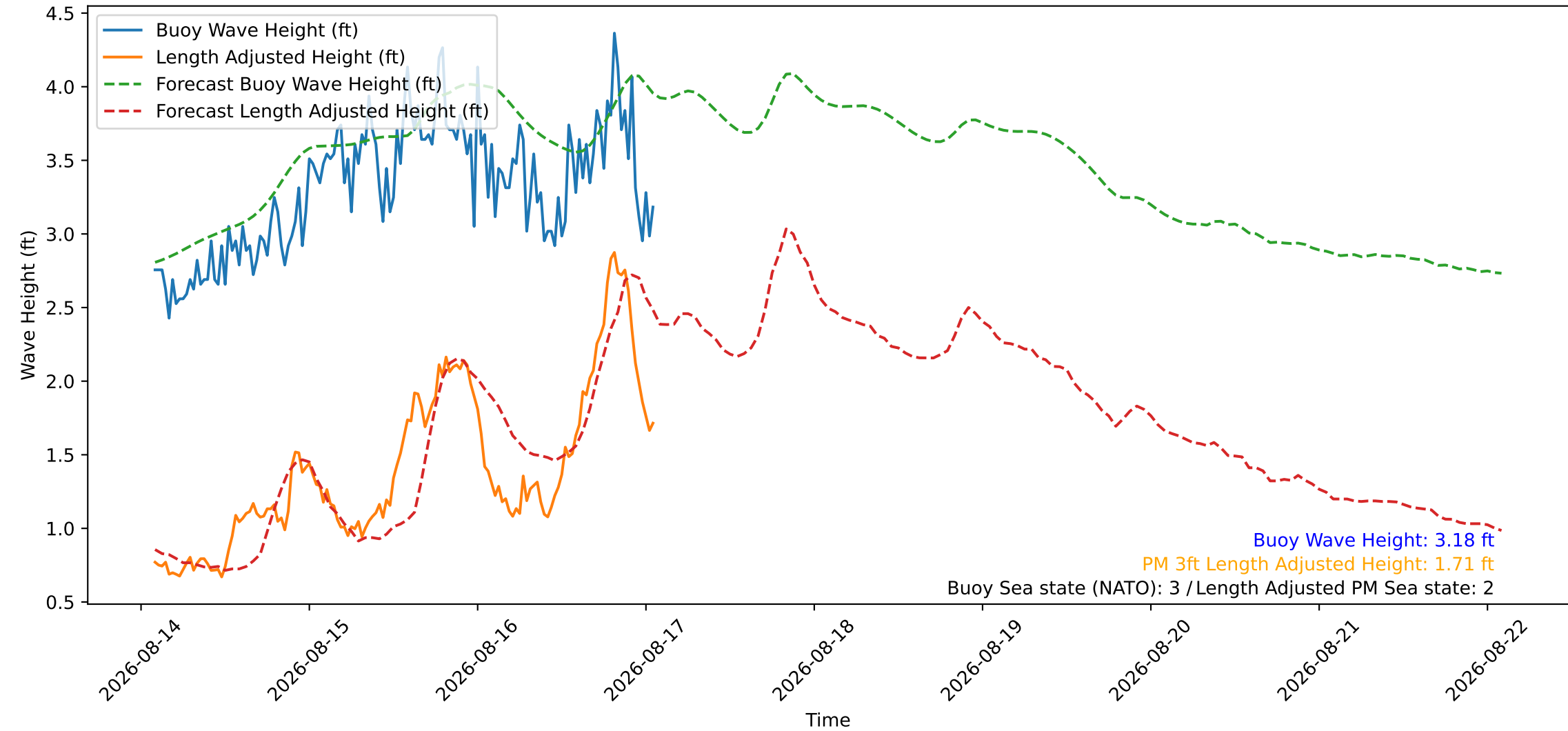
Wave Heights over Time for Green Beach at 2026-08-17 01:41:08
