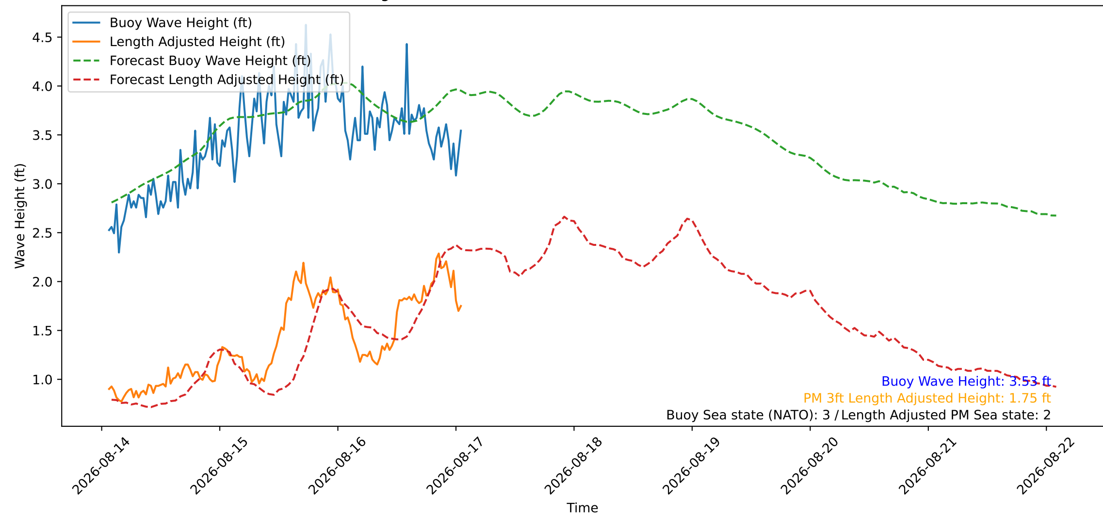
Wave Heights over Time for Oceanside Harbor at 2026-08-17 01:40:26
