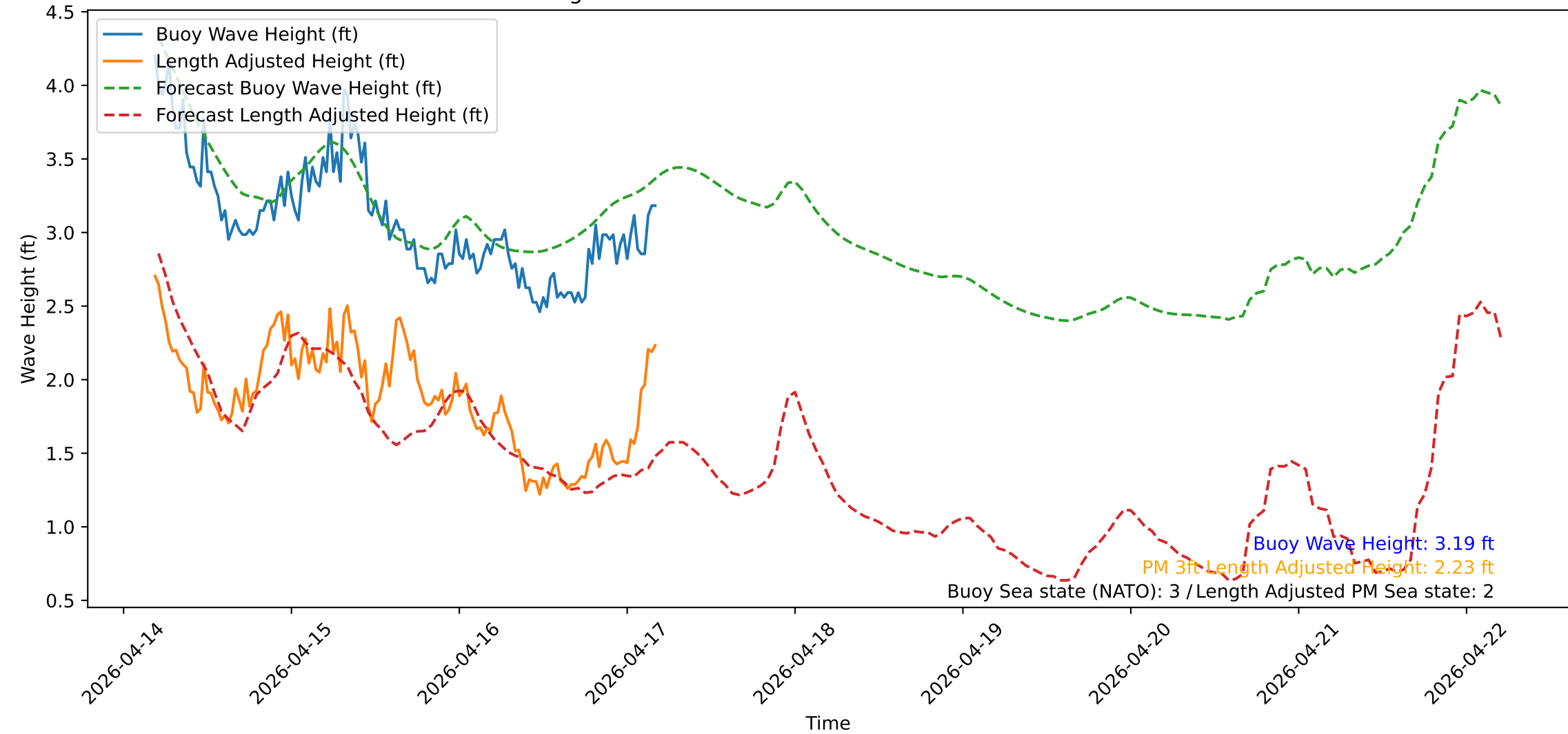
Wave Heights over Time for Green Beach at 2026-04-17 04:41:14
