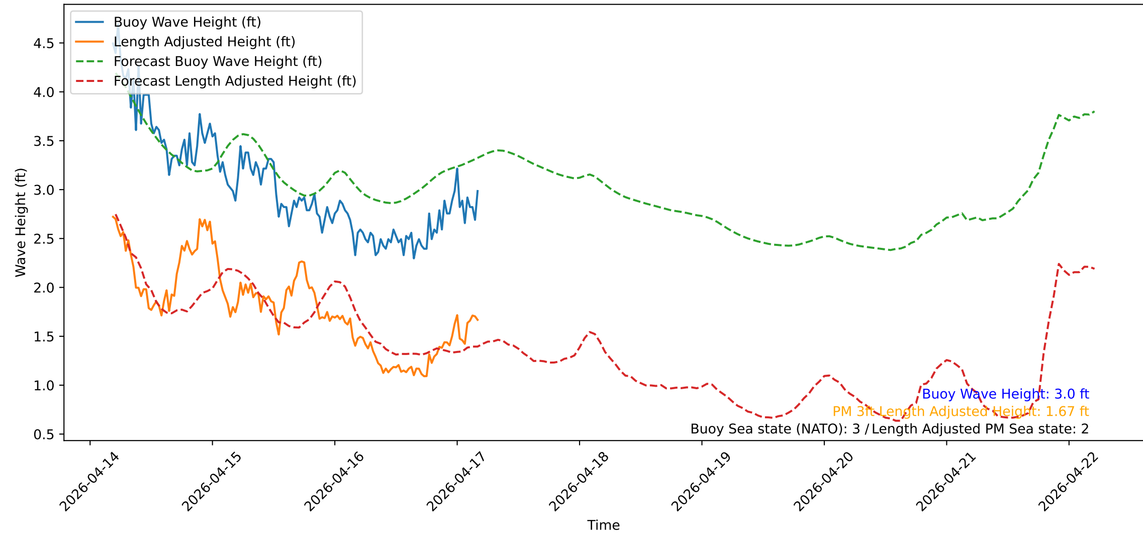
Wave Heights over Time for Oceanside Harbor at 2026-04-17 04:40:32
