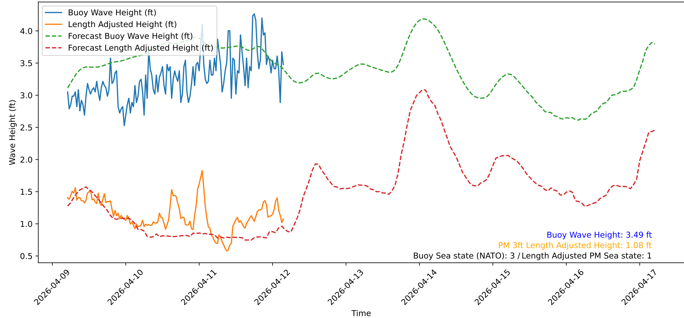
Wave Heights over Time for Red Beach at 2026-04-12 04:50:51
