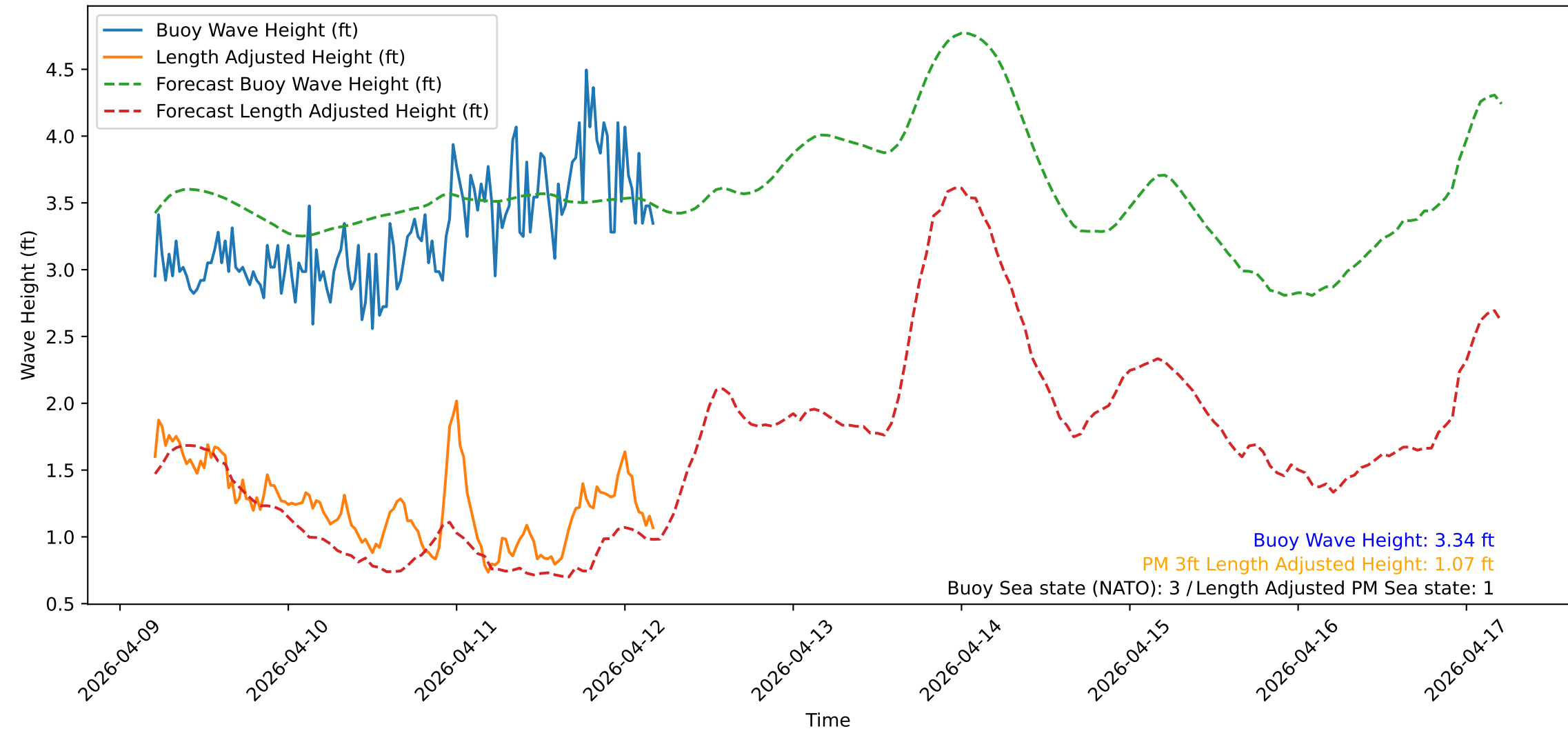
Wave Heights over Time for Green Beach at 2026-04-12 04:51:13
