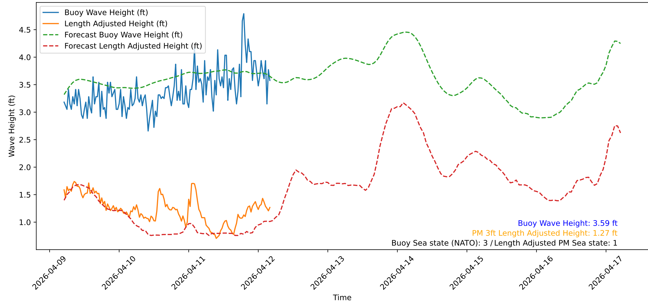
Wave Heights over Time for Oceanside Harbor at 2026-04-12 04:50:31
