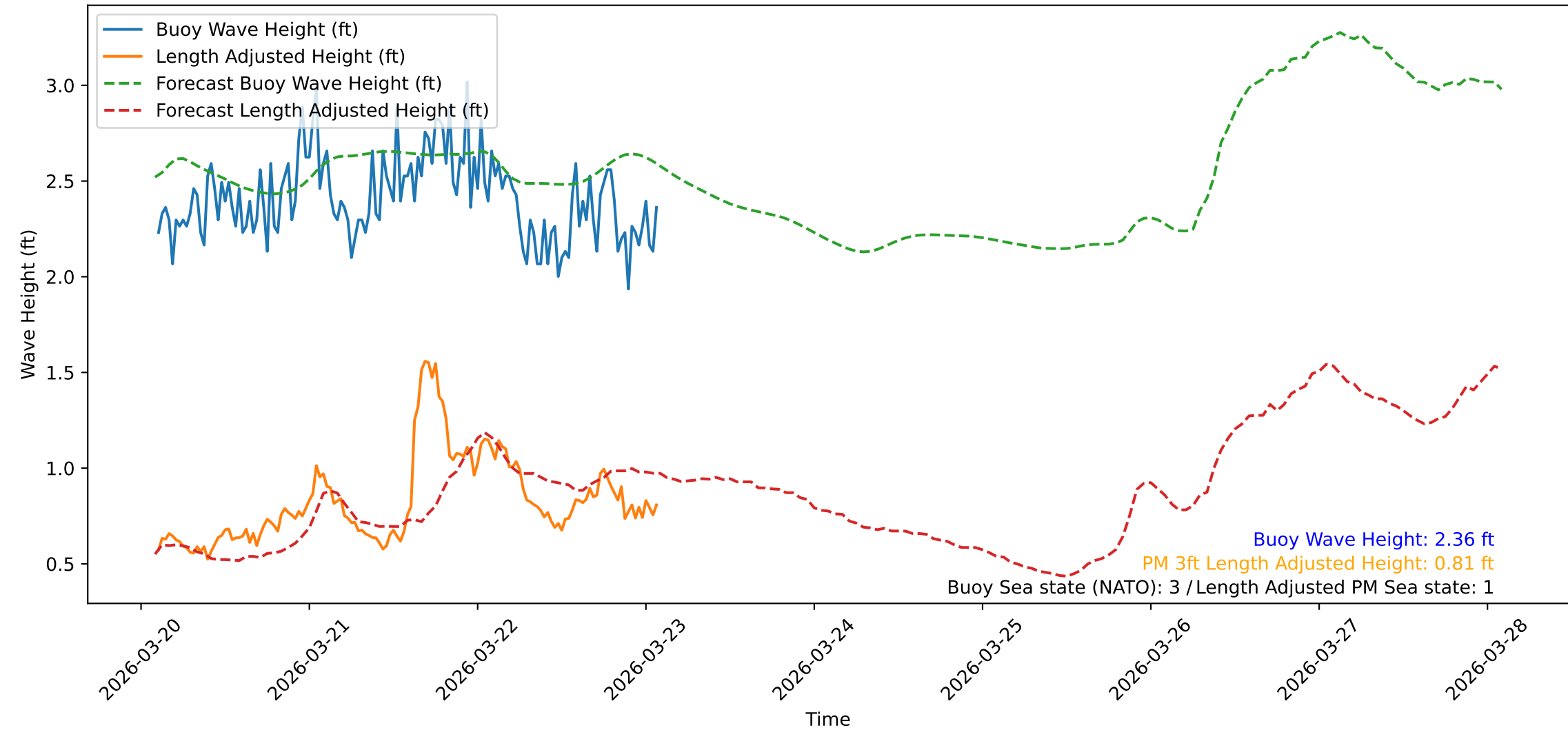
Wave Heights over Time for Oceanside Harbor at 2026-03-23 02:20:32
