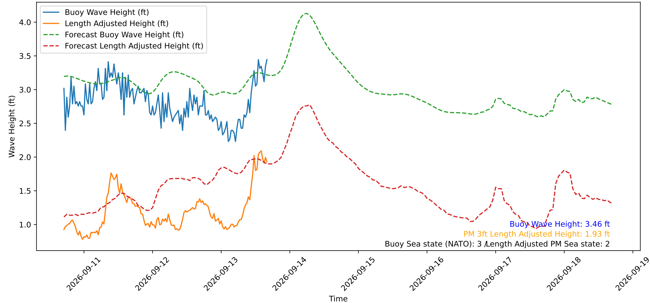
Wave Heights over Time for Red Beach at 2026-09-13 16:40:49
