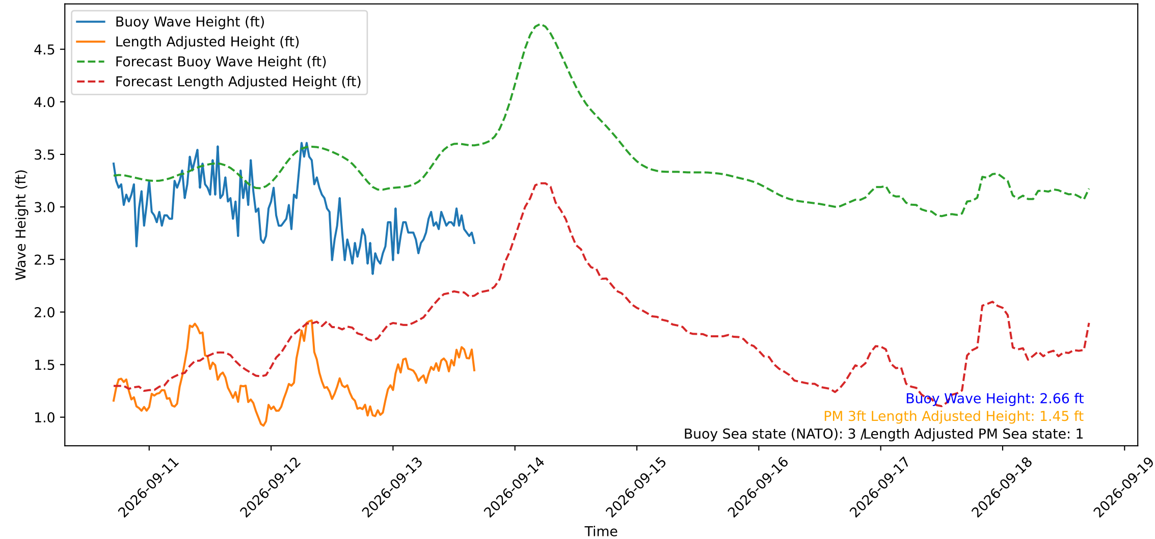
Wave Heights over Time for Green Beach at 2026-09-13 16:41:12
