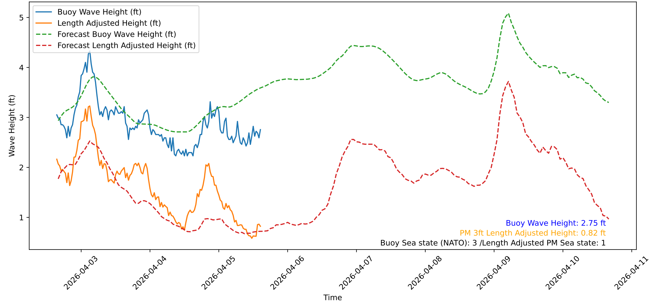
Wave Heights over Time for Green Beach at 2026-04-05 15:31:12
