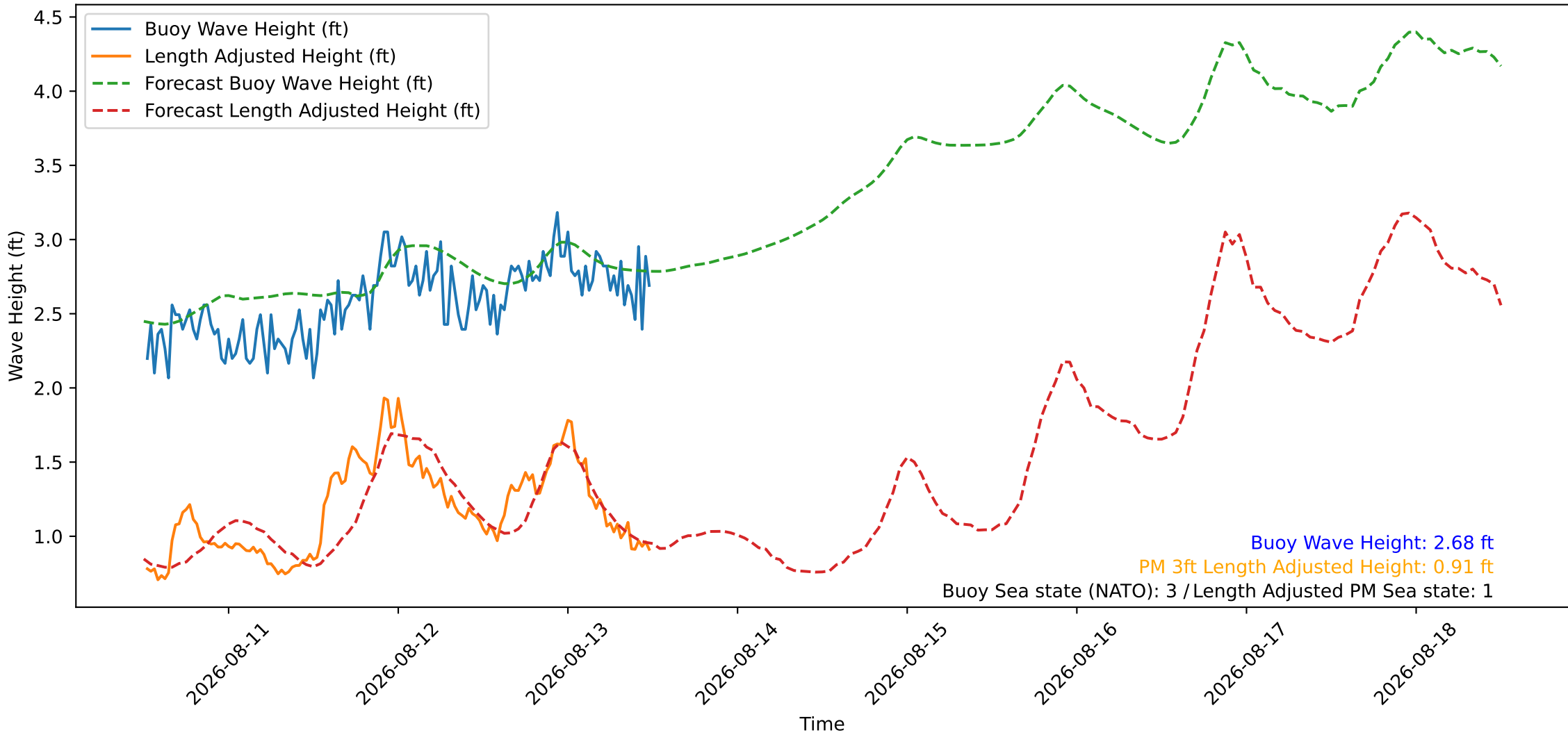
Wave Heights over Time for Oceanside Harbor at 2026-08-13 12:20:26
