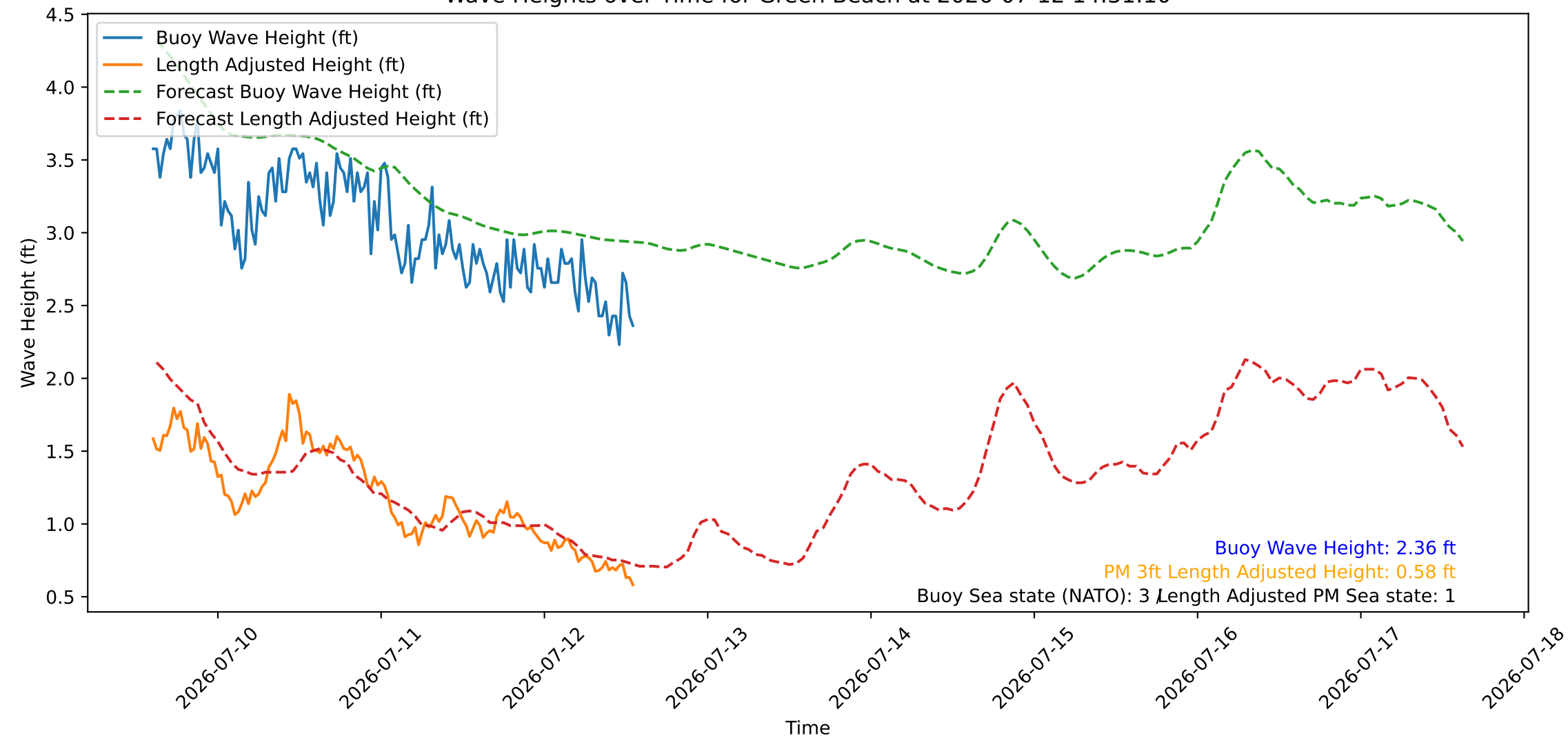
Wave Heights over Time for Green Beach at 2026-07-12 14:31:10
