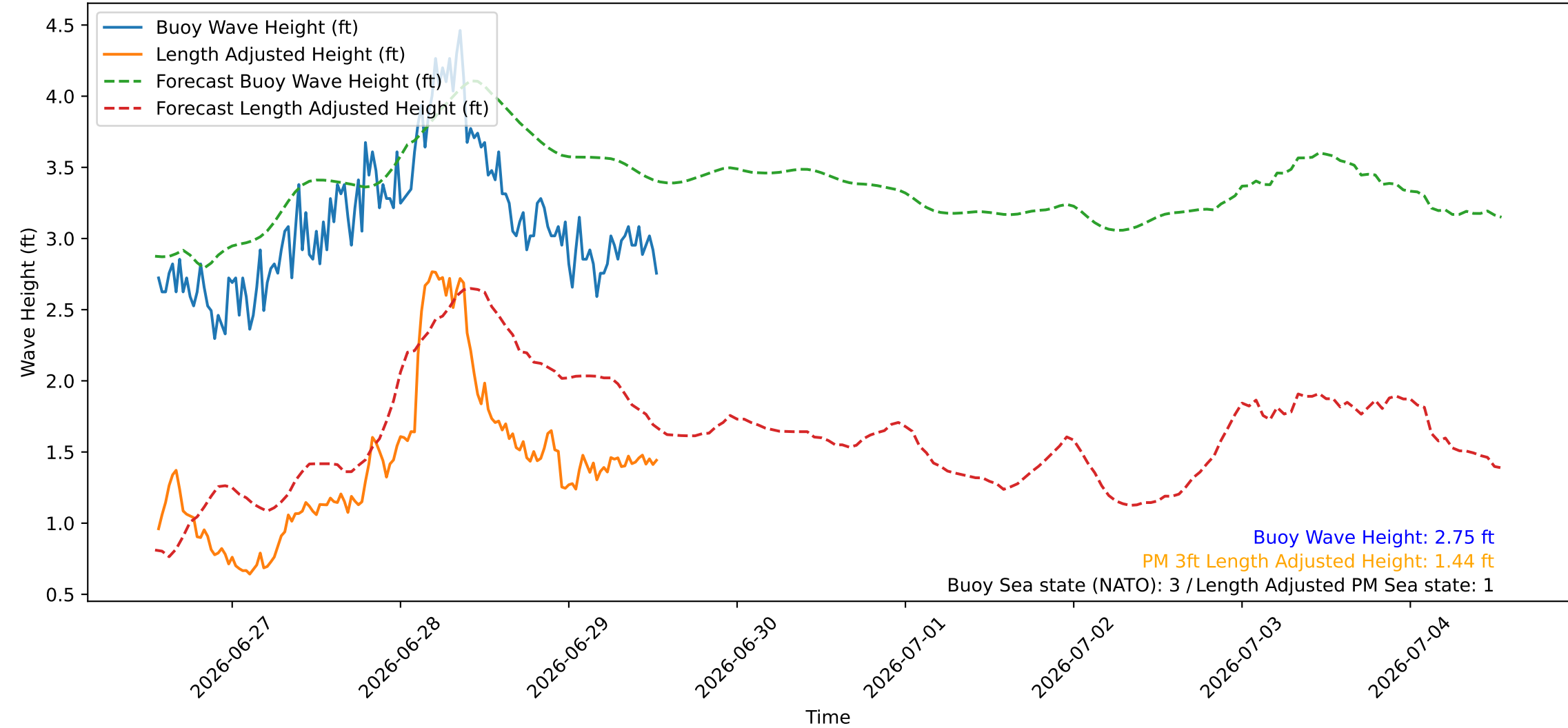
Wave Heights over Time for Red Beach at 2026-06-29 13:20:46
