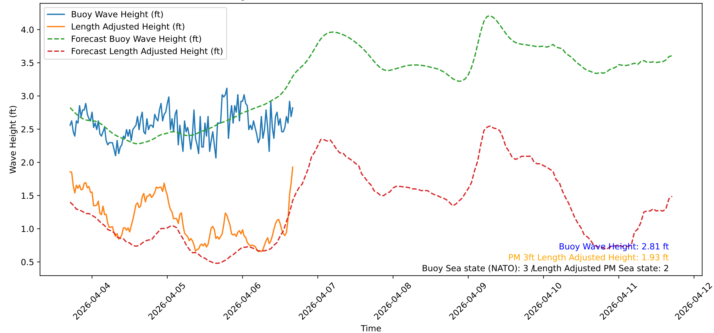
Wave Heights over Time for Oceanside Harbor at 2026-04-06 16:50:31
