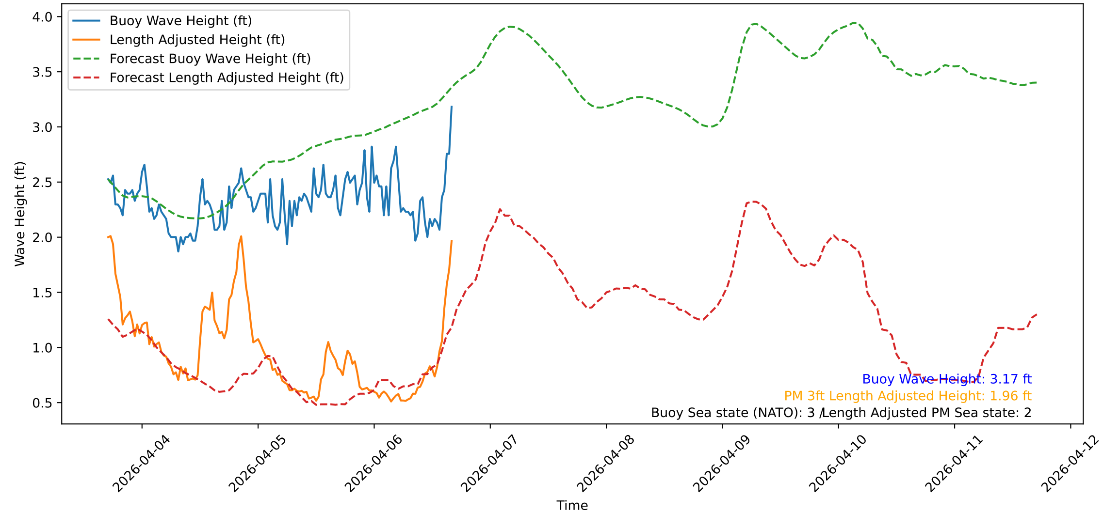
Wave Heights over Time for Red Beach at 2026-04-06 16:50:47
