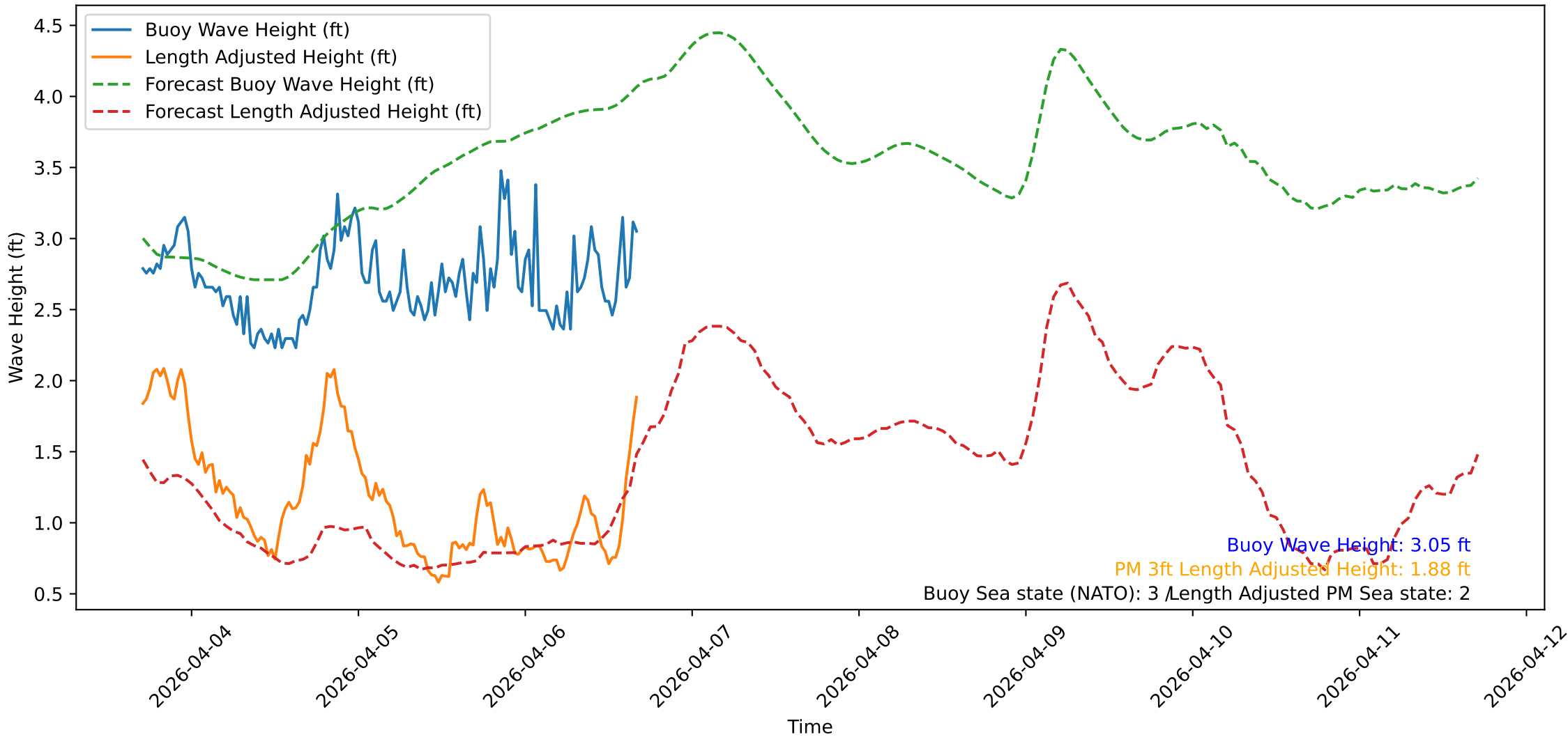
Wave Heights over Time for Green Beach at 2026-04-06 16:51:09
