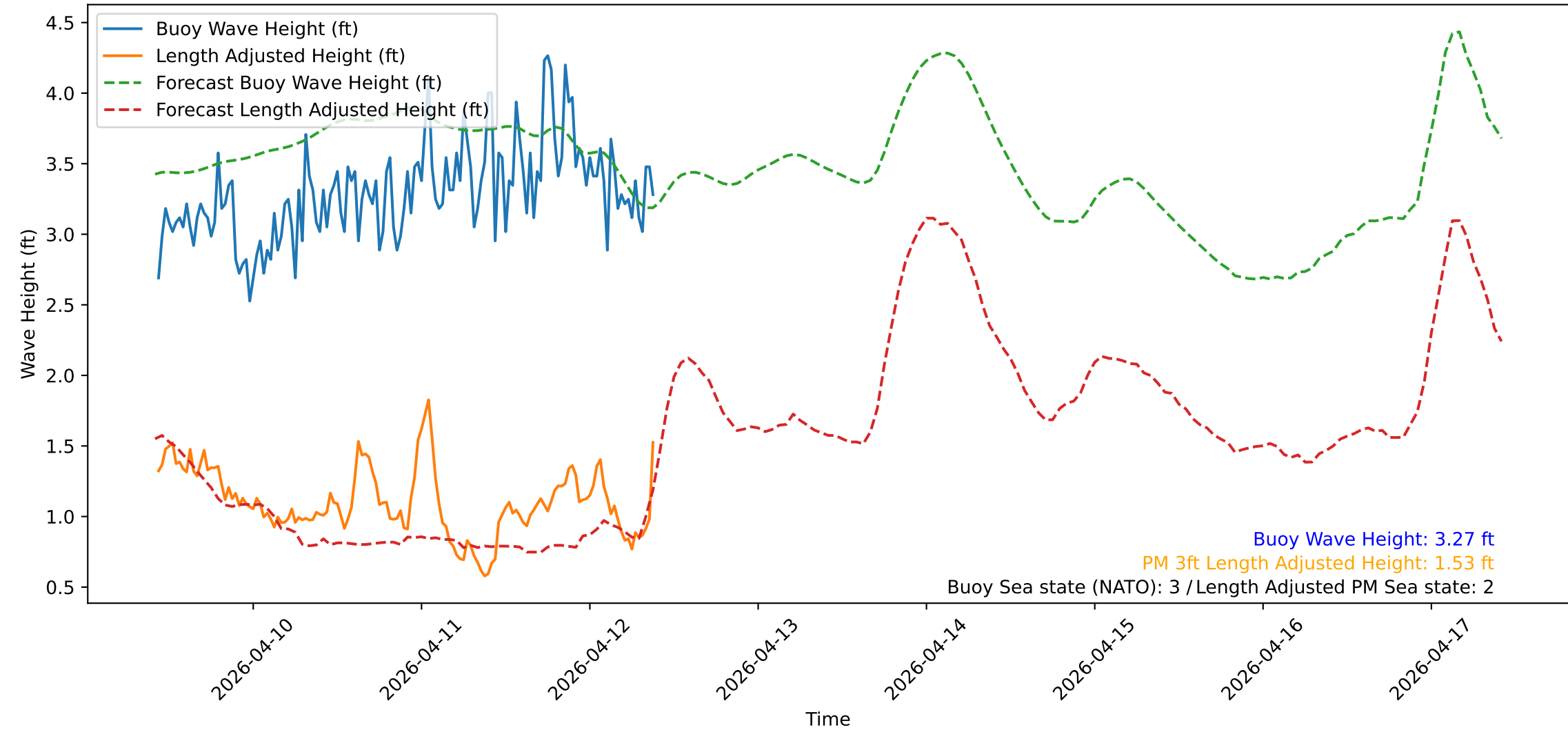
Wave Heights over Time for Red Beach at 2026-04-12 10:20:51
