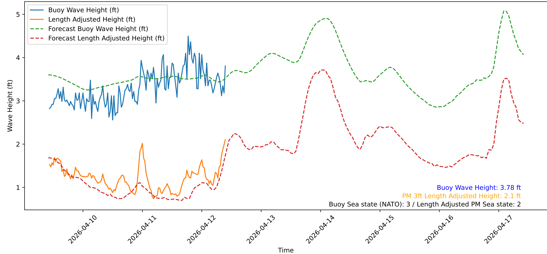
Wave Heights over Time for Green Beach at 2026-04-12 10:21:13
