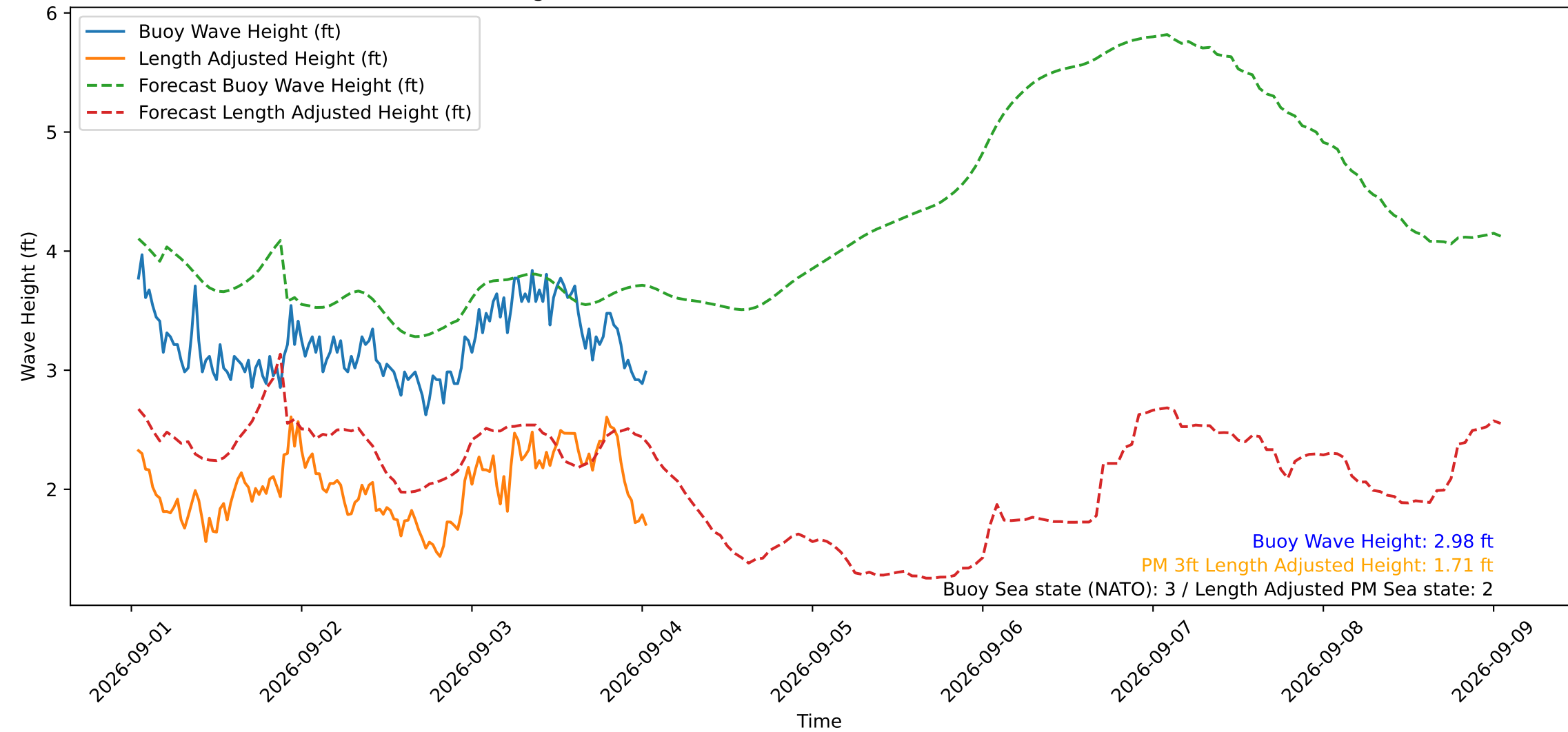
Wave Heights over Time for Oceanside Harbor at 2026-09-04 01:10:29
