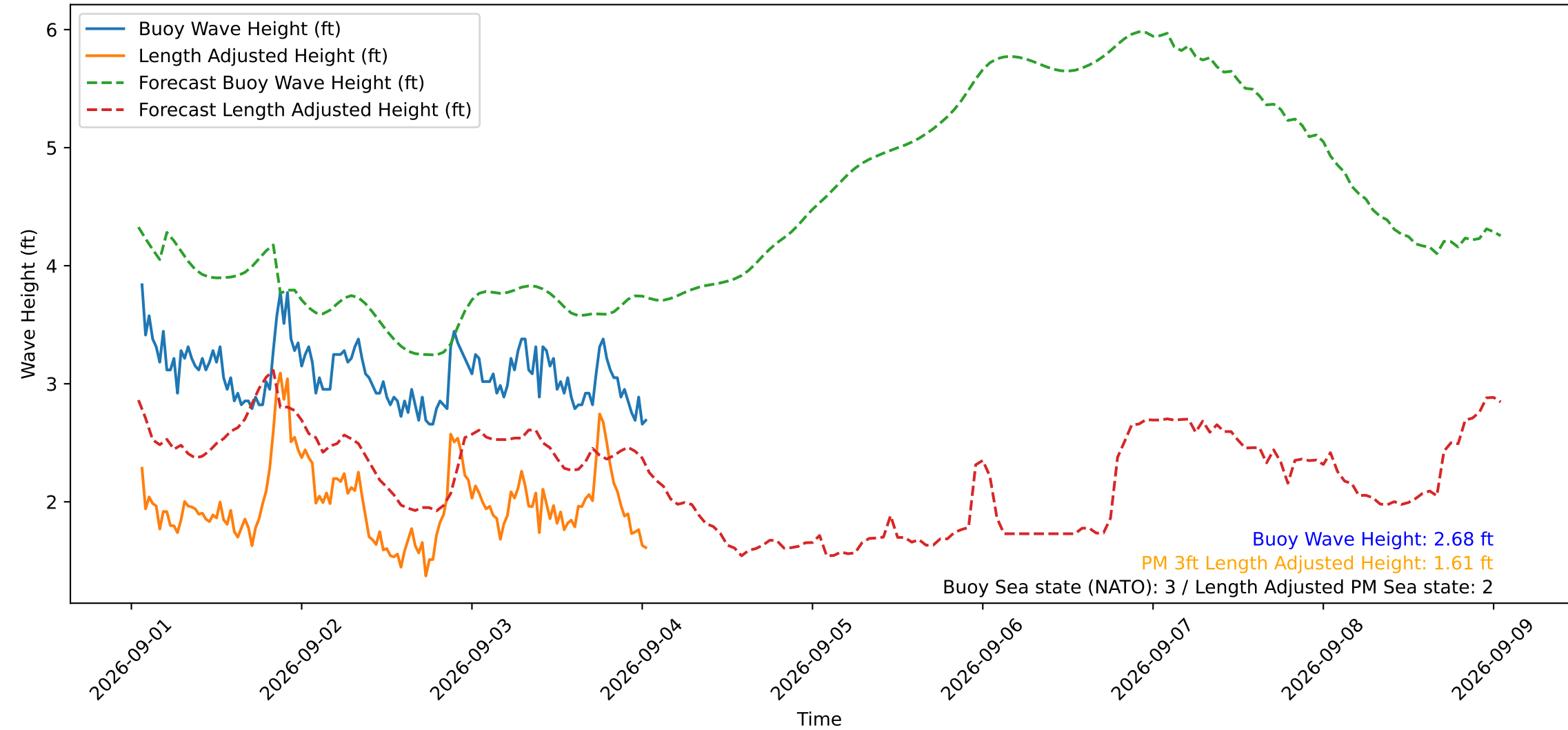
Wave Heights over Time for Green Beach at 2026-09-04 01:11:12
