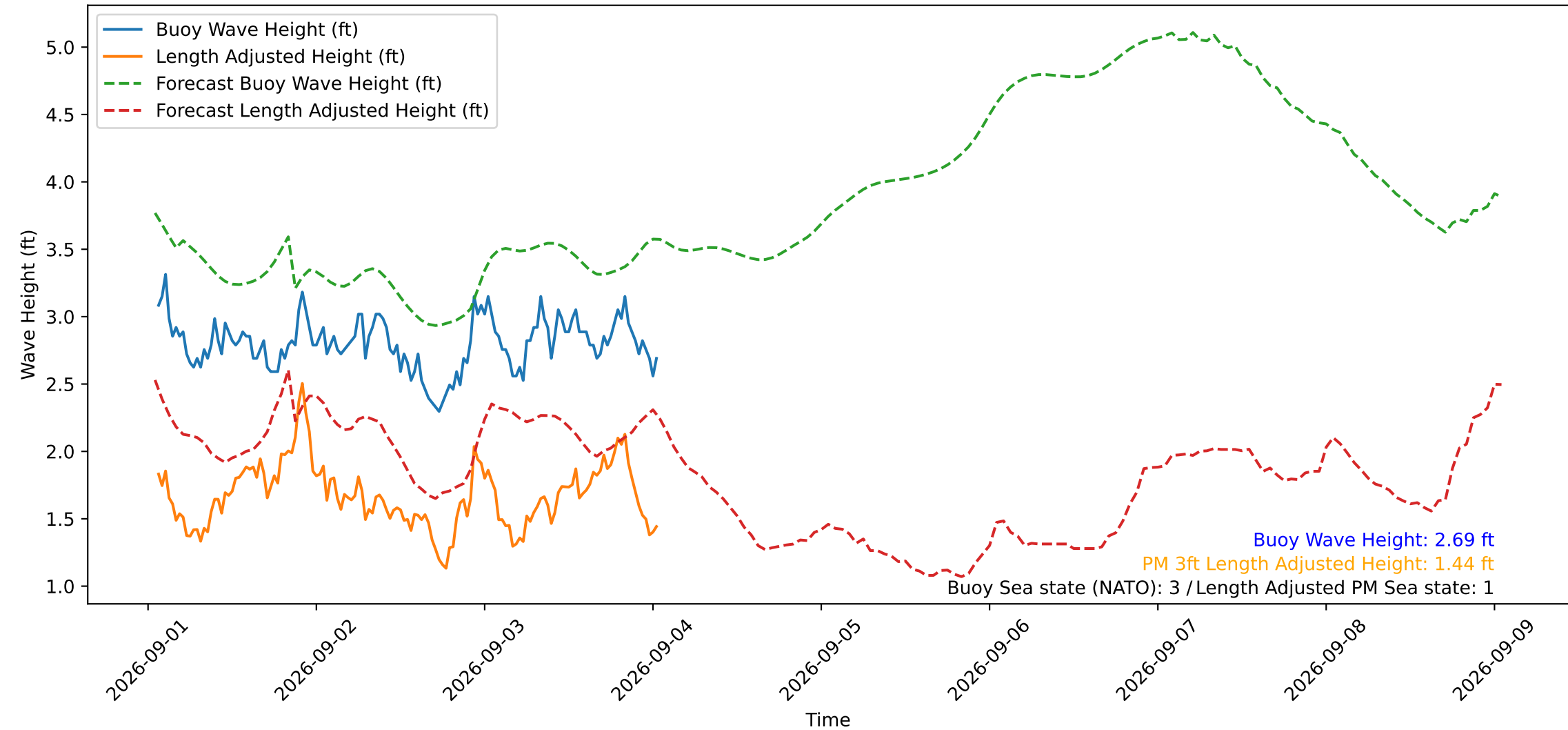
Wave Heights over Time for Red Beach at 2026-09-04 01:10:49
