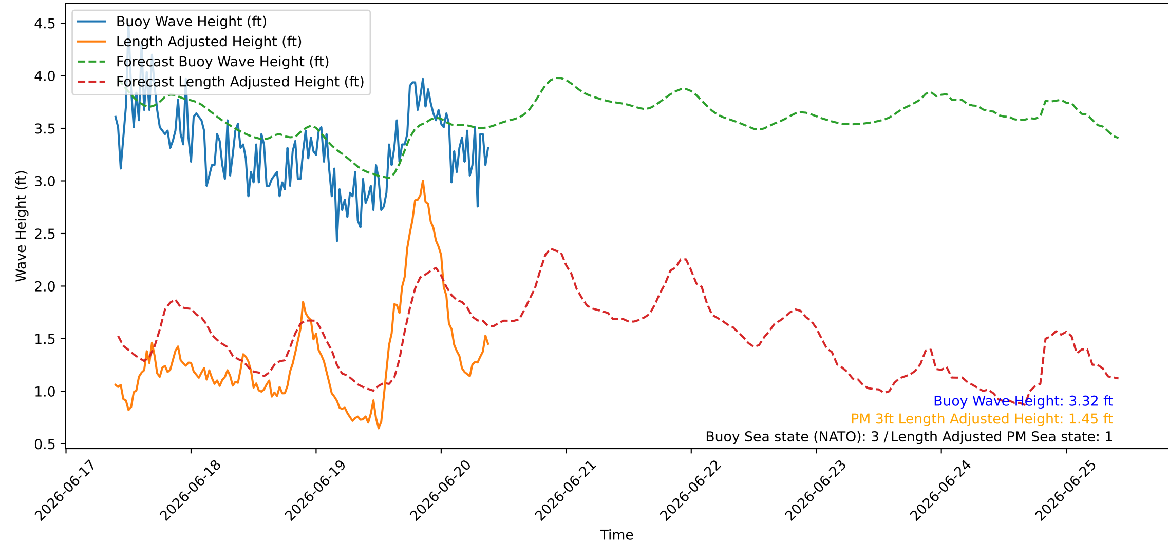
Wave Heights over Time for Green Beach at 2026-06-20 09:41:08
