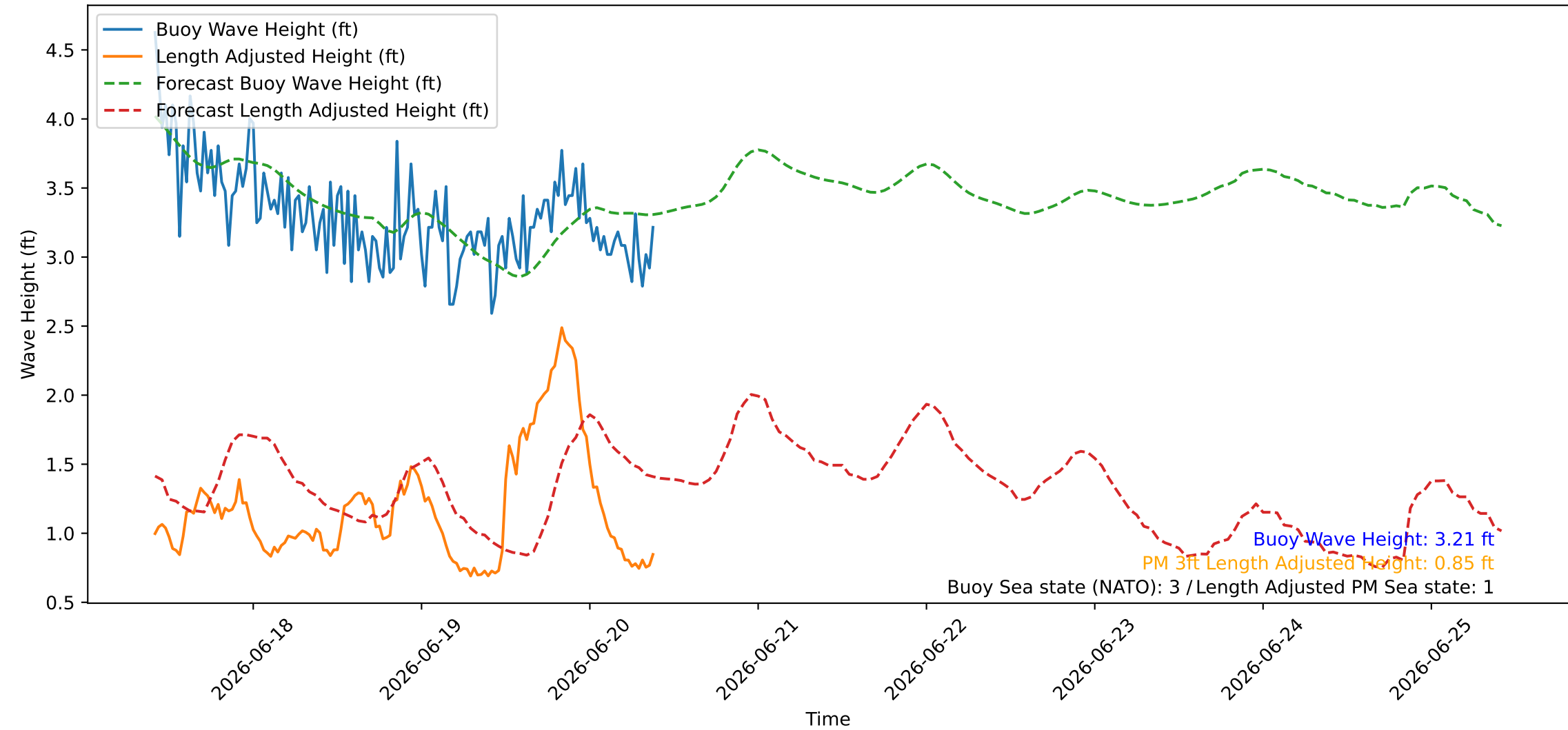
Wave Heights over Time for Red Beach at 2026-06-20 09:40:45
