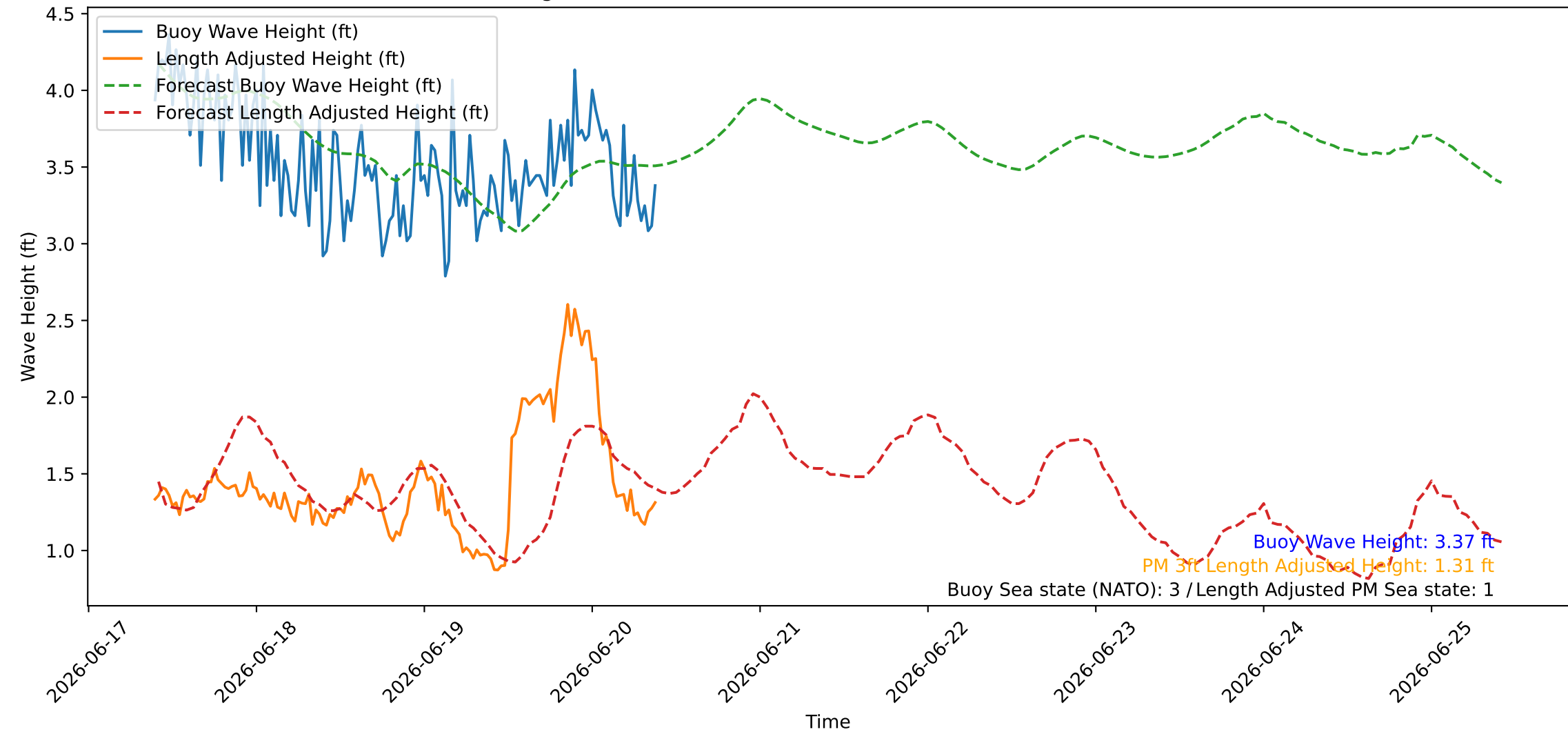
Wave Heights over Time for Oceanside Harbor at 2026-06-20 09:40:26
