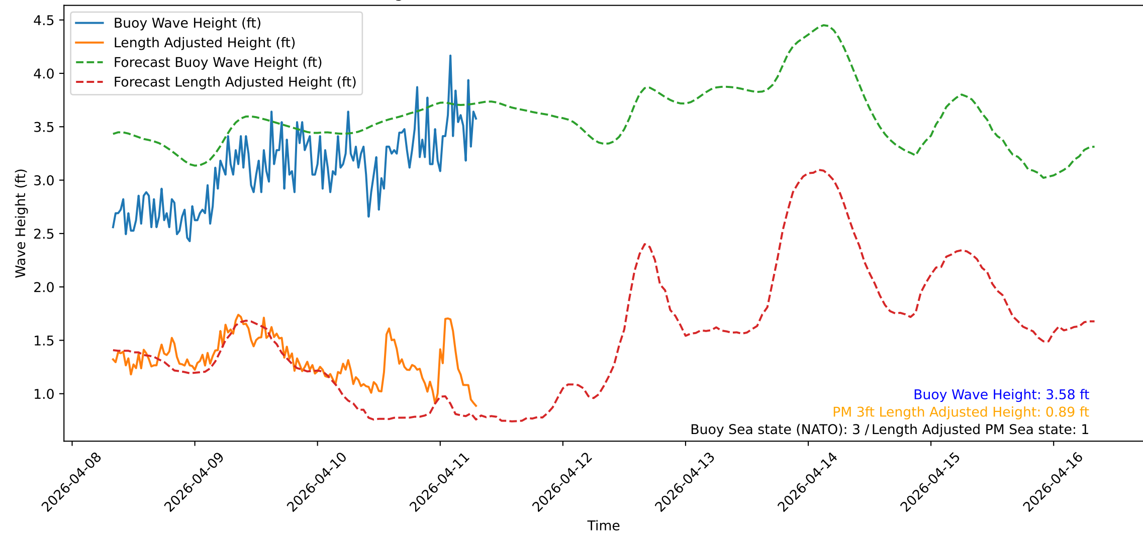
Wave Heights over Time for Oceanside Harbor at 2026-04-11 07:50:31
