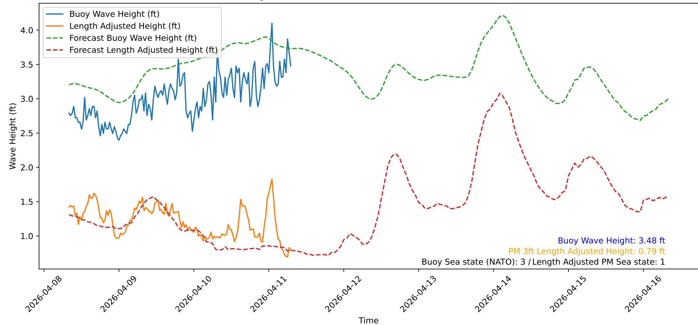
Wave Heights over Time for Red Beach at 2026-04-11 07:50:51
