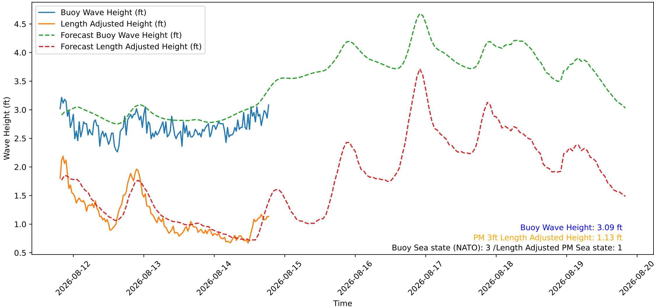
Wave Heights over Time for Green Beach at 2026-08-14 19:31:09
