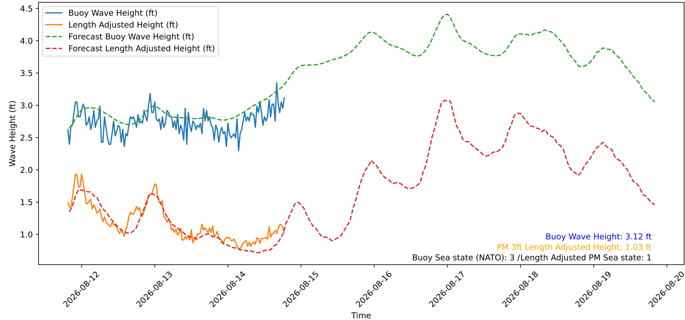
Wave Heights over Time for Oceanside Harbor at 2026-08-14 19:30:27
