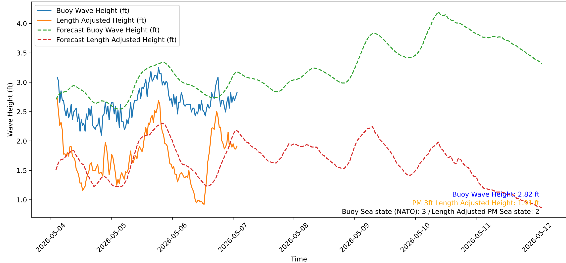
Wave Heights over Time for Oceanside Harbor at 2026-05-07 02:20:31
