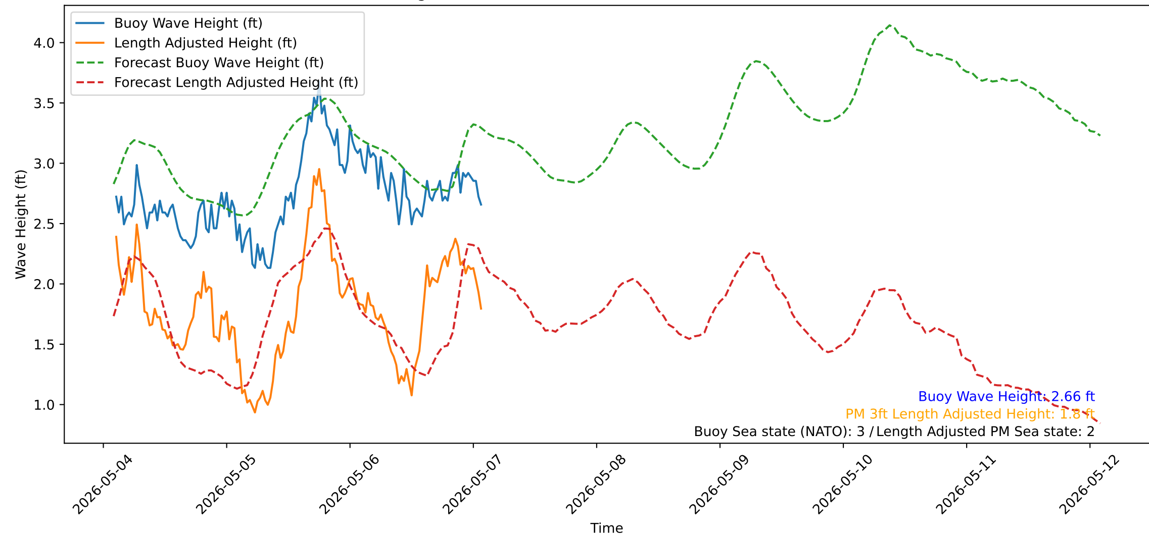
Wave Heights over Time for Green Beach at 2026-05-07 02:21:14
