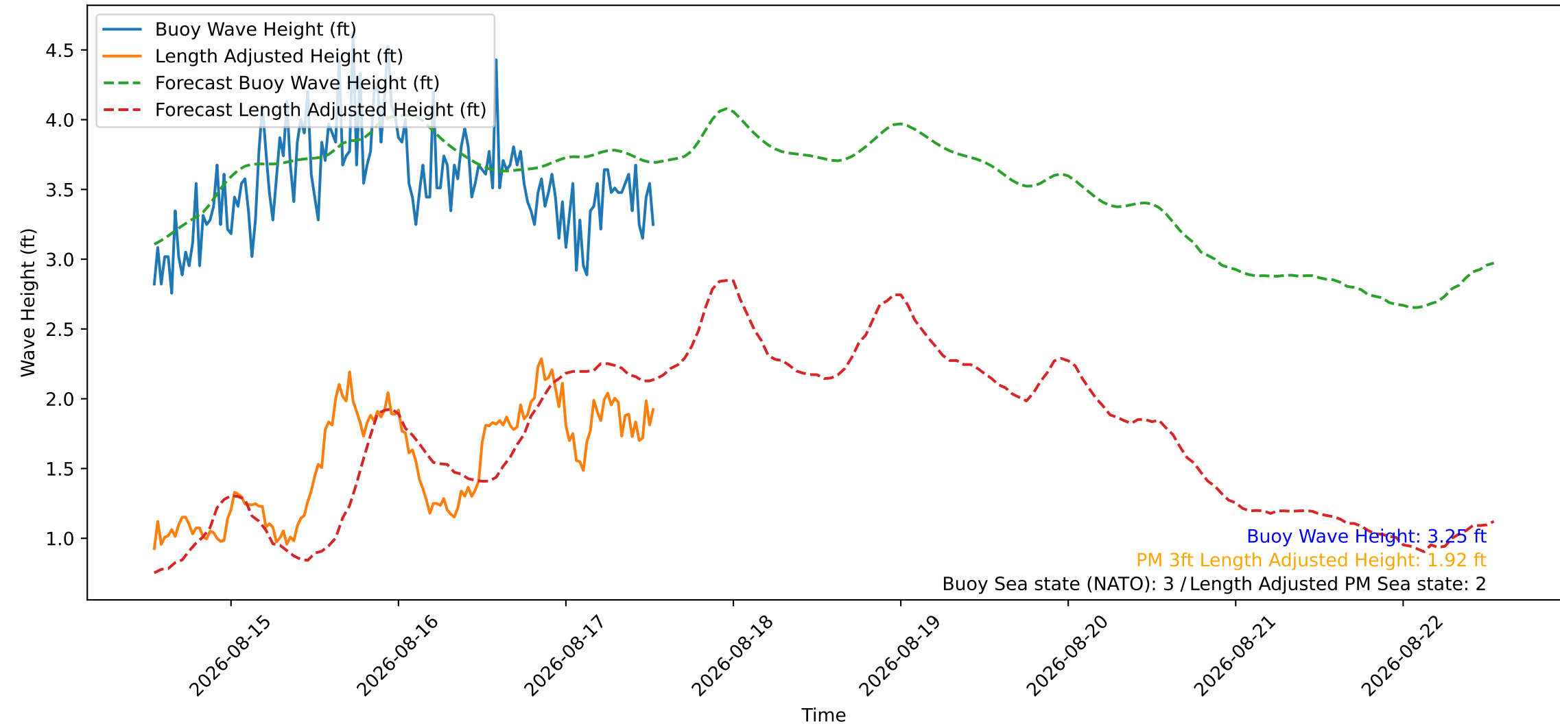
Wave Heights over Time for Oceanside Harbor at 2026-08-17 13:10:26
