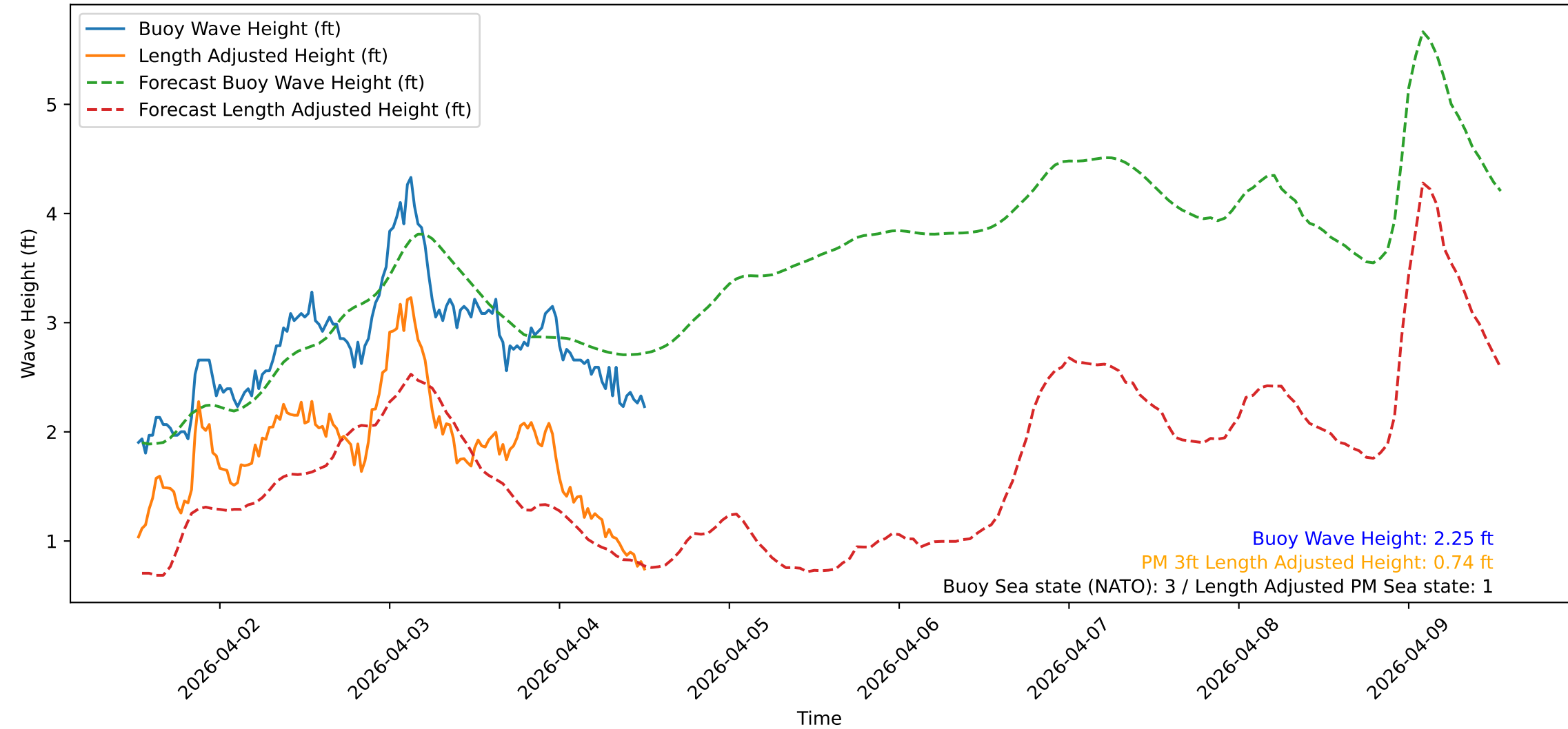
Wave Heights over Time for Green Beach at 2026-04-04 12:41:09
