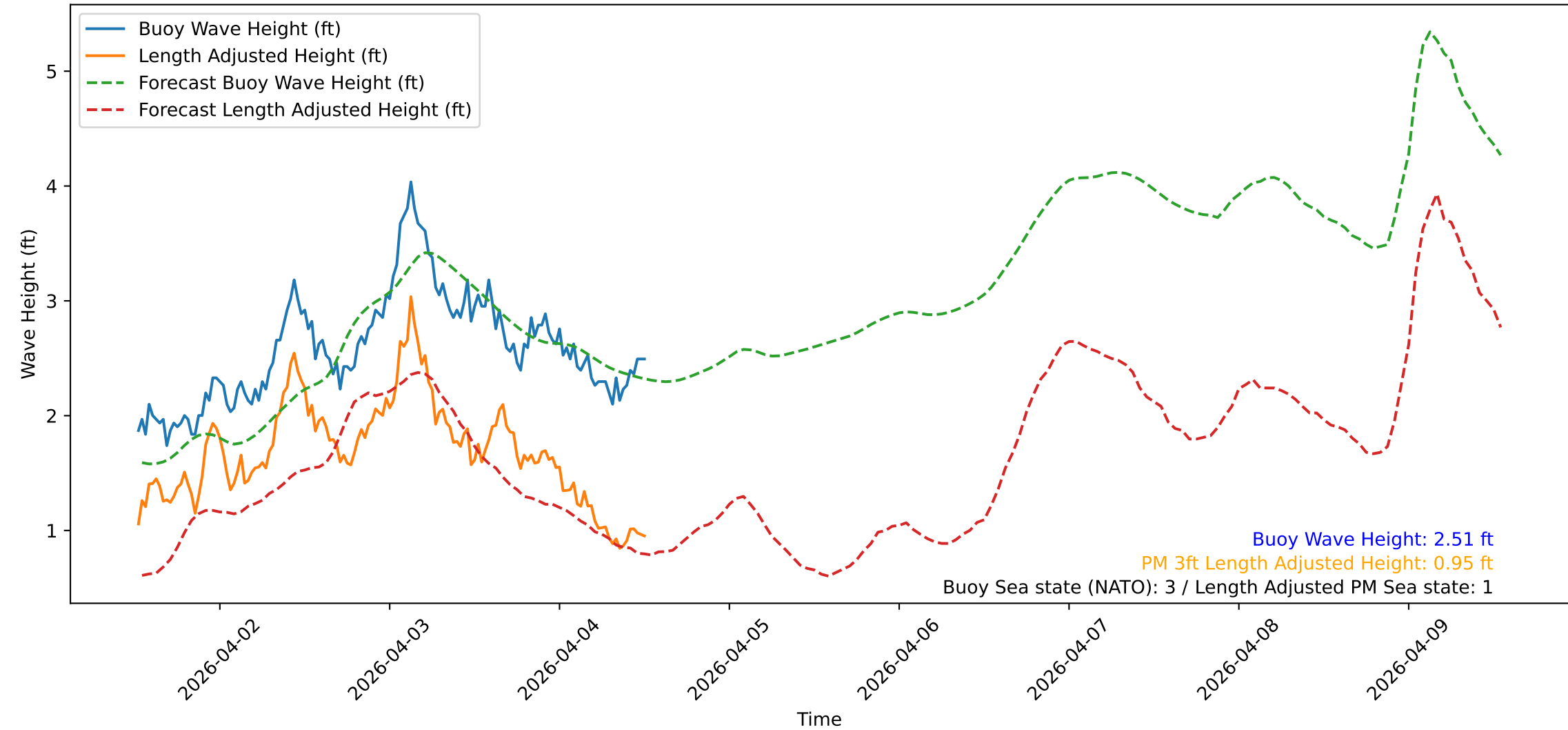
Wave Heights over Time for Oceanside Harbor at 2026-04-04 12:40:31
