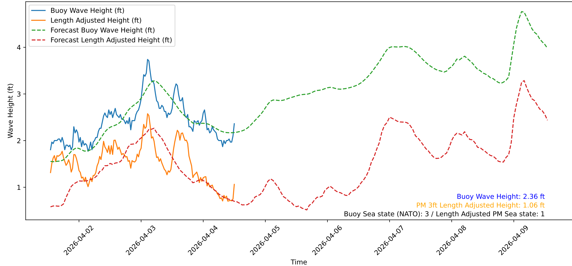
Wave Heights over Time for Red Beach at 2026-04-04 12:40:47
