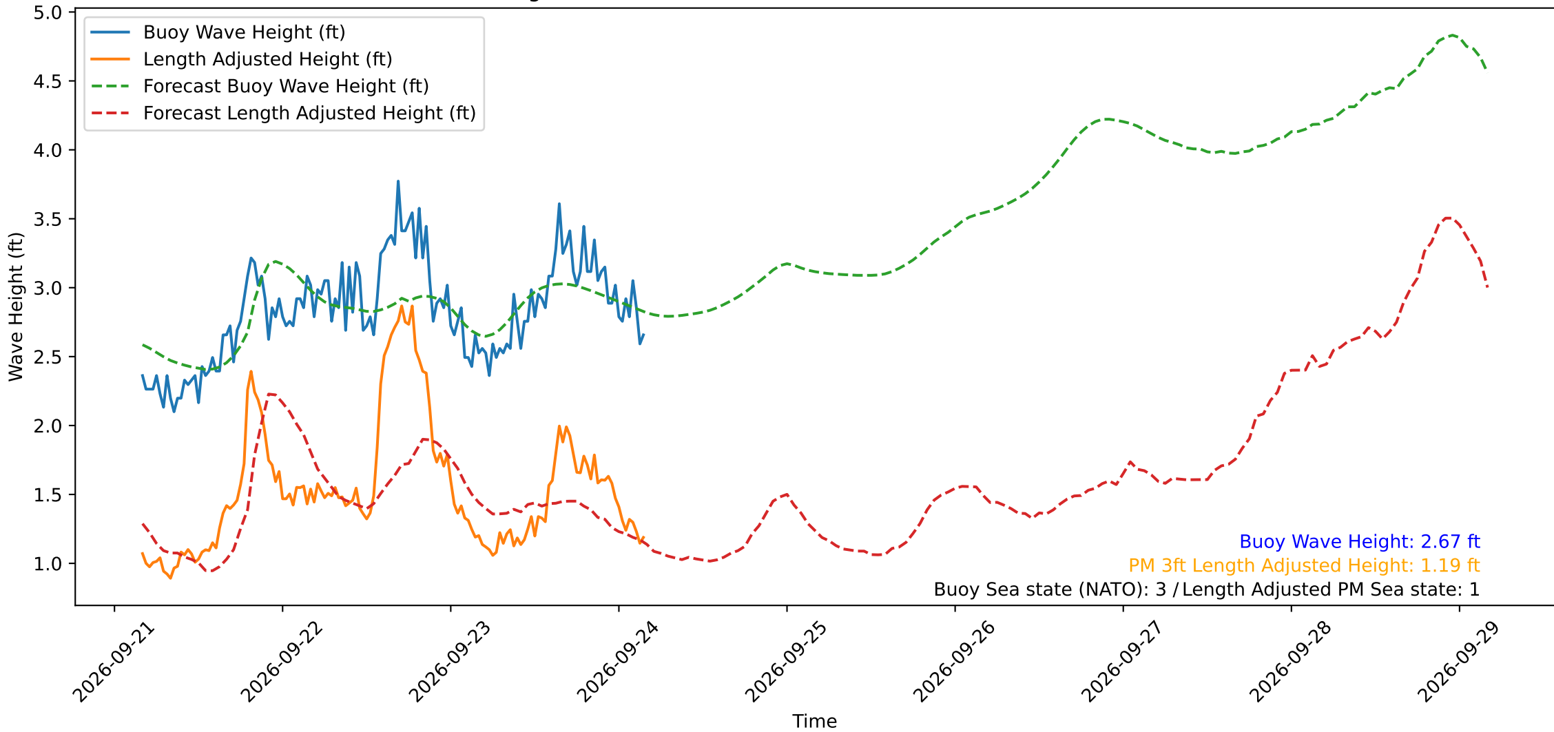
Wave Heights over Time for Oceanside Harbor at 2026-09-24 04:10:29
