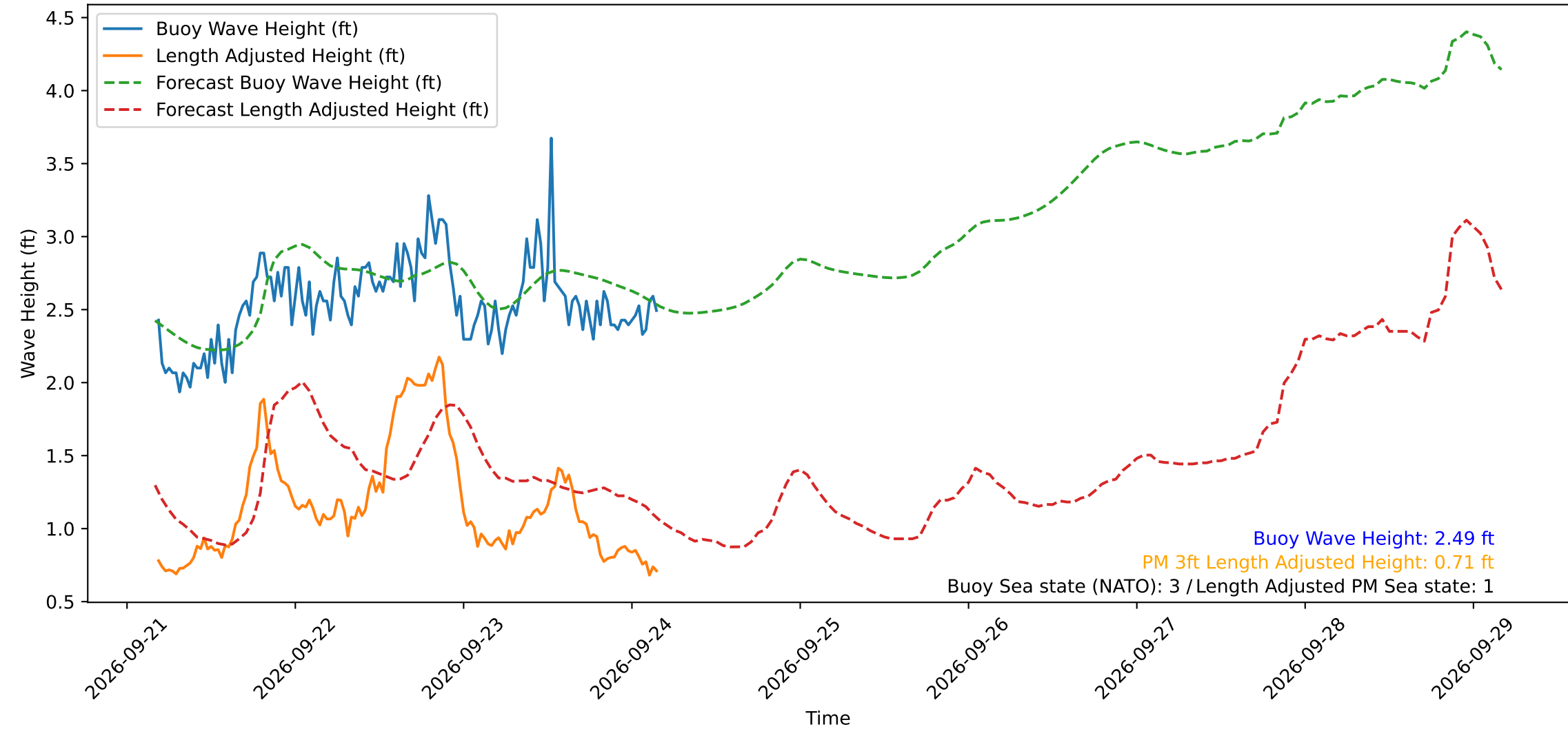
Wave Heights over Time for Red Beach at 2026-09-24 04:10:49
