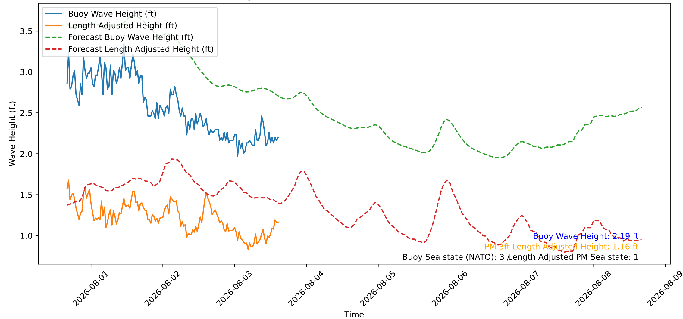
Wave Heights over Time for Red Beach at 2026-08-03 15:30:46
