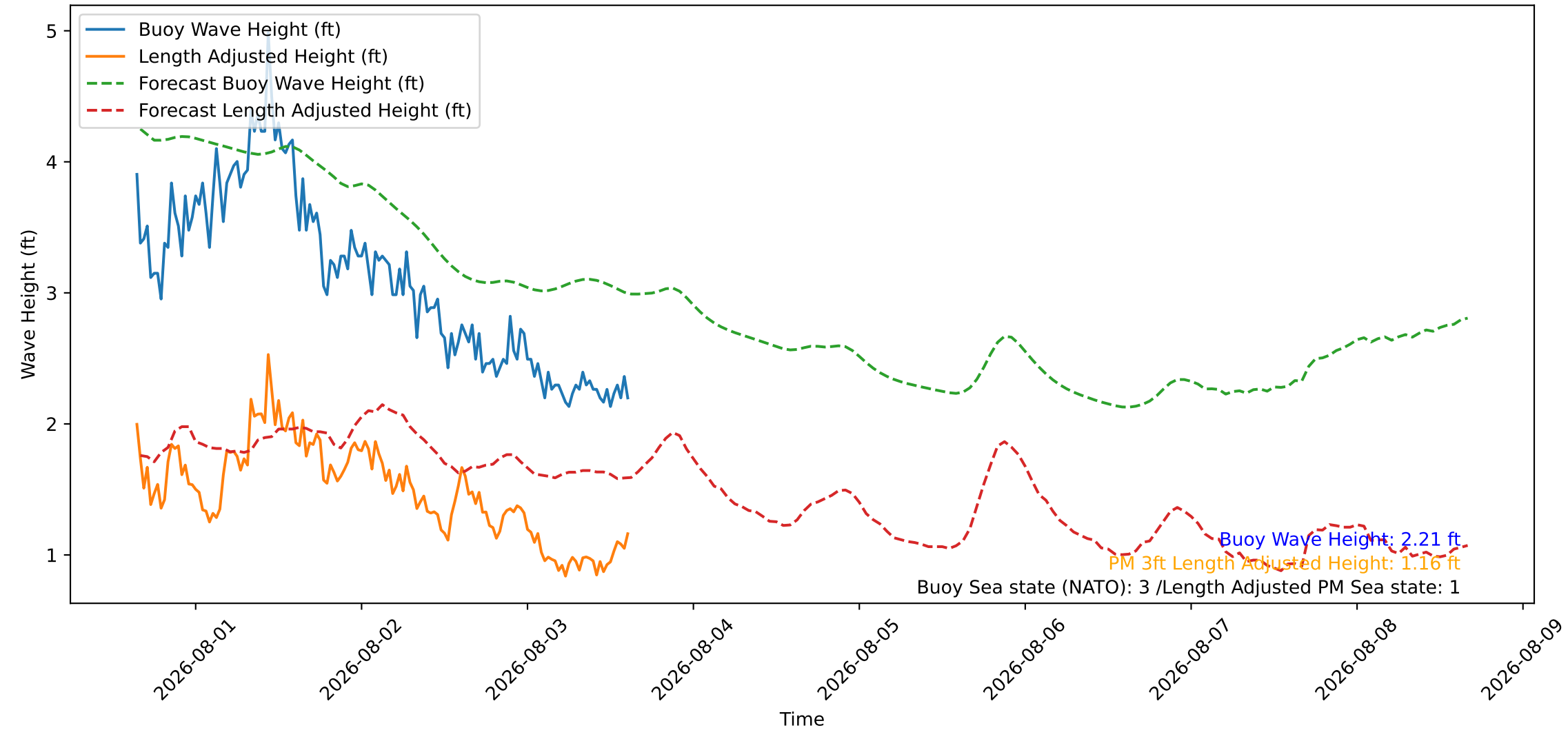
Wave Heights over Time for Green Beach at 2026-08-03 15:31:08
