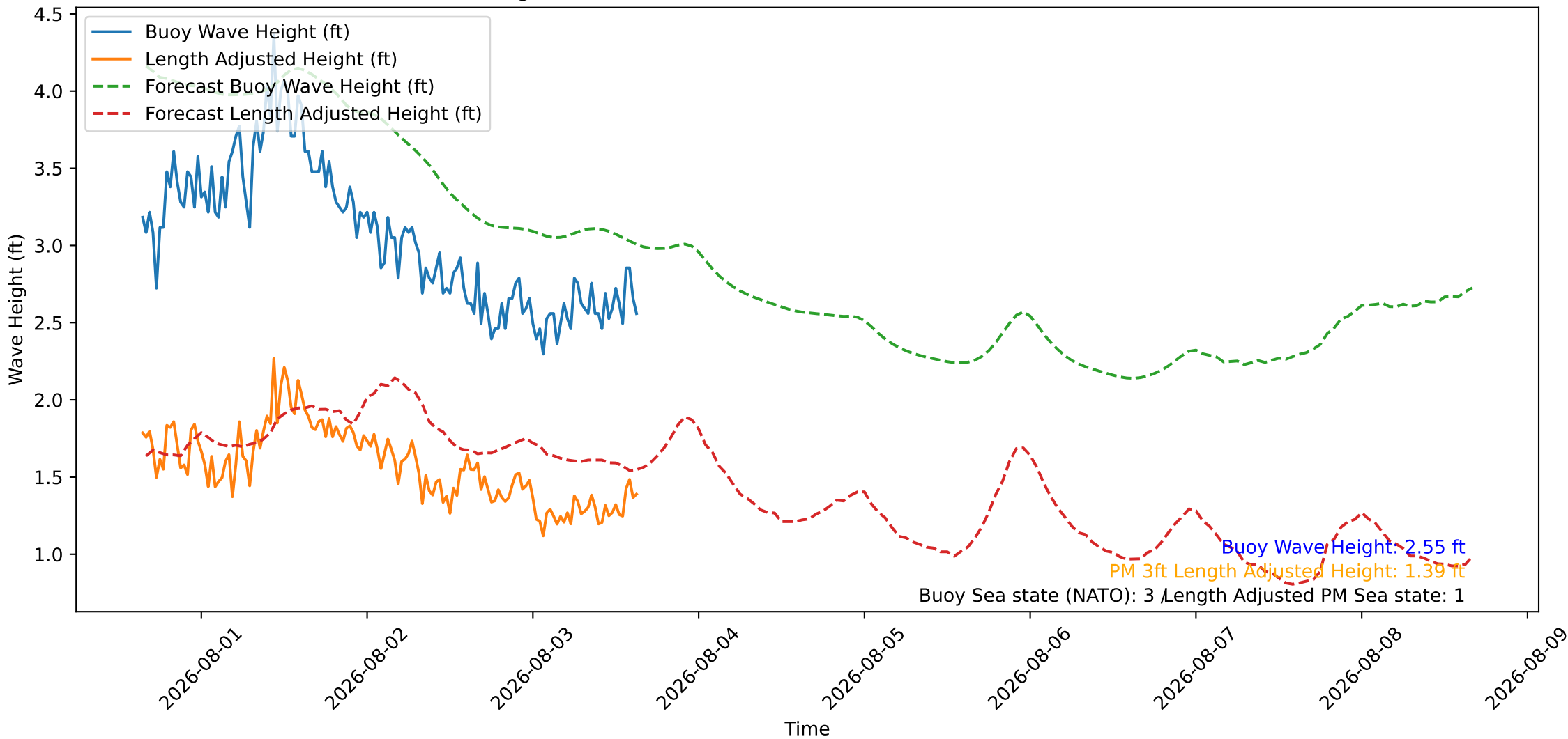
Wave Heights over Time for Oceanside Harbor at 2026-08-03 15:30:27
