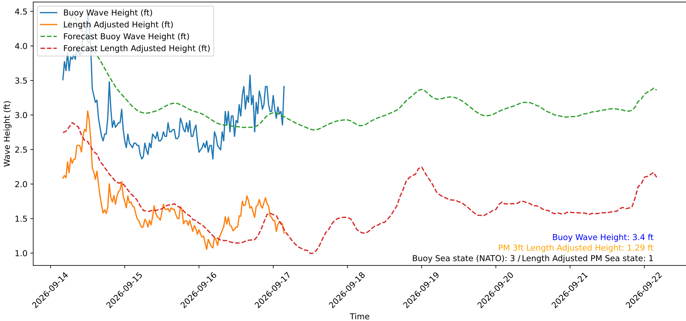
Wave Heights over Time for Oceanside Harbor at 2026-09-17 04:10:29
