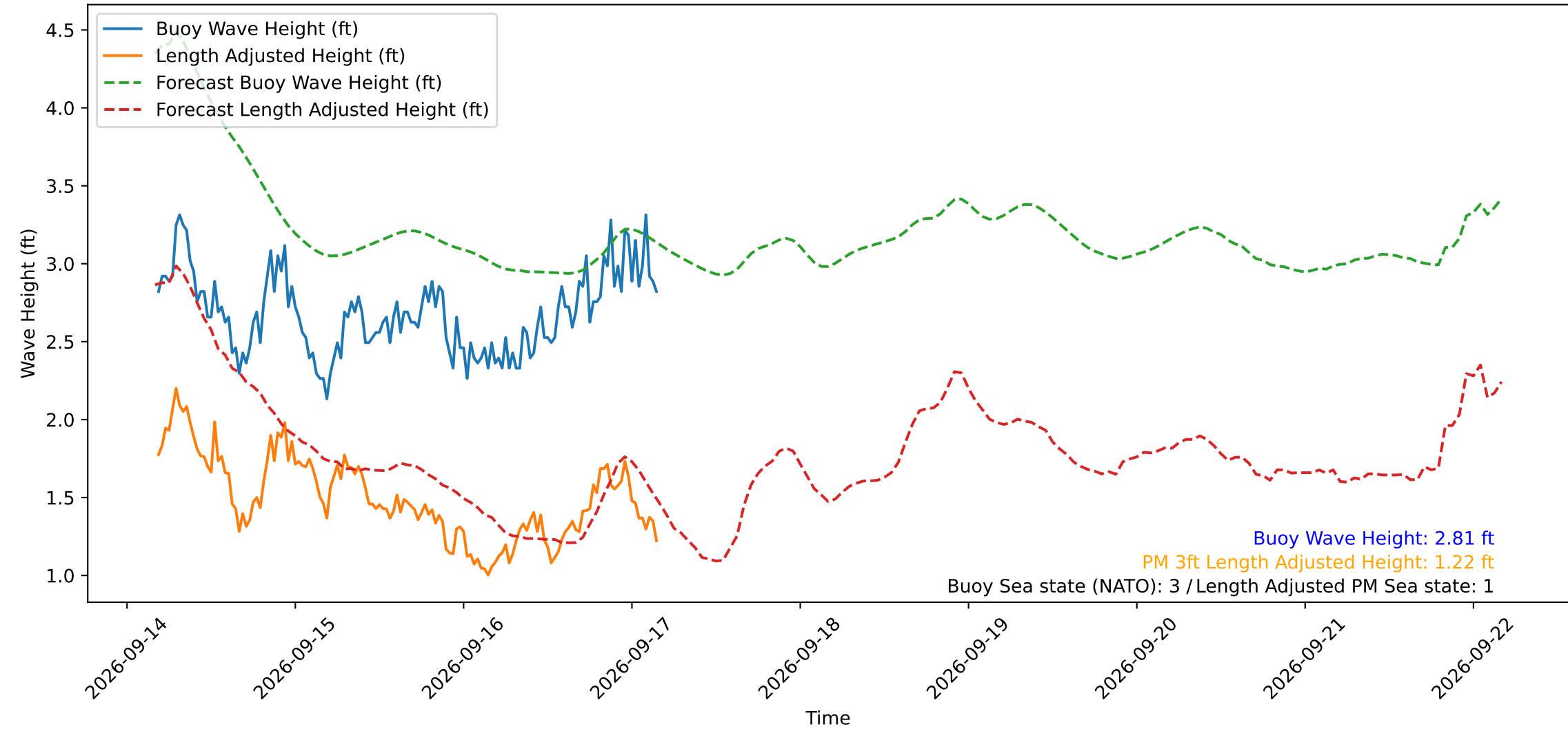
Wave Heights over Time for Green Beach at 2026-09-17 04:11:11
