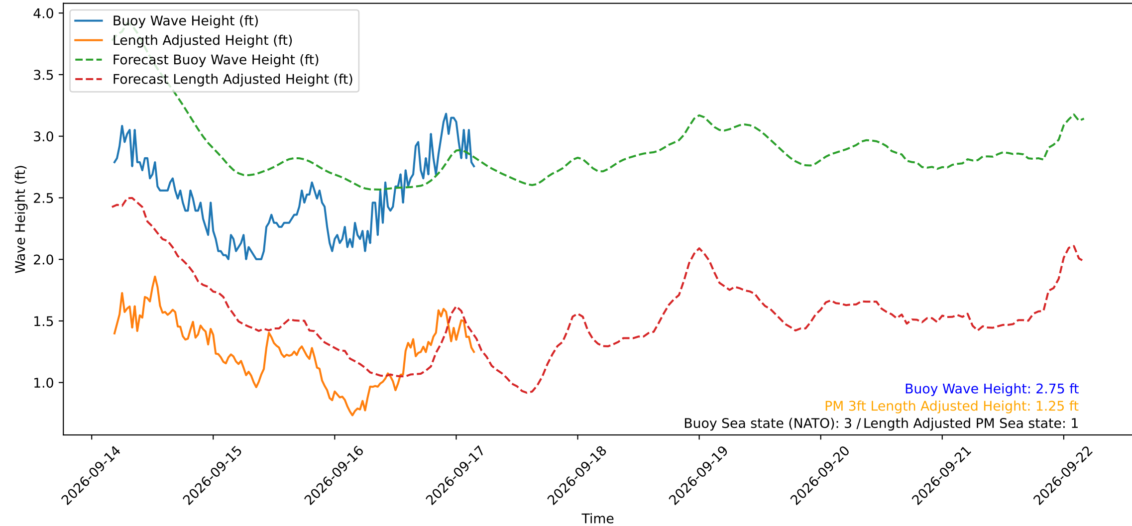
Wave Heights over Time for Red Beach at 2026-09-17 04:10:49
