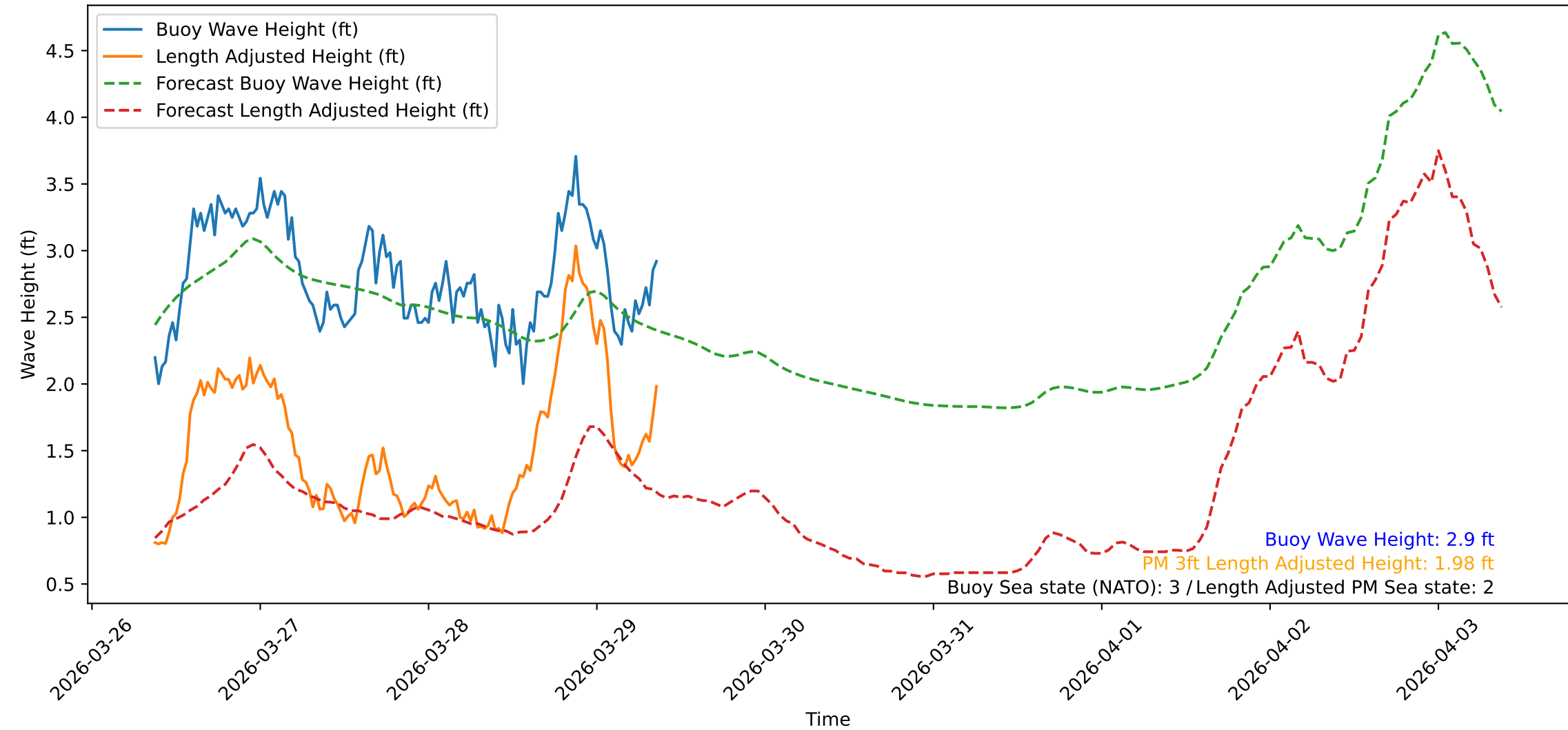
Wave Heights over Time for Green Beach at 2026-03-29 09:11:11
