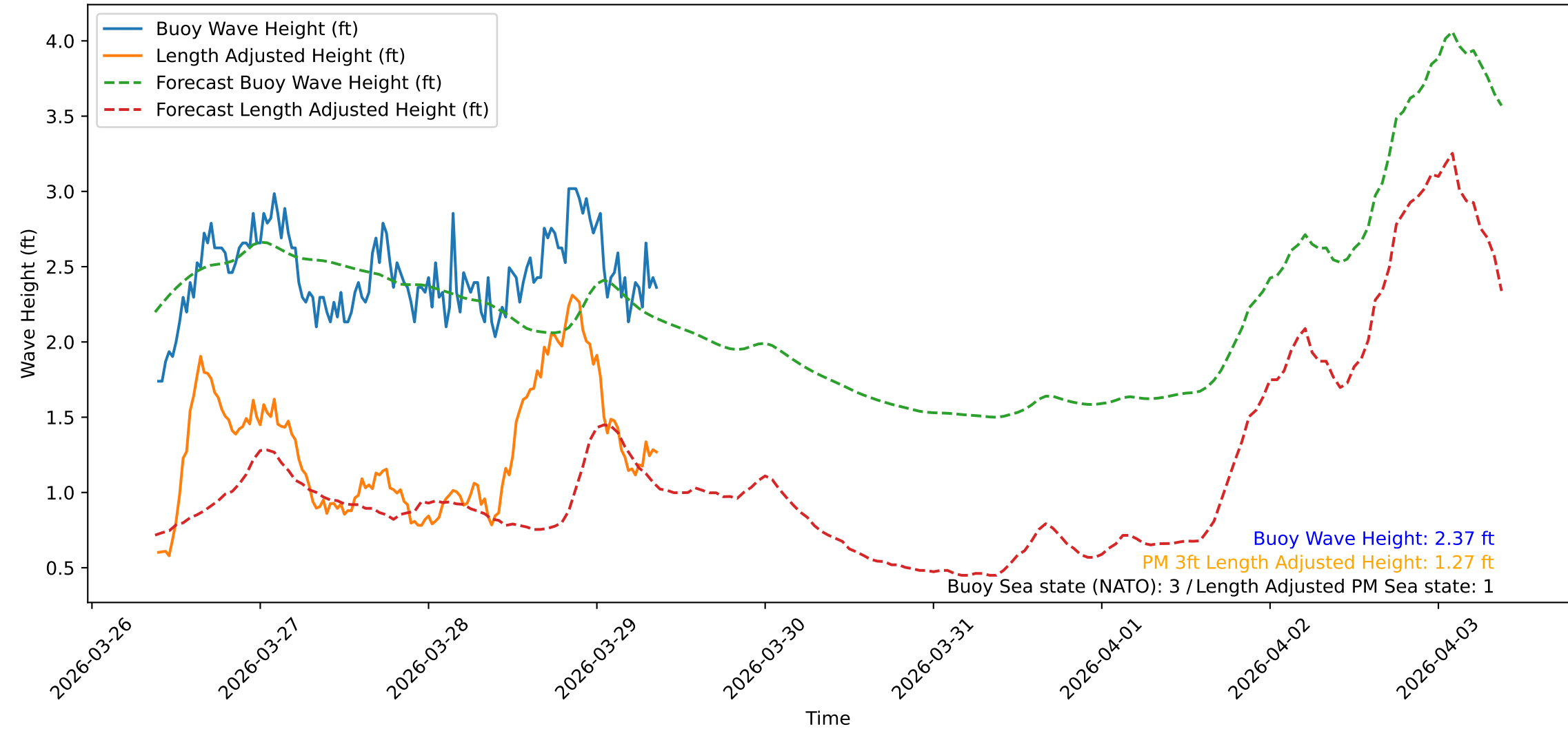
Wave Heights over Time for Red Beach at 2026-03-29 09:10:48
