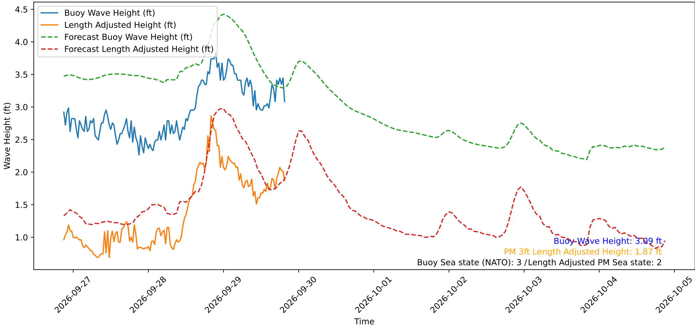
Wave Heights over Time for Red Beach at 2026-09-29 20:30:50
