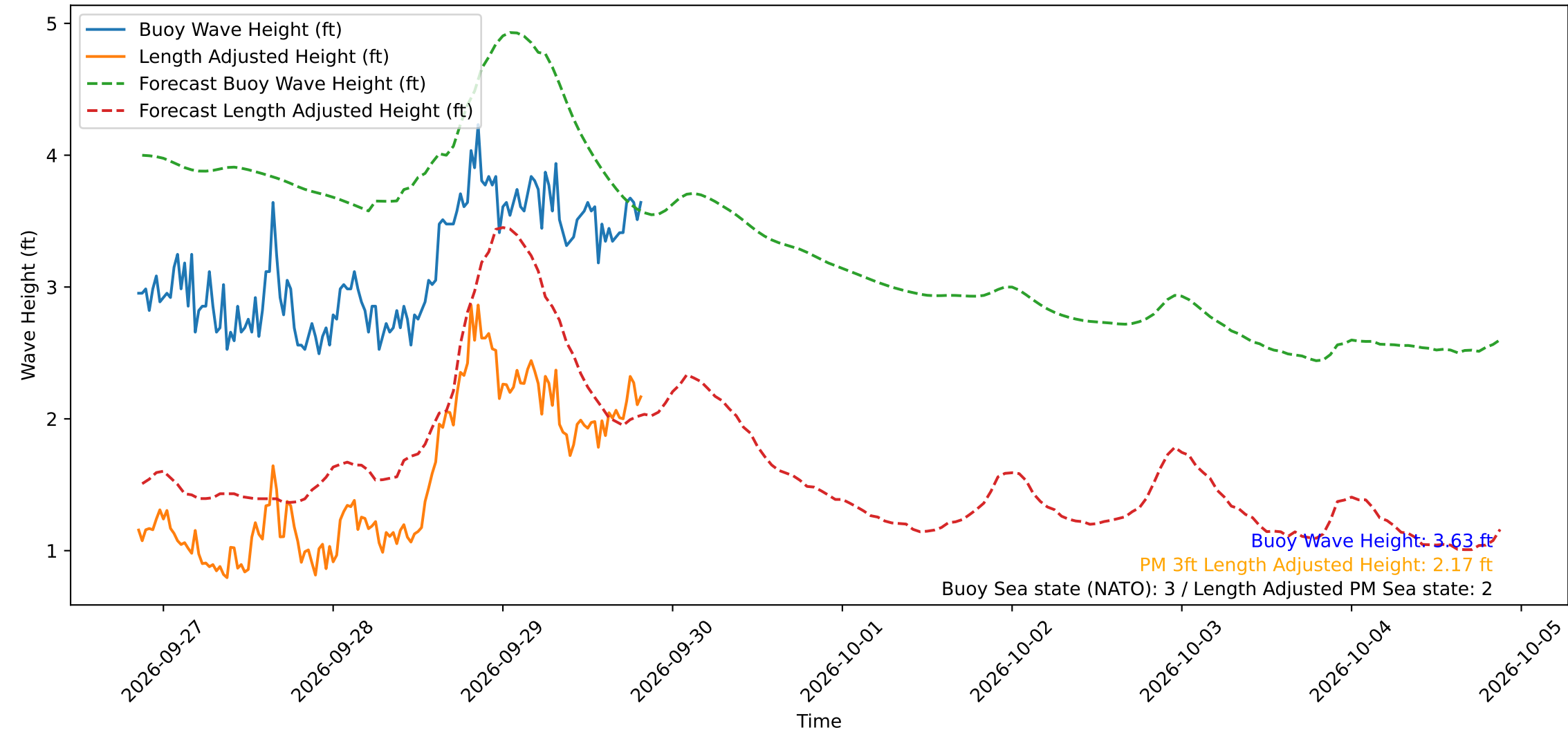
Wave Heights over Time for Oceanside Harbor at 2026-09-29 20:30:30
