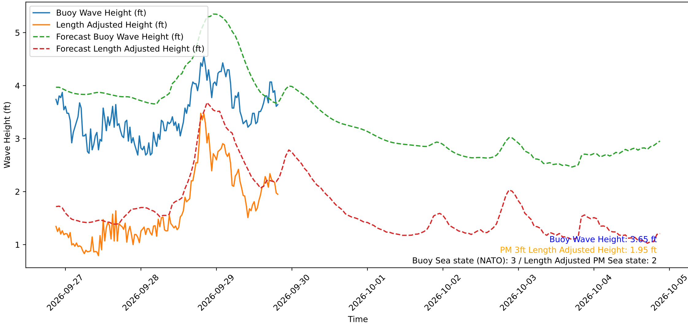
Wave Heights over Time for Green Beach at 2026-09-29 20:31:13
