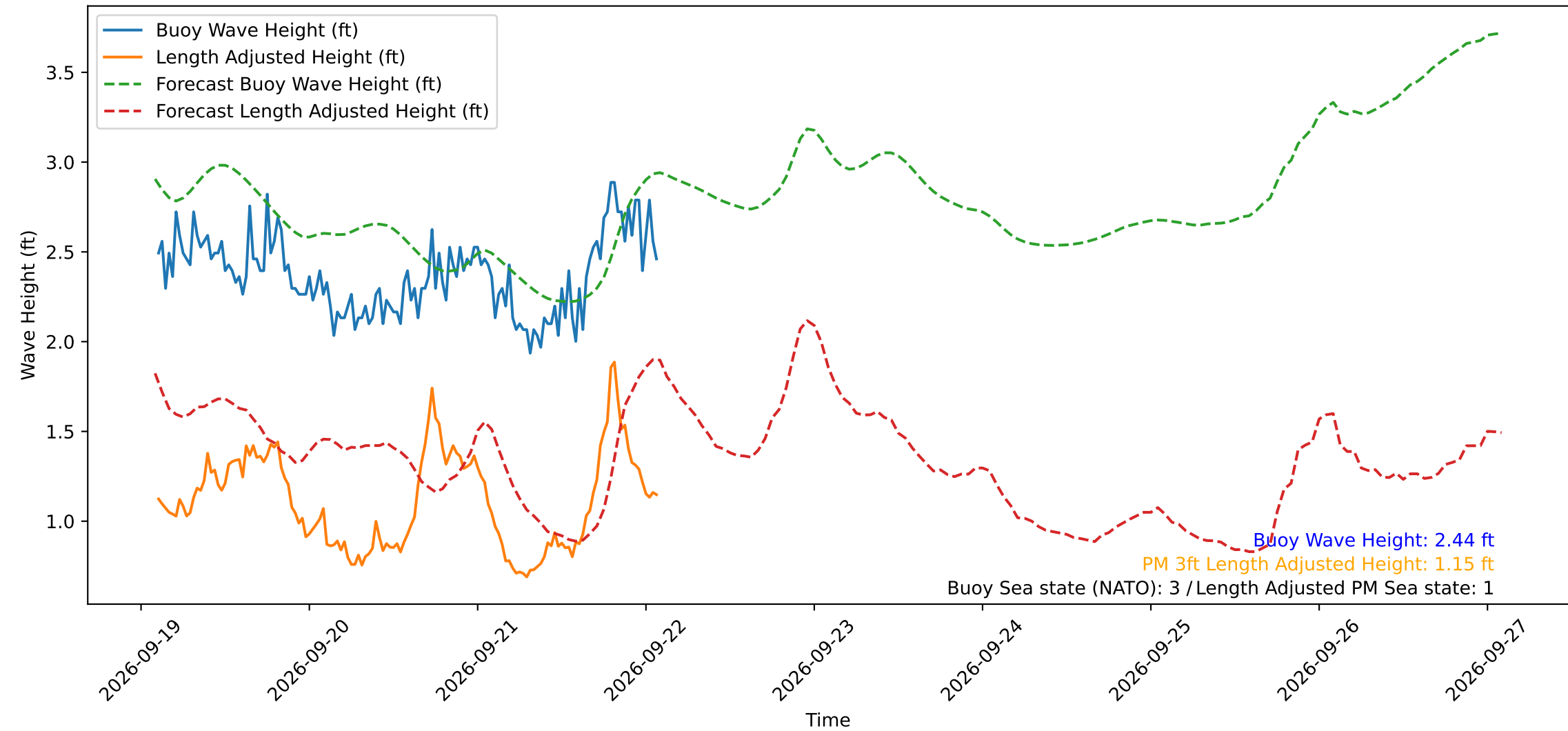
Wave Heights over Time for Red Beach at 2026-09-22 02:20:51
