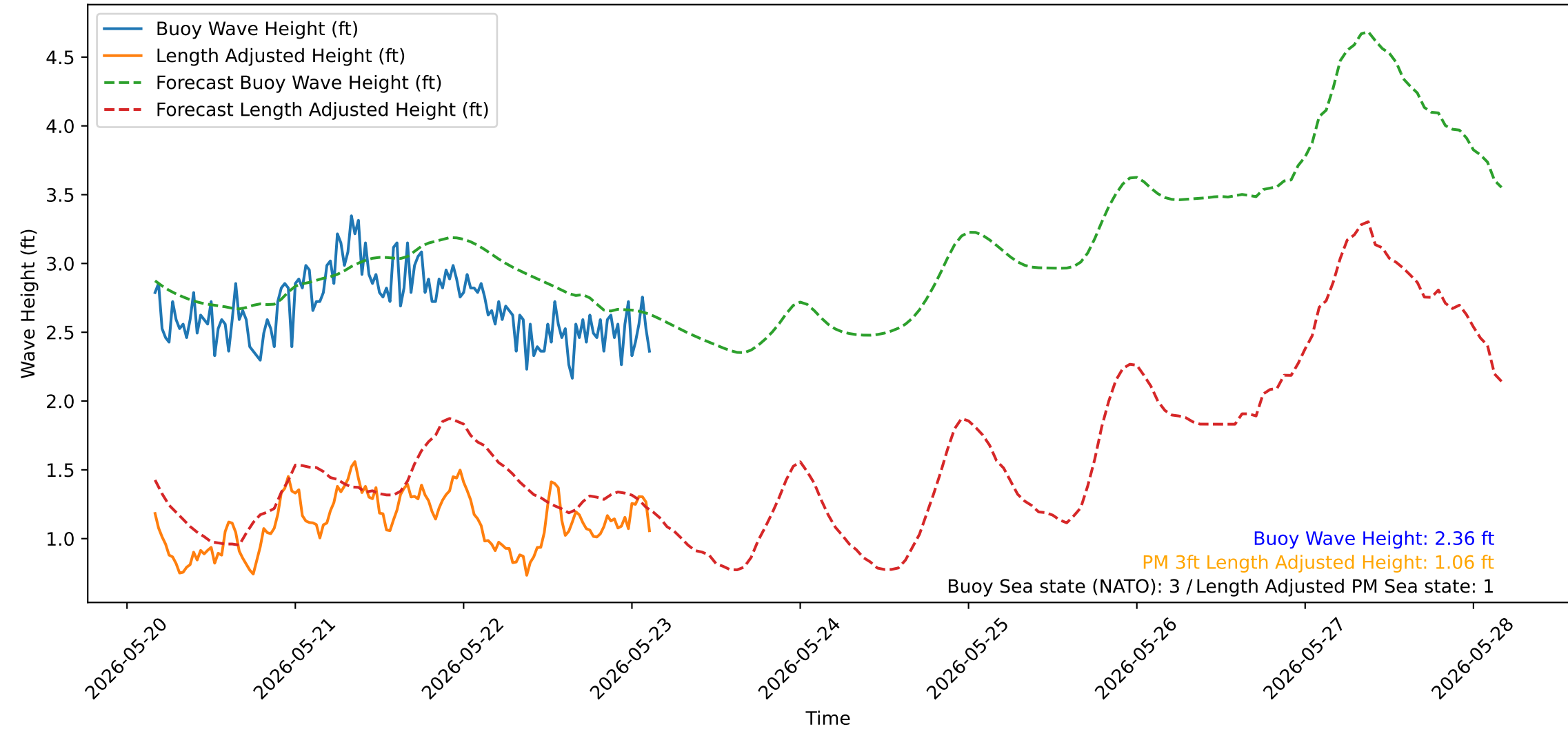
Wave Heights over Time for Red Beach at 2026-05-23 03:30:51
