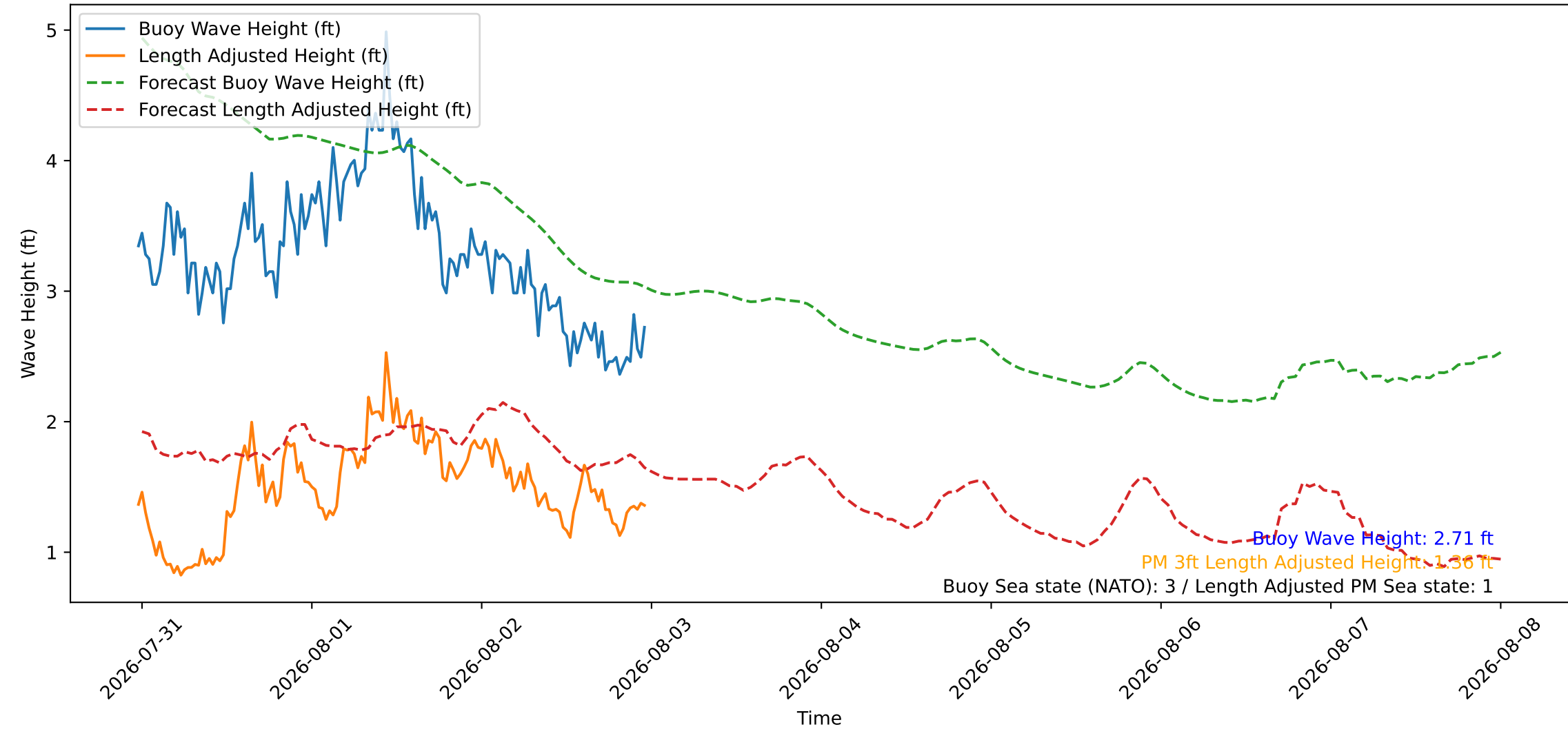
Wave Heights over Time for Green Beach at 2026-08-02 23:41:09
