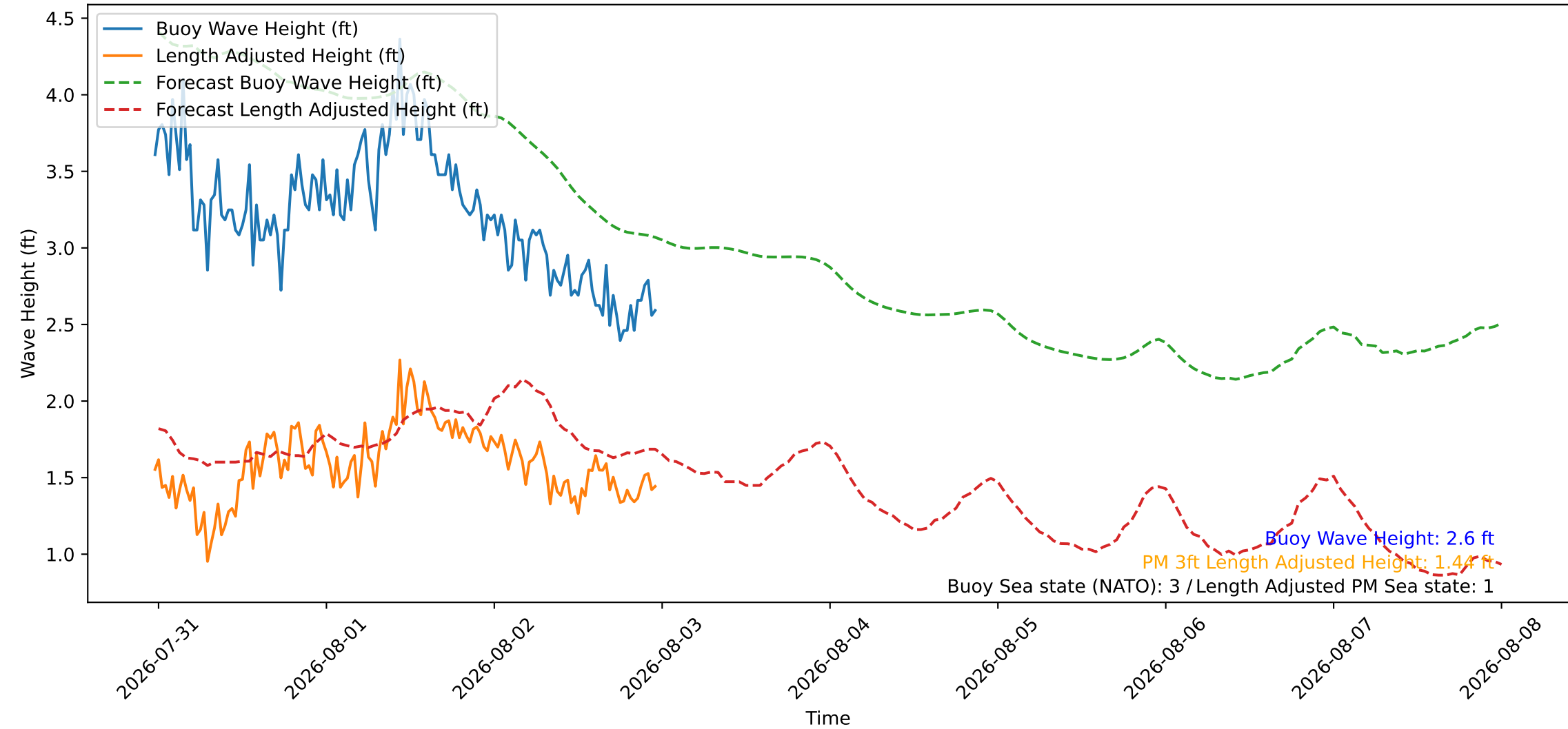
Wave Heights over Time for Oceanside Harbor at 2026-08-02 23:40:26
