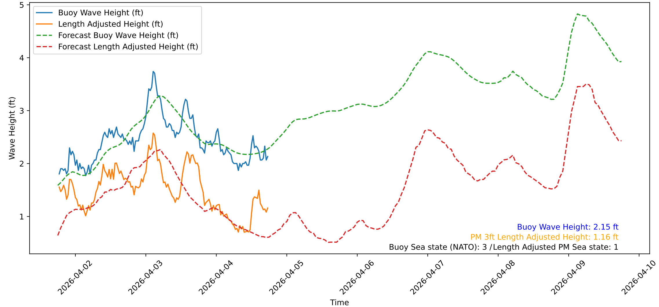
Wave Heights over Time for Red Beach at 2026-04-04 18:20:48
