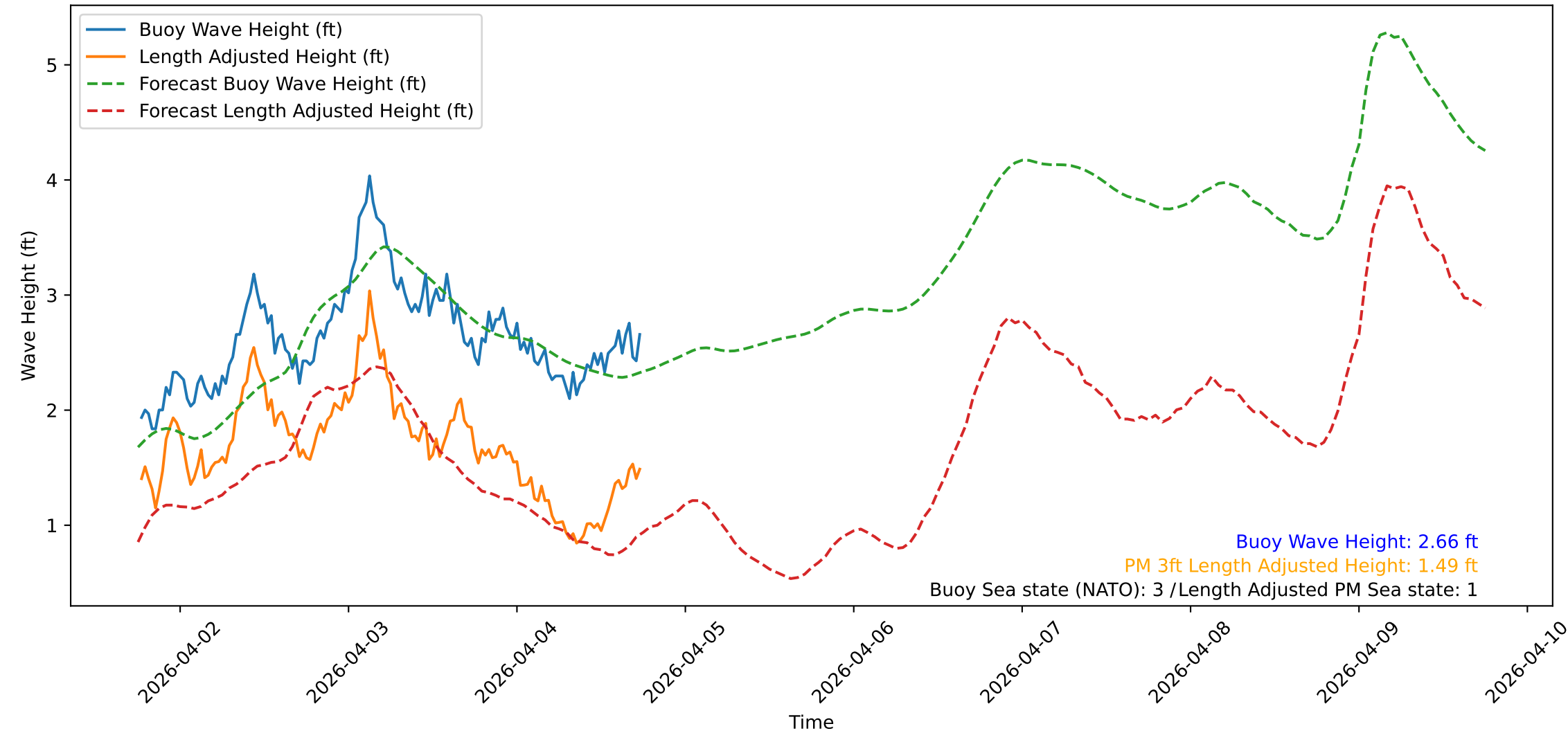
Wave Heights over Time for Oceanside Harbor at 2026-04-04 18:20:32
