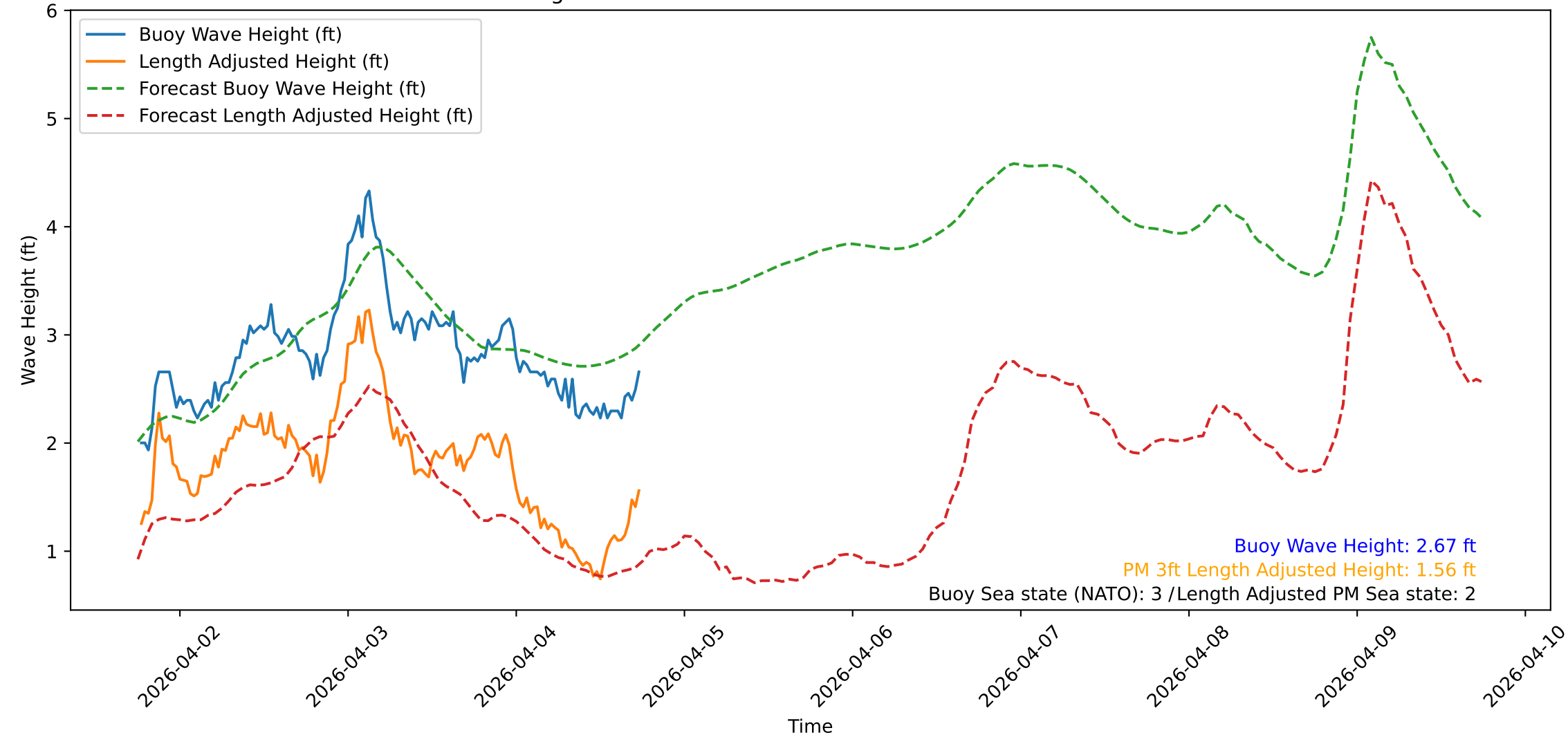
Wave Heights over Time for Green Beach at 2026-04-04 18:21:13
