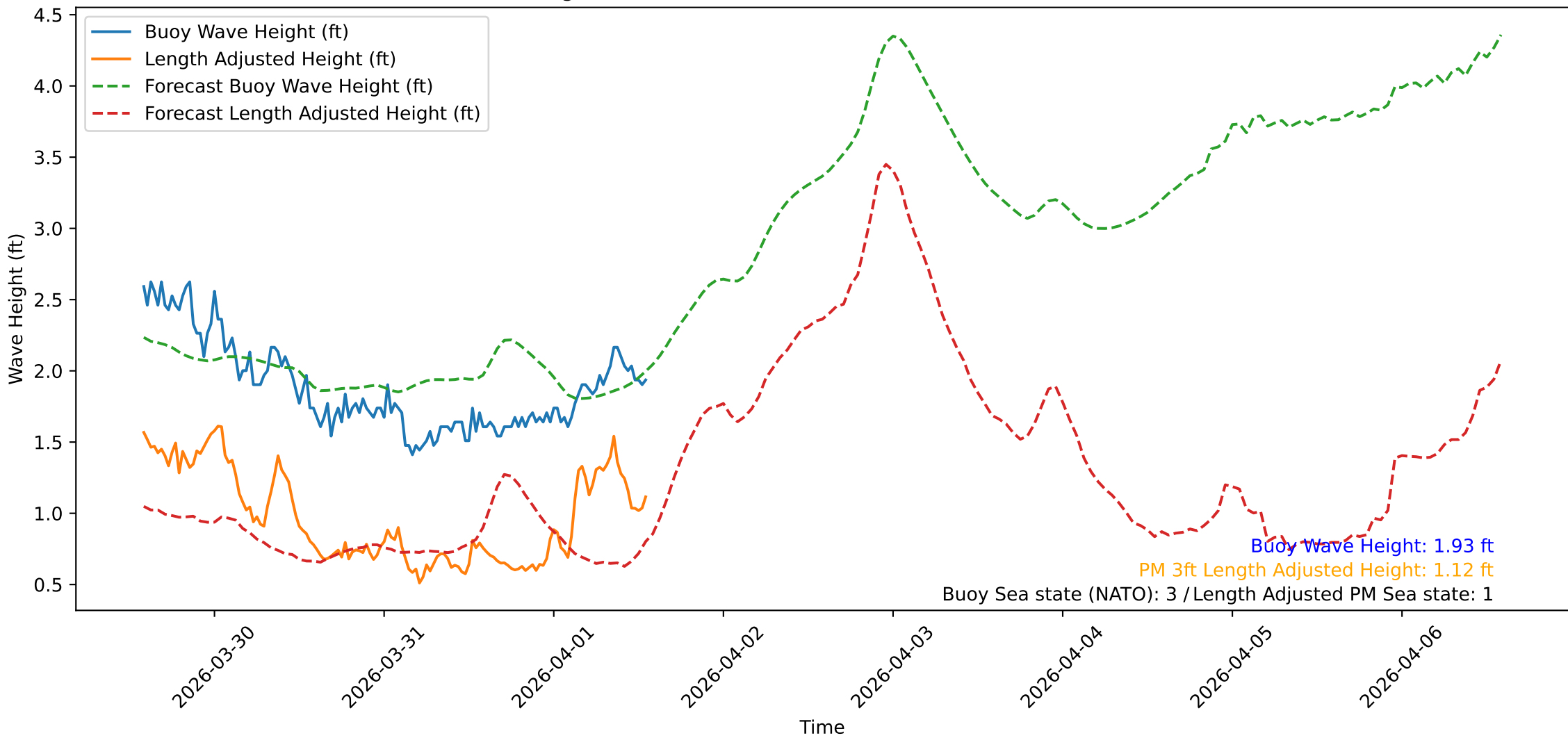
Wave Heights over Time for Green Beach at 2026-04-01 13:51:09
