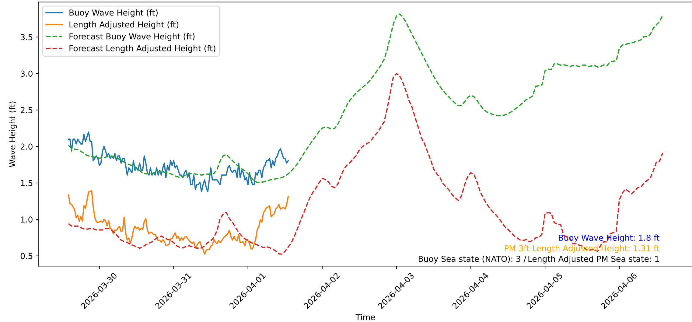
Wave Heights over Time for Red Beach at 2026-04-01 13:50:47
